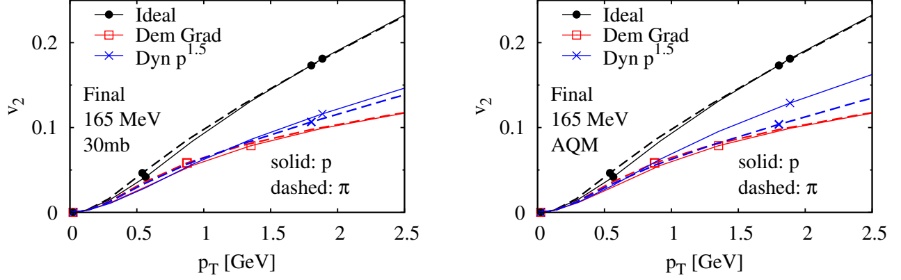
FIG. 7: Differential elliptic flow v_2(p_T) for pions and protons in Au + Au at \sqrt{s_{NN}} = 200 GeV at RHIC with impact parameter b = 7 fm, using 2+1D boost invariant hydrodynamic solutions from AZHYDRO[21, 22], followed by Cooper-Frye fluid-to-particle conversion at T_{conv} = 165 MeV with either the standard “democratic” approach (open boxes) or self-consistent shear corrections (crosses) with momentum dependence \delta f \propto p^{3/2} computed from kinetic theory for a gas of hadrons up to m = 1.672 GeV. In both plots, dashed lines are for pions, while solid curves are for protons, and feeddown from resonance decays is included. Left plot: scenario with constant 30-mb hadronic cross sections. Right plot: cross sections based on the additive quark model (AQM). Results with uncorrected, local equilibrium phase space distributions ( \delta f = 0 ) are also shown (filled circles).
