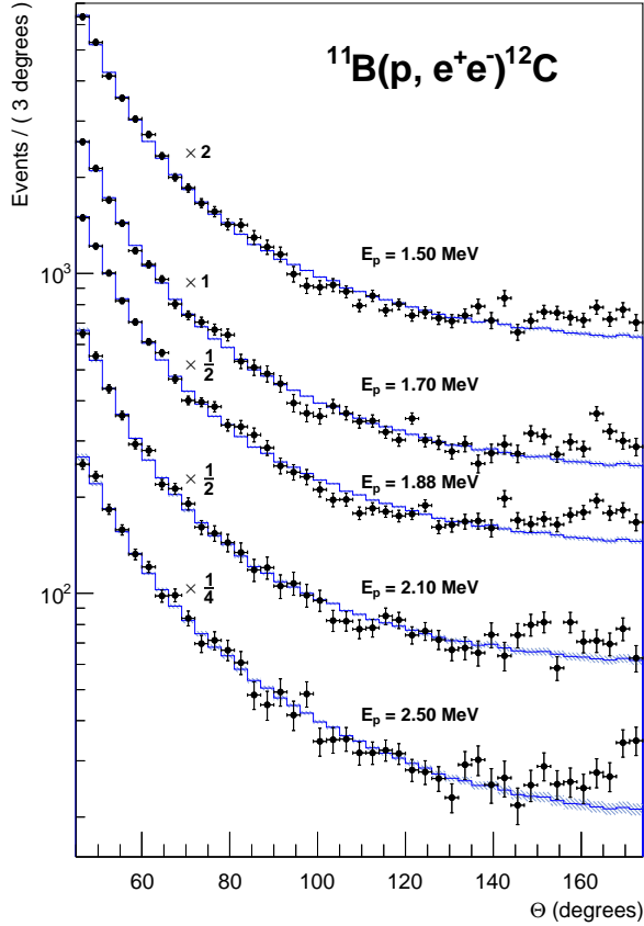
FIG. 3. a) Experimental angular correlations of the e^+e^- pairs measured in the ^{11}\text{B}(p, e^+e^-)^{12}\text{C} reaction at the vicinity of the J^\pi = 1^+ resonance for different proton energies.
