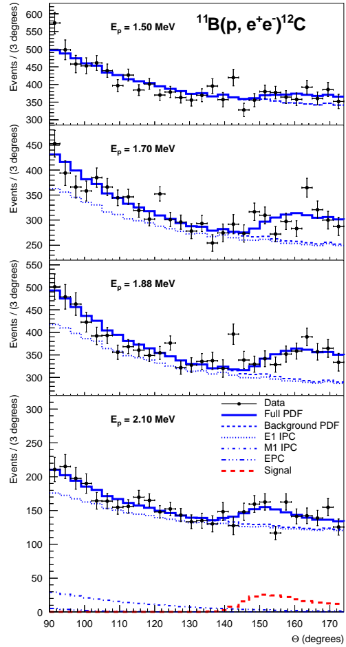
FIG. 4. Experimental angular correlations of the e^+e^- pairs measured at different proton energies. The full curves for each proton energy shows the results of the fit, using simulated angular distributions.
