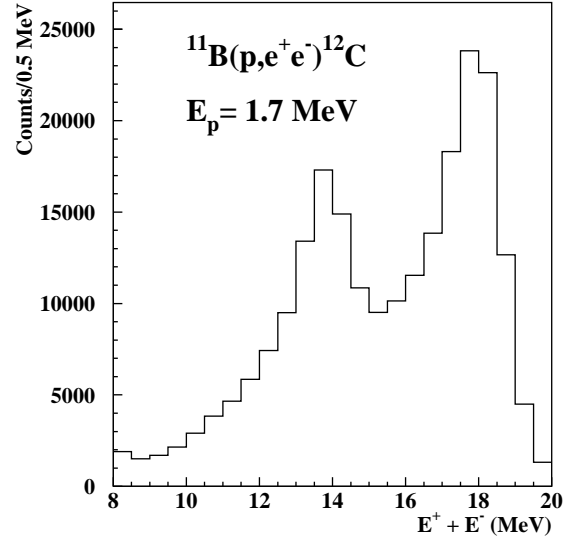
FIG. 2. Total energy spectrum of the e^+e^- -pairs from the ^{11}\text{B}(p, e^+e^-)^{12}\text{C} nuclear reaction.
