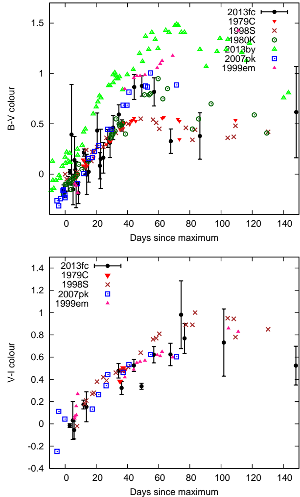
Figure 8. The B-V (upper panel) and V-I (lower panel, if I -band data was available) colour evolution of SN 2013fc, compared to similar SNe 1979C and 1998S and to other type II SNe with a plateau phase and a subsequent drop. All colours are corrected for extinction.
