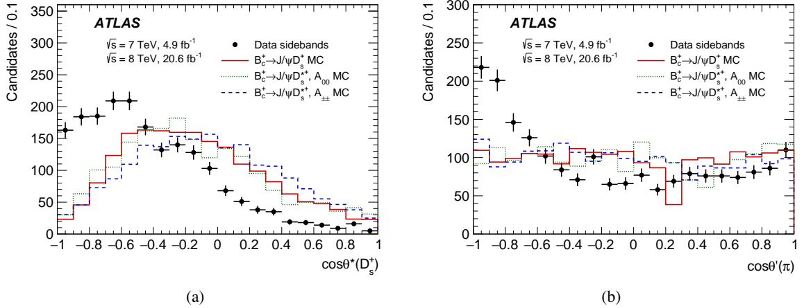
Figure 2: Distributions of (a) \cos \theta^*(D_s^+) and (b) \cos \theta'(\pi) , where \theta^*(D_s^+) and \theta'(\pi) are two angular variables defined in Sect. 3. The distributions are shown for data sidebands (black dots) and MC simulation of B_c^+ \rightarrow J/\psi D_s^+ signal (red solid line) and A_{00} (green dotted line) and A_{\pm\pm} (blue dashed line) components of B_c^+ \rightarrow J/\psi D_s^+ signal. The distributions are obtained after applying all selection criteria except the ones on the plotted variable. The MC distributions are normalised to data.
