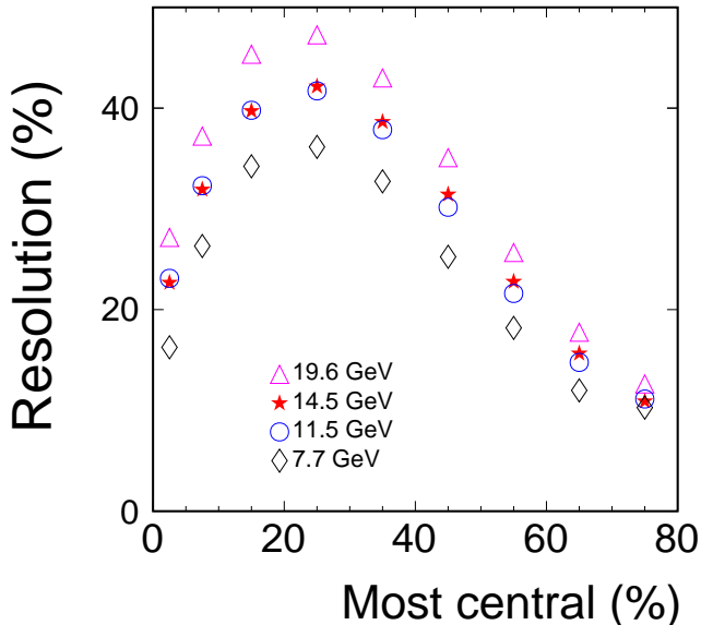
FIG. 2. (Color online) The subevent plane resolution for several beam energies versus centrality with 5% being the most central.
