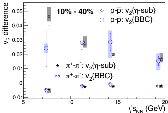
FIG. 7. (Color online) The v_2 difference between protons and antiprotons (and between \pi^+ and \pi^- ) for 10%–40% centrality Au+Au collisions at 7.7, 11.5, 14.5, and 19.6 GeV. The v_2\{\text{BBC}\} results were slightly shifted horizontally.
