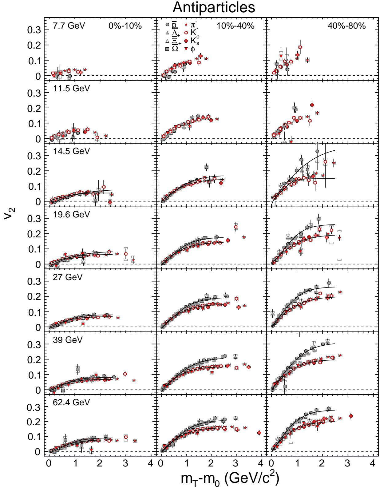
FIG. 4. (Color online) The elliptic flow v_2 of identified antiparticles ( \pi^- , K^- , K_s^0 , \bar{p} , \phi , \bar{\Lambda} , \bar{\Xi}^+ , \bar{\Omega}^+ ) as a function of m_T - m_0 , for 0%–10%, 10%–40%, and 40%–80% central Au + Au collisions at \sqrt{s_{NN}} = 7.7, 11.5, 14.5, 19.6, 27, 39, and 62.4 GeV. The lines show simultaneous fits to baryons and mesons with Eq. (1). The systematic errors are shown by the hooked error bars.
