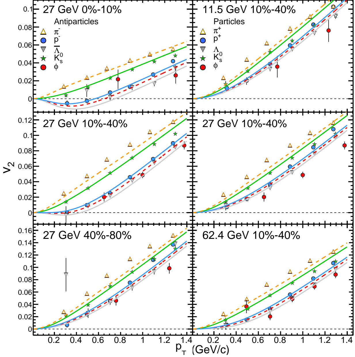
FIG. 11. (Color online) Elliptic flow v_2 as a function of p_T for particles and antiparticles. The data are shown by symbols. On the left side are Blast Wave fits (lines) for three centrality bins for \sqrt{s_{NN}} = 27 GeV. On the right side are Blast Wave fits for three beam energies for 10%–40% centrality. Antiparticles are on the left, particles on the right. The lines are the same color and in the same order as the points. The dashed lines for \pi and \phi are not fits, but predictions based on the other fits. The error bars depict the combined statistical and systematic errors.
