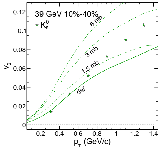
FIG. 8. (Color online) Elliptic flow v_2 as a function of p_T for K_s^0 data at \sqrt{s_{NN}} = 39 GeV for 10%–40% centrality. The curves are for AMPT default and AMPT string melting with cross sections of 1.5, 3.0, and 6.0 mb.
