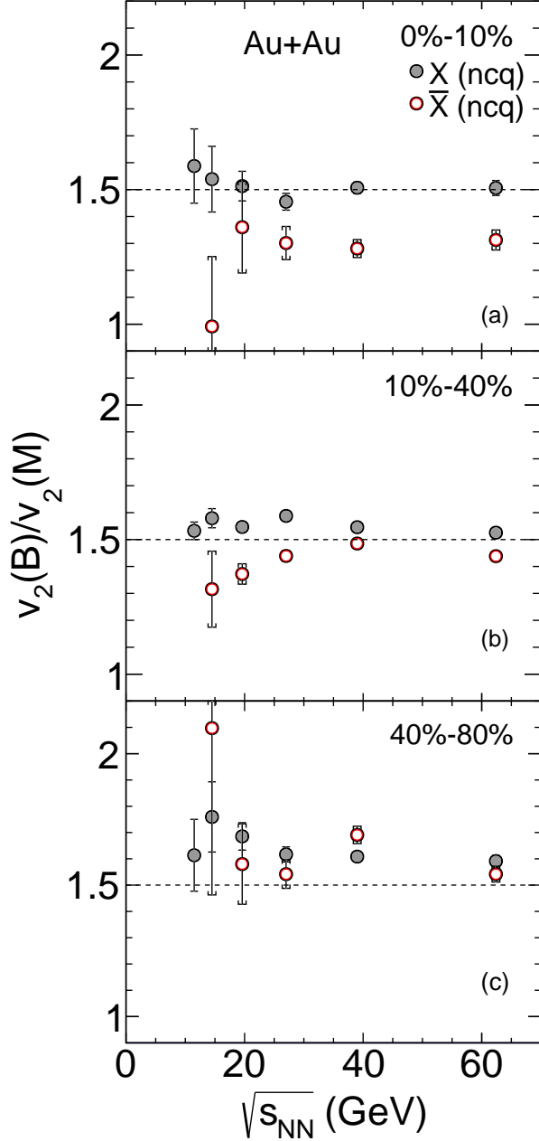
FIG. 5. (Color online) The ratio of v_2 between baryons (B) and mesons (M) of particles (X) and antiparticles ( \bar{X} ) as a function of \sqrt{s_{NN}} for 0%–10%, 10%–40% and 40%–80% central Au + Au collisions. The values of baryons and mesons are taken from the fit lines in Figs. 3 and 4 with Eq. 1 at the appropriate values of m_T - m_0 . See text for details. The open points are for antiparticles and the closed points for particles.
