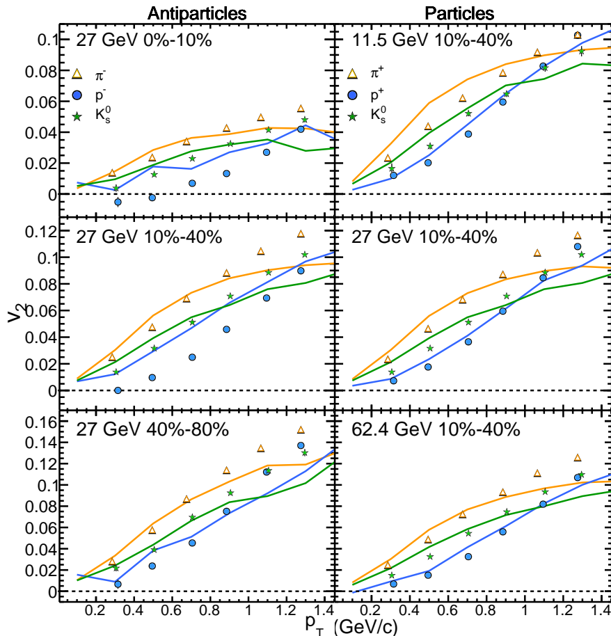
FIG. 9. (Color online) Elliptic flow v_2 as a function of p_T for particles and antiparticles. The symbols show the experimental data. The error bars are mostly smaller than the points. The lines, with the same color code and the same order, show the AMPT string melting calculations with a cross section 1.5 mb. Antiparticles are on the left for three centrality bins. Particles are on the right for three beam energies.
