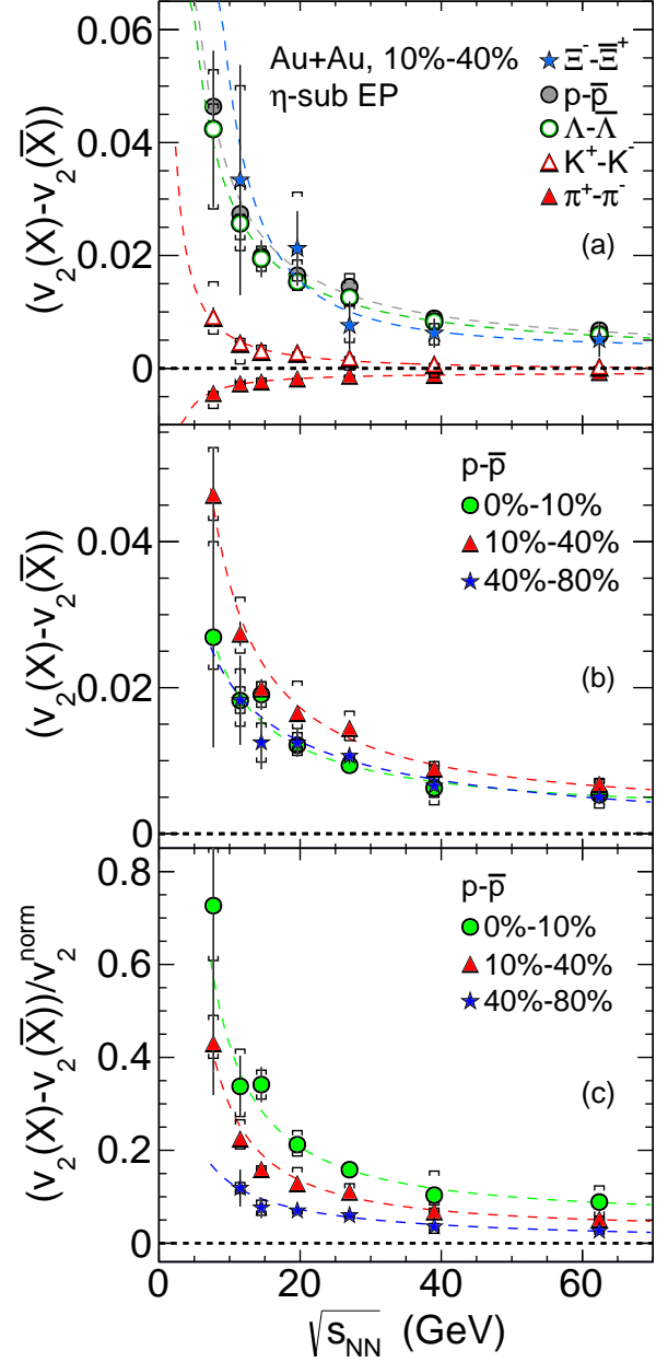
FIG. 6. (Color online) (a) The difference in v_2 between particles (X) and their corresponding antiparticles ( \bar{X} ) (see legend) as a function of \sqrt{s_{NN}} for 10%–40% central Au + Au collisions. (b) The difference in v_2 between protons and antiprotons as a function of \sqrt{s_{NN}} for 0%–10%, 10%–40% and 40%–80% central Au + Au collisions. (c) The relative difference. The systematic errors are shown by the hooked error function. The dashed lines in the plot are fits with a power-law function.
