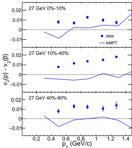
FIG. 10. (Color online) Elliptic flow v_2 as a function of p_T for protons minus antiprotons at \sqrt{s_{NN}} = 27 GeV for three centralities. The curves are for AMPT string melting with cross sections of 1.5 mb. The symbols are data.
