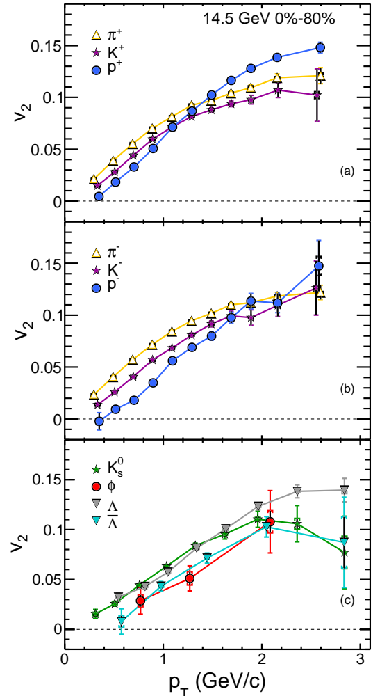
FIG. 1. (Color online) Elliptic flow v_2 as a function of p_T for minimum bias data (0%–80% centrality) at \sqrt{s_{NN}} = 14.5 GeV for identified particles. (a) positively charged particles. (b) negatively charged particles. (c) neutral particles. The systematic errors are shown by the short error bars with caps. The lines connect the points.
