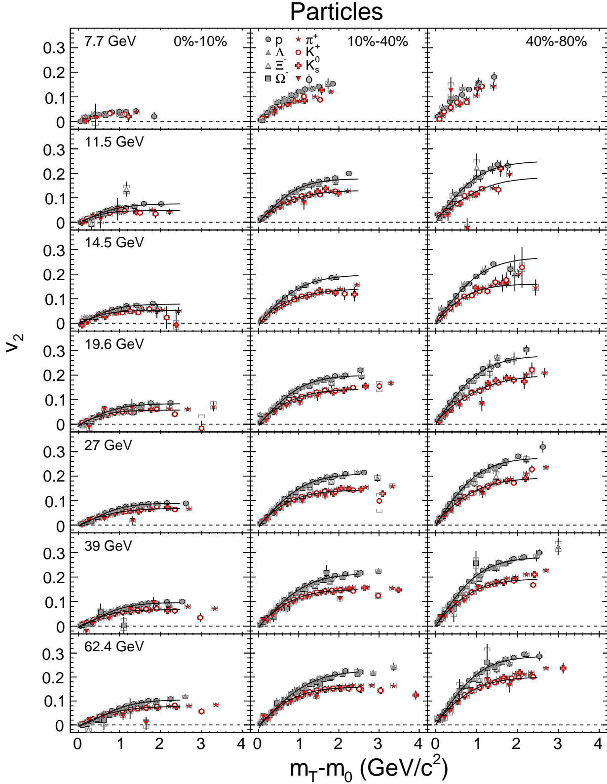
FIG. 3. (Color online) The elliptic flow v_2 of identified particles ( \pi^+ , K^+ , K_s^0 , p , \phi , \Lambda , \Xi^- , \Omega^- ) as a function of m_T - m_0 , for 0%–10%, 10%–40%, and 40%–80% central Au + Au collisions at \sqrt{s_{NN}} = 7.7, 11.5, 14.5, 19.6, 27, 39, and 62.4 GeV. The lines show simultaneous fits to baryons and mesons with Eq. (1). The systematic errors are shown by the hooked error bars.
