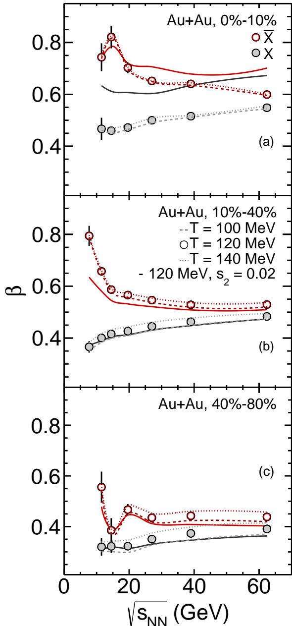
FIG. 12. (Color online) The transverse radial velocity parameter \beta as a function of \sqrt{s_{NN}} for Au + Au collisions for three centralities and three assumed temperatures. The circles are for 120 MeV, open red circles for antiparticles and closed black circles for particles. The error bars seen at low beam energies depict the combined statistical and systematic errors. The solid red and black lines show the result when the s_2 parameter is fixed at 0.02 and the temperature held at 120 MeV.
