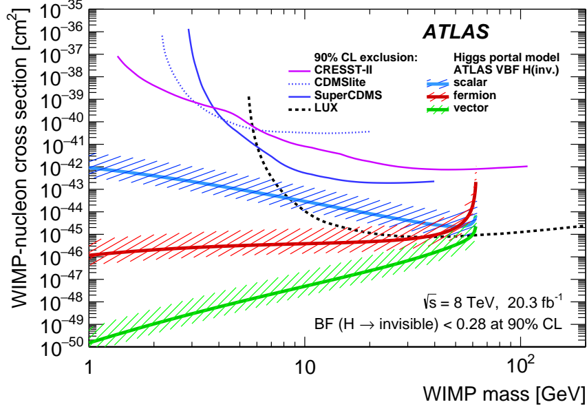
Figure 8: The WIMP–nucleon cross section as a function of the WIMP mass. The exclusion limits [35–39] of the direct detection experiments are compared to the ATLAS results from the \text{BF}(H \rightarrow \text{invisible}) limit in the Higgs-portal scenario, translated into the WIMP–nucleon cross section using the formulas from Ref. [10]. The exclusion limits are shown at 90% CL. The error bands on the ATLAS results indicate the uncertainty coming from the different estimations of the Higgs–nucleon coupling form factor [95, 96].
