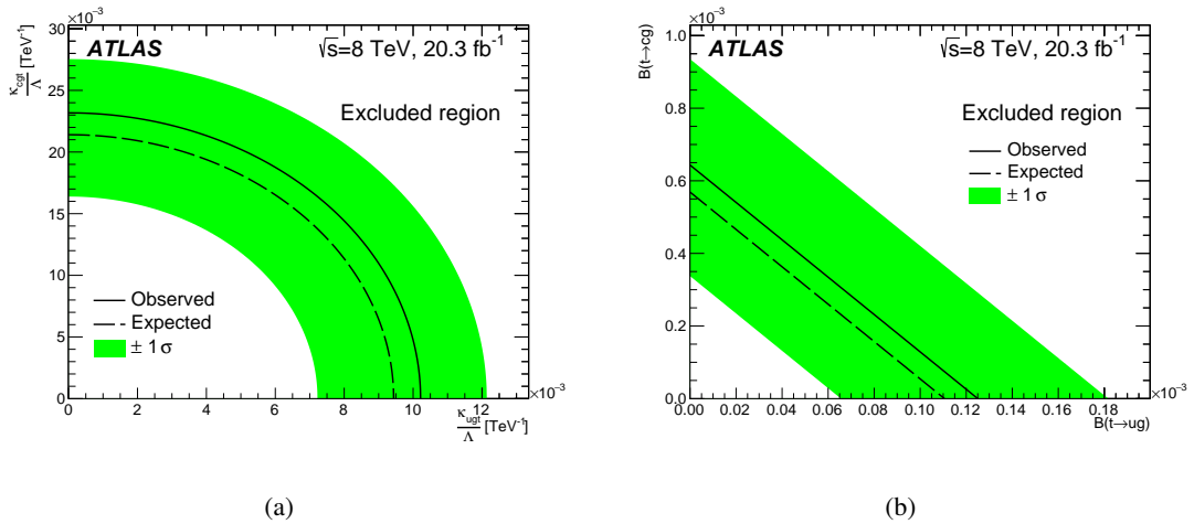
Figure 10: (a) Upper limit on the coupling constants \kappa_{ugt} and \kappa_{cgt} and (b) on the branching fractions \mathcal{B}(t \rightarrow ug) and \mathcal{B}(t \rightarrow cg) . The shaded band shows the one standard deviation variation of the expected limit.
