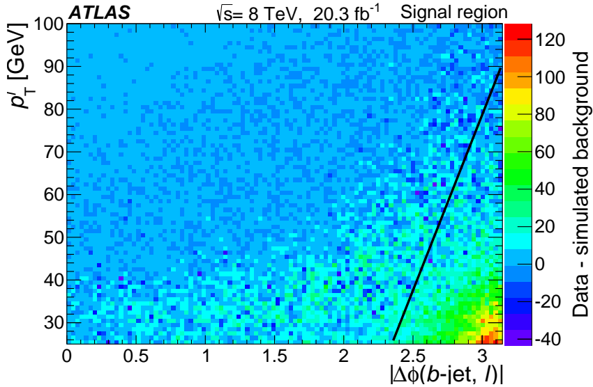
Figure 2: The transverse momentum of the lepton versus the azimuthal angle between the lepton and the jet. The colours indicate the number of events in data after the simulated backgrounds except the multi-jet contribution have been subtracted and before the cut given by Eq. 1 is applied. The solid black line shows the cut.
