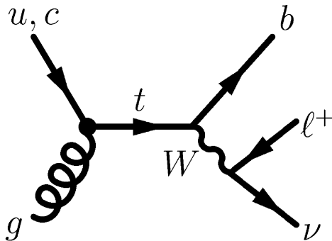
Figure 1: Leading-order Feynman diagram for FCNC top-quark production in the qg \rightarrow t mode followed by the decay of the top quark into a b -quark and a W boson, where the W boson decays into a lepton and a neutrino.
