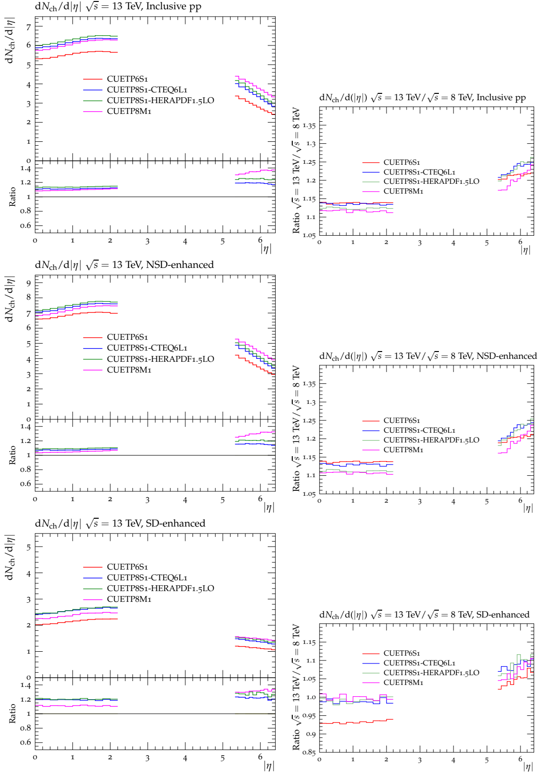
Figure 32: Predictions at \sqrt{s} = 13 TeV for the charged-particle pseudorapidity distribution dN_{\text{ch}}/d|\eta| , for (top) inelastic, (middle) NSD-enhanced, and (bottom) SD-enhanced pp collisions from CUETP6S1-CTEQ6L1, CUETP8S1-CTEQ6L1, CUETP8S1-HERAPDF1.5LO, and CUETP8M1. Also shown are the ratios of the tunes to predictions of CUETP8M1, and the ratio of 13 TeV to 8 TeV results for each of the tunes (right).
