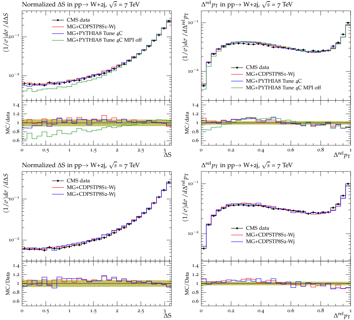
Figure 6: CMS data at \sqrt{s} = 7 TeV [36] for the normalized distributions of the correlation observables \Delta S (left), and \Delta^{\text{rel}}p_T (right) in the W +dijet channel, compared to MADGRAPH (MG) interfaced to: PYTHIA8 Tune 4C, Tune 4C with no MPI, and the CMS PYTHIA8 DPS partial CDPSTP8S1-Wj (top); and CDPSTP8S1-Wj, and CDPSTP8S2-Wj (bottom). The bottom panels of each plot show the ratios of these tunes to the data, and the green bands around unity represent the total experimental uncertainty.
