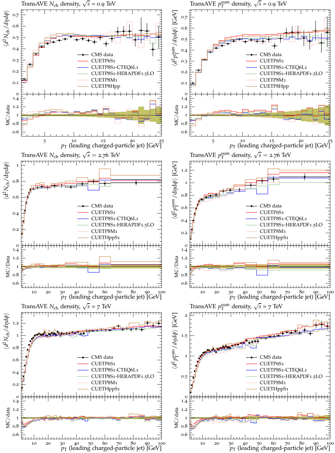
Figure 10: CMS data on charged-particle (left) and p_{\text{T}}^{\text{sum}} (right) densities at \sqrt{s} = 0.9 [24] (top), 2.76 [42] (middle), and 7 TeV [24] (bottom) with p_{\text{T}} > 0.5 GeV and |\eta| < 2.0 in the transverse (TransAVE) region as defined by the leading charged-particle jet, as a function of the transverse momentum of the leading charged-particle jet. The data are compared to predictions of PYTHIA6 using CUETP6S1-CTEQ6L1, PYTHIA8 using CUETP8S1-CTEQ6L1, CUETP8S1-HERAPDF1.5LO, and CUETP8M1, and HERWIG++ using CUETHppS1. The bottom panels of each plot show the ratios of these predictions to the data, and the green bands around unity represent the total experimental uncertainty.
