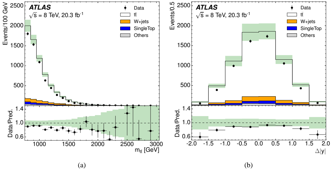
Figure 1: Detector-level distributions of (a) the invariant mass of the t\bar{t} system and (b) the difference of the absolute rapidities \Delta|y| of top and anti-top-quark candidates, for the combination of the e +jets and \mu +jets channels. The observed distributions are compared to the SM expectation based on a mixture of data-driven techniques and Monte Carlo simulation. The ratio of data to the SM expectation is shown in the lower plots. Error bars on the data points indicate the statistical uncertainty. The hashed area shows the uncertainty of the SM prediction. This includes the statistical uncertainty, the theory uncertainties in the cross-sections, the effect of detector systematic uncertainties on the expected yield, the luminosity uncertainty, the uncertainty in the normalisations, and the signal modelling uncertainty.
