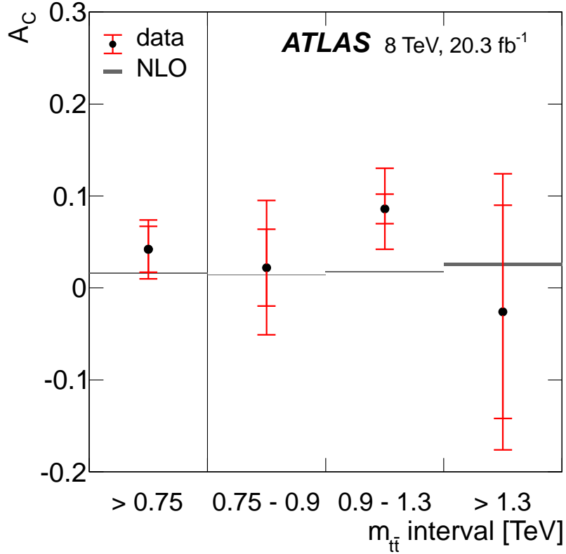
Figure 2: A summary of the charge asymmetry measurements. The error bars on the data indicate the modelling and unfolding systematic uncertainties, shown as the inner bar, and the total uncertainty, which includes the statistical uncertainty and the experimental systematic uncertainties. The SM prediction of the NLO calculation in Ref. [13] for the charge asymmetry of top-quark pairs with |\Delta|y| < 2 is indicated as a shaded horizontal bar in each m_{t\bar{t}} bin, where the width of the bar indicates the uncertainty.
