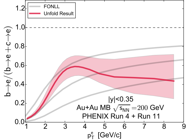
FIG. 17. (Color Online) The fraction of heavy flavor electrons from bottom hadron decays as a function of p_T from this work and from FONLL p+p calculations [31].
