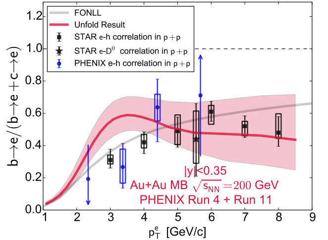
FIG. 18. (Color Online) bottom electron fraction as a function of p_T compared to measurements in p+p collisions at \sqrt{s} = 200 GeV from PHENIX [32] and STAR [33]. Also shown are the central values for FONLL [31] for p+p collisions at \sqrt{s_{NN}} = 200 GeV.
