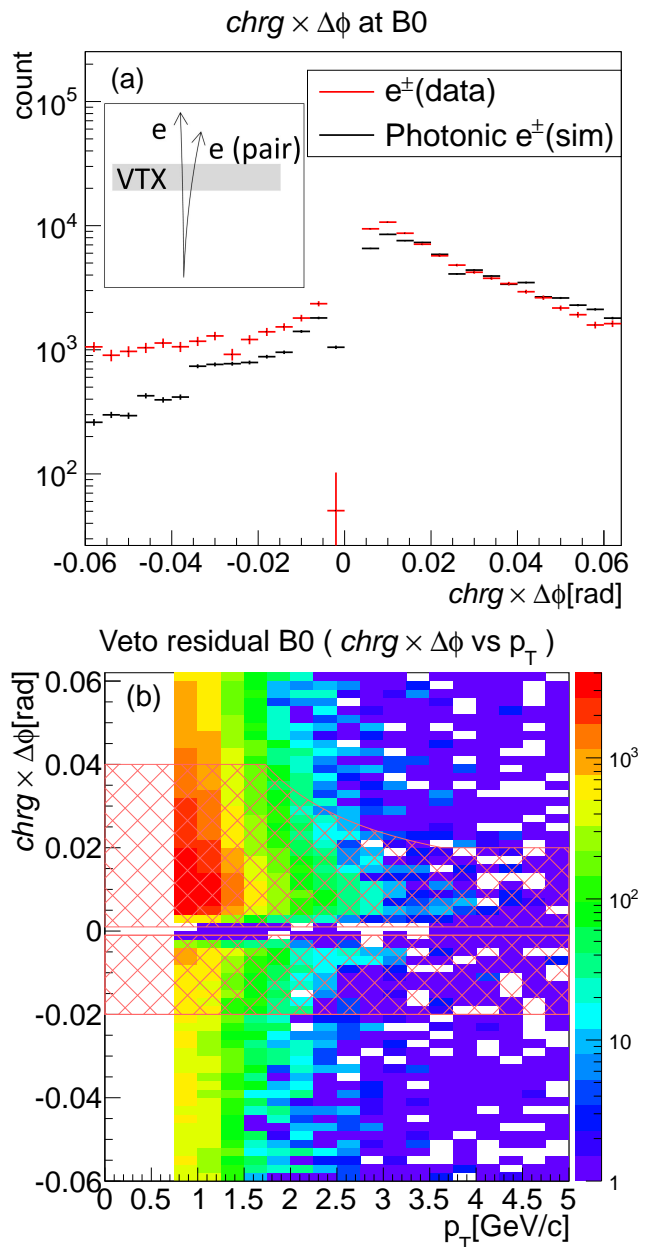
FIG. 7. (a) Distribution of correlated hits in B0 near electron tracks for 1 < p_T < 2 GeV/c. The red points are from Au+Au data and the black points are from Monte Carlo simulation. The insert in (a) illustrates the electron pairs from Dalitz decays. (b) The window of the conversion veto cut for B0 layer (hatched) and the hit distribution near electron track in 2D space of chrg \times \Delta\phi vs p_T of electrons in Au+Au collisions. (See the text for details).
