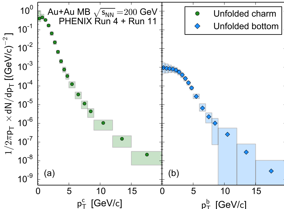
FIG. 15. (Color Online) Unfolded (a) charm ( h_c ) and (b) bottom ( h_b ) hadron invariant yield as a function of p_T , integrated over all rapidities, as constrained by electron yield vs DCA_T in 5 p_T bins and previously published heavy flavor electron invariant yield vs p_T [12].
