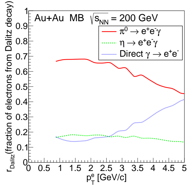
FIG. 21. (Color Online) The fraction of \pi^0 , \eta , and direct photon Dalitz decay electrons in all Dalitz electrons as a function of electron p_T ( p_T^e ).
