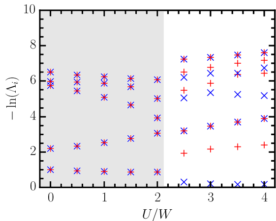
FIG. 4. (color online) The ten largest values of entanglement spectrum extrapolated to the thermodynamic limit as a function of U for \Delta = 2 , J_K = W , J_H = 0.5W . For better visibility of the degeneracies, the subsequent eigenvalues are denoted by + and \times symbols, respectively.
