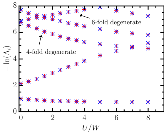
FIG. 1. (color online) The low-lying entanglement spectrum in the isotropic case extrapolated to the thermodynamic limit for J_K = W and J_H = 0.5W . For better visibility of the degeneracies, the subsequent eigenvalues are denoted by + and \times symbols, respectively. In certain cases, where the multiplicity is larger than 2, the degree of degeneracy is given explicitly in the figure.
