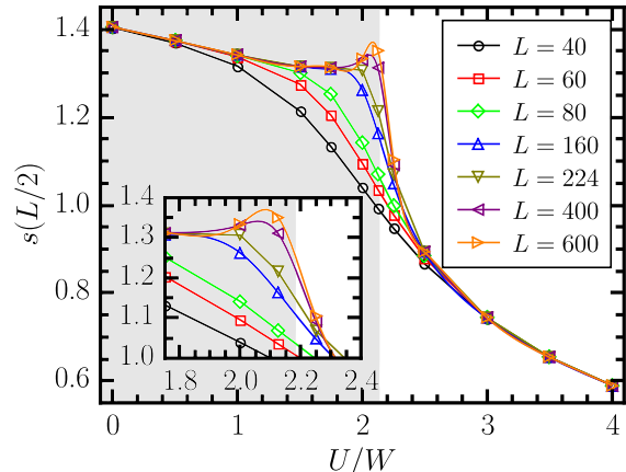
FIG. 3. (color online) The main figure shows the block entropy in the anisotropic case as a function of U for several chain lengths and \Delta = 2 , J_K = W , J_H = 0.5W . The lines are the spline fit to the data points. The inset shows the enlarged region around the critical point.
