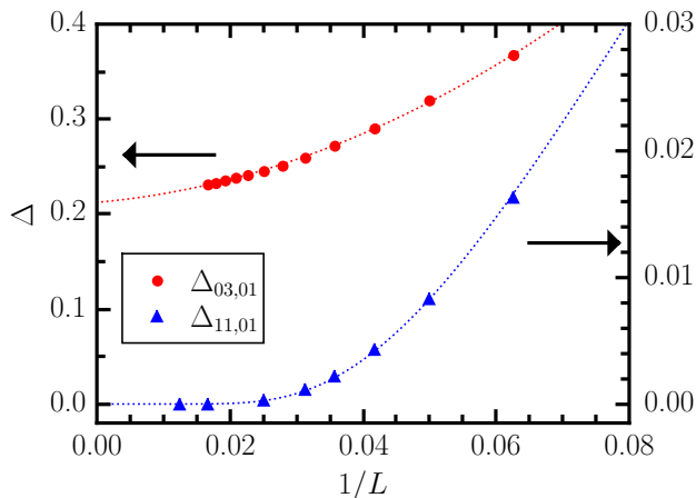
FIG. 5. (color online) Various gap values as a function of inverse chain length for U = 0 and J_K = W , J_H = 0.5W for chains with up to L = 80 lattice sites. The dotted lines denote the best fits to the data using Eqs (11), (12) (see text).
