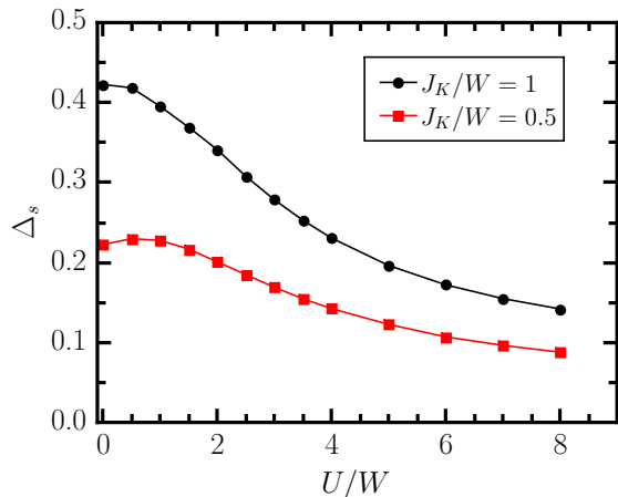
FIG. 2. (color online) The spin gap (extrapolated to the thermodynamic limit) in the isotropic model as a function of U for various J_K and J_H = 0.5W . The lines are guides to the eye.
