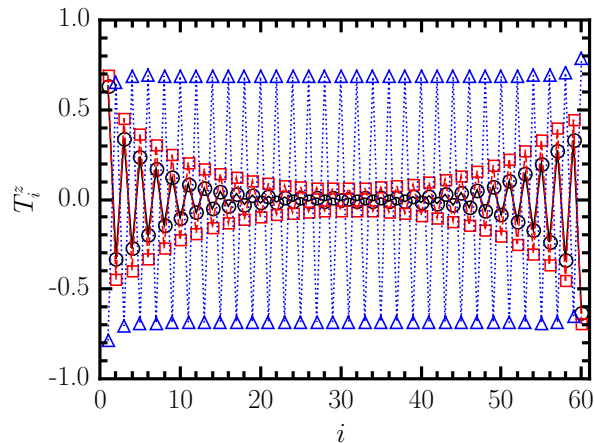
FIG. 7. (color online) The total spin z -component ( T_i^z ) along a finite chain with L = 60 sites and for different values of U . The symbols \circ , \square and \triangle denote U/W = 0, 1 and 3 , respectively. The other parameters are J_K = W , \Delta = 2 , J_H = 0.5W in all cases.
