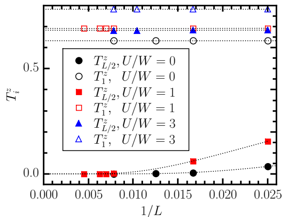
FIG. 8. (color online) Finite-size scaling of T_i^z values at the end of the chain (open symbols) and in the bulk (filled symbols) for different values of U up to L = 224 sites. The other parameters are J_K = W , \Delta = 2 , J_H = 0.5W in all cases.
