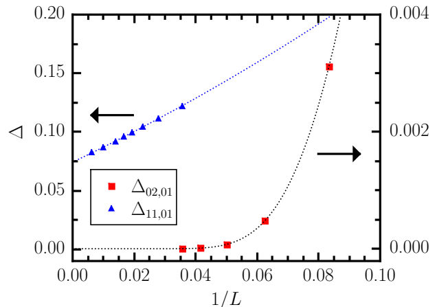
FIG. 6. (color online) Various gap values as a function of inverse chain length for U = 3W and J_K = W , J_H = 0.5W for chains with up to L = 160 lattice sites. The dotted lines denote the best fits to the data using Eqs. (11), (12) (see text).
