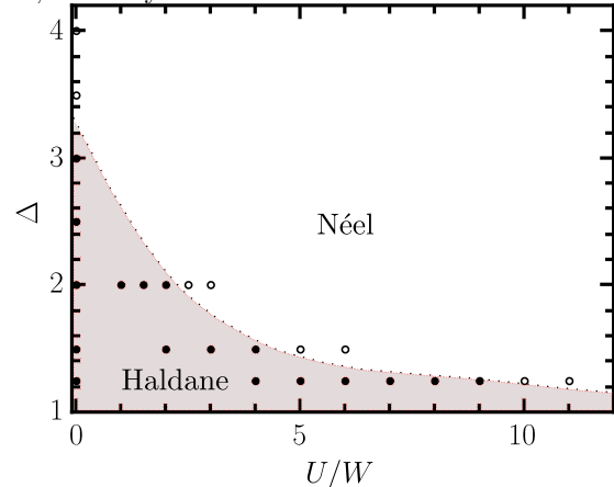
FIG. 9. The phase diagram of the anisotropic model as functions of the anisotropy and the Hubbard interaction strength for J_K = W and J_H = 0.5W . The filled and open circles correspond to Haldane and Néel ground state, respectively. The dotted line denotes the approximate phase boundary.
