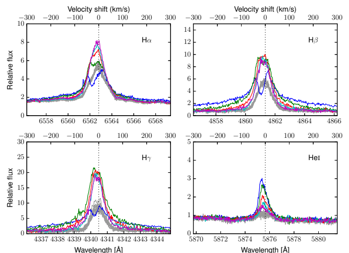
Fig. 12. Individual H\alpha , H\beta , H\gamma , and He\ I spectra from the beginning of the 2453603 flare event. Gray lines show pre-flare spectra, coloured lines show the brightening part of the flare. The spectra were corrected for the radial velocity of V374 Peg with the value of V_r = -3\text{ km s}^{-1} (Montes et al. 2001).
