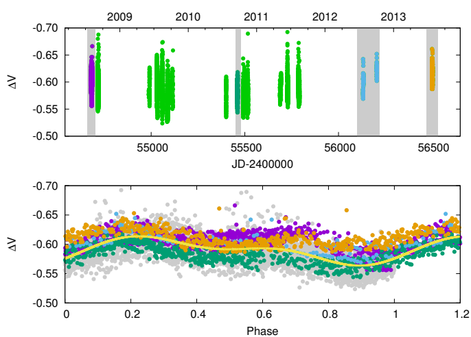
Fig. 2. \Delta V light curve of V374 Peg (top), and the marked parts phased at the bottom. Continuous line shows a model fit with two spots (see Sect. 3.4). Note, that the plot does not show most of the flares.
