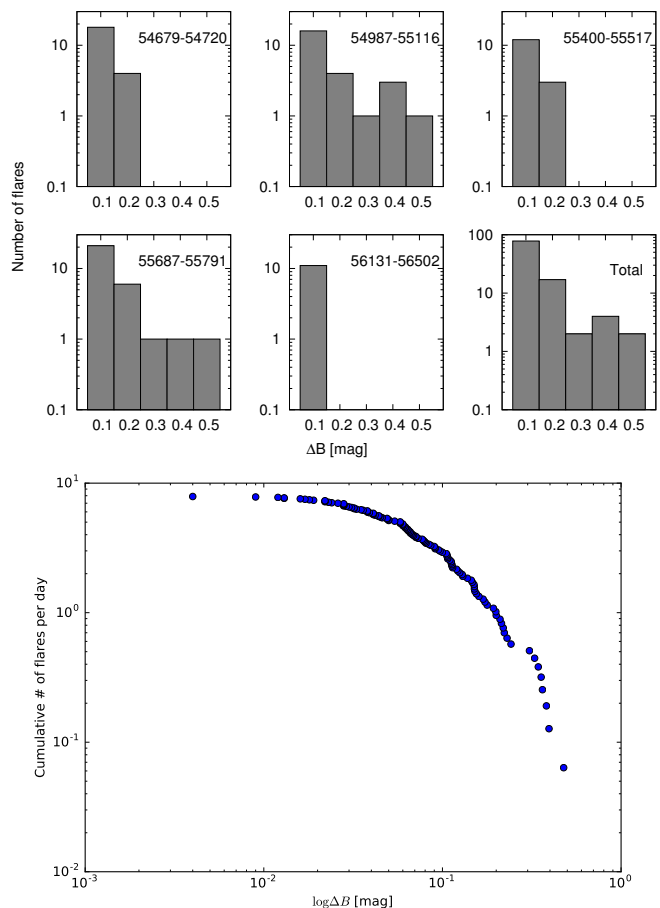
Fig. 6. Top plots: numbers of flares are shown to their peak B brightness. Bottom plot: cumulative number of flares per day vs. flare amplitudes.
