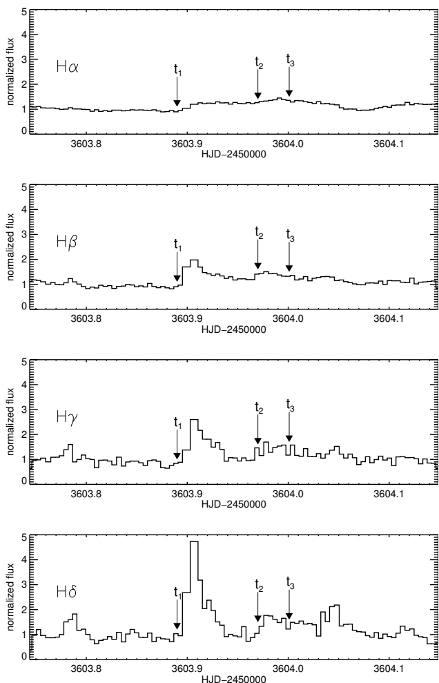
Fig. 14. Light curves for the HJD 2453603 event for H\alpha , H\beta , H\gamma , and H\delta . The flare, which can be seen easily, is pronounced in H\beta , H\gamma , and H\delta , and much weaker in H\alpha . The starting times of the BWE are marked with arrows.
