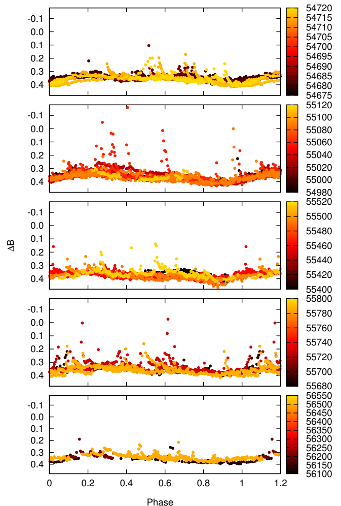
Fig. 15. Phased \Delta B light curves as used for flare statistics. Colours brighten with HJD. Note that the second and fourth plot do not show the strongest flares.
