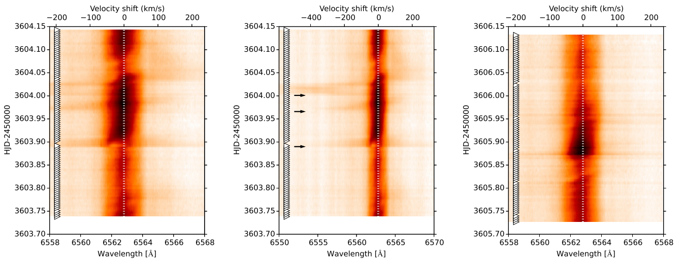
Fig. 9. Dynamic H \alpha spectra of V374 Peg from 2005, showing strong flare events. The first two plots show the same data with different wavelength scales. This way the CME signature – the blue wing enhancement – can be also seen (their start indicated with arrows in the second plot).
