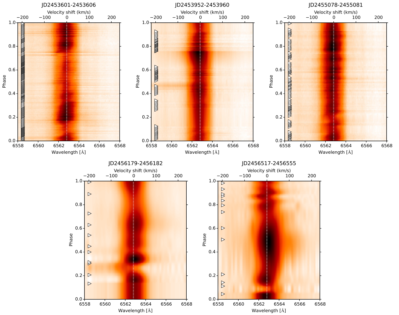
Fig. 8. Phased dynamic H \alpha spectra from 2005, 2006, 2009 (CFHT observations, top row), 2012 and 2013 (RCC observations, bottom row). Triangles mark the rotational phases of the individual spectra, dotted line shows the 0 km s -1 velocity shift.
