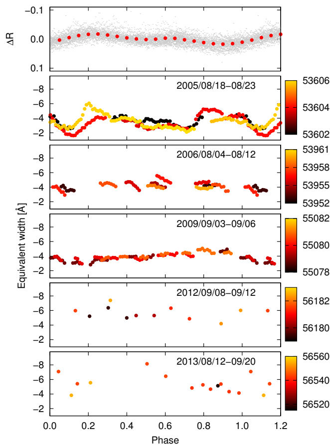
Fig. 11. Top plot shows folded, and averaged \Delta R light curve of V374 Peg including also the observations from 1998 and 2000, after removing long-term trends. The bottom plots show the change of H\alpha equivalent width with rotational phase, colours brightening with time.
