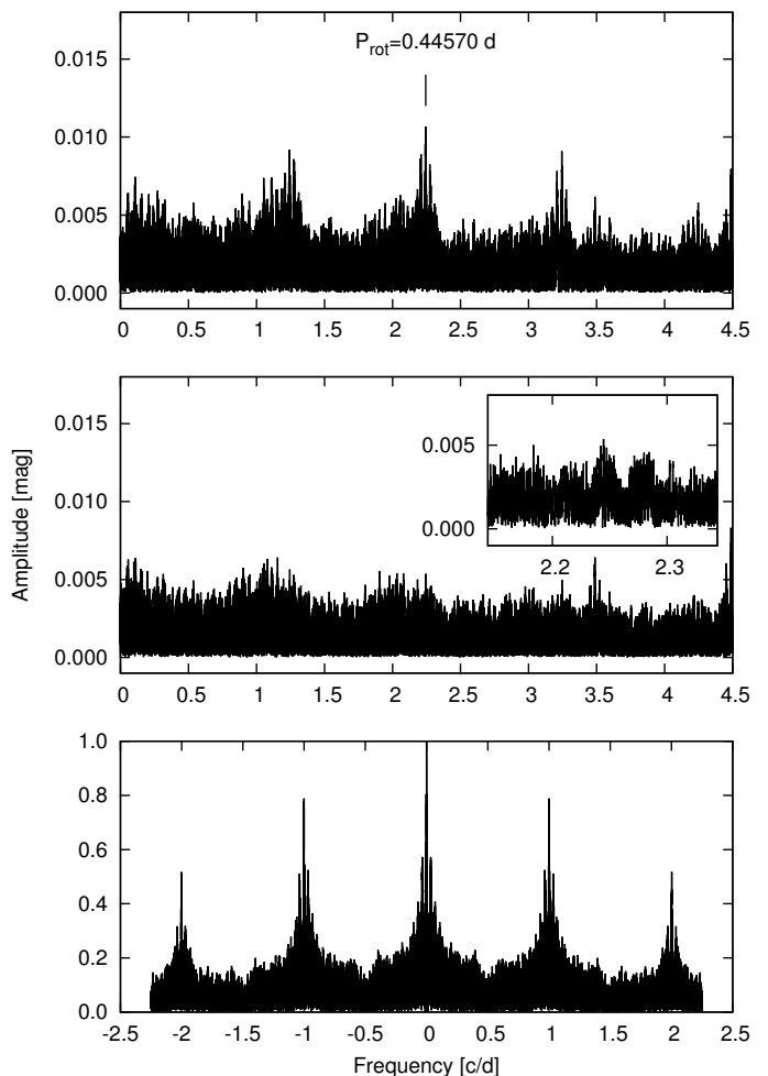
Fig. 4. Fourier spectrum of the \Delta R light curve (top), the spectrum pre-whitened with the rotation frequency (middle), the inset showing a zoom-in to the rotation area, and the spectral window (bottom).
