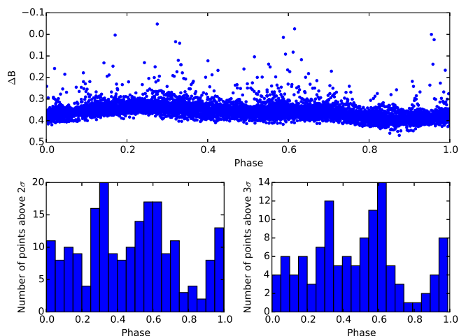
Fig. 5. Phased \Delta B light curves as used for flare statistics (top) and number of light curve points above 2\sigma/3\sigma after removing the effect of spottedness (bottom). Note that the top plot does not show the whole magnitude range of flares to better visualise the spotted light curve.
