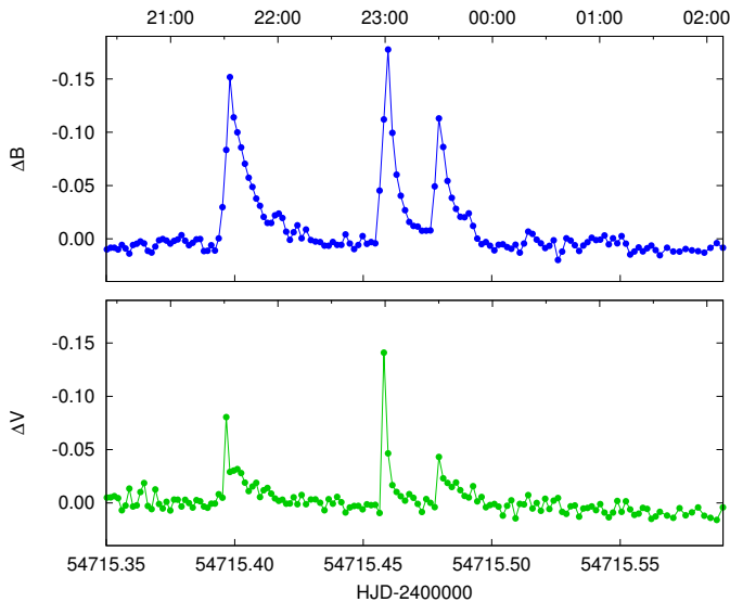
Fig. 10. \Delta B and \Delta V light curve of the complex flare event from HJD 2454715.
