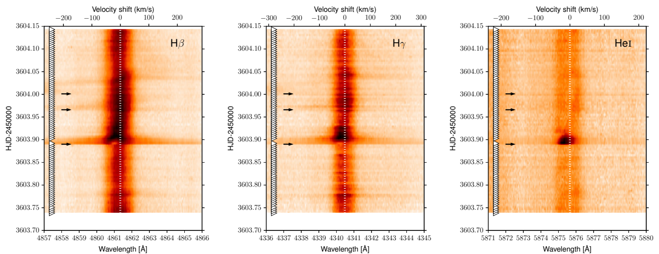
Fig. 13. Dynamic H \beta , H \gamma , and He I spectra of V374 Peg from HJD 2453603, showing strong flare events. Arrows mark the start of the blue wing enhancements (see text).
