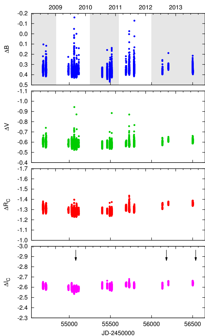
Fig. 1. BV(RI)_C photometry of V374 Peg from the Pizskéstető observations. Ranges marked in the \Delta B light curve were used for flare statistics (see Section 4.1). Arrows over the \Delta I light curve mark the dates of the spectroscopic observations during this time.
