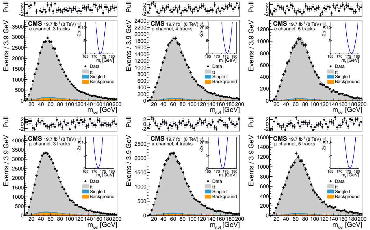
Figure 7: Template fits to the observed m_{\text{svl}} distributions for the semileptonic channels (e and \mu from top to bottom row), and for exactly three, four, and five tracks assigned to the secondary vertex (from left to right column). The top panels show the bin-by-bin difference between the observed data and the fit result, divided by the statistical uncertainty (pull). The inset shows the scan of the negative log-likelihood as a function of the calibrated top quark mass, accounting only for the statistical uncertainty, when performed exclusively in each event category.
