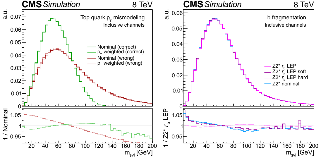
Figure 8: Variation of the simulated m_{\text{svl}} shape with systematic effects: reweighting of the simulated top quark p_T shape to the observed distribution, separately for correct and wrong lepton-vertex pairings (left); and different b quark fragmentation function shapes (right). The bottom panels in the two plots show the ratios between the top quark p_T reweighted and nominal shapes for the correct and wrong pairings (left), and between the various fragmentation models and the central Z2^* LEP r_b tune (right).
