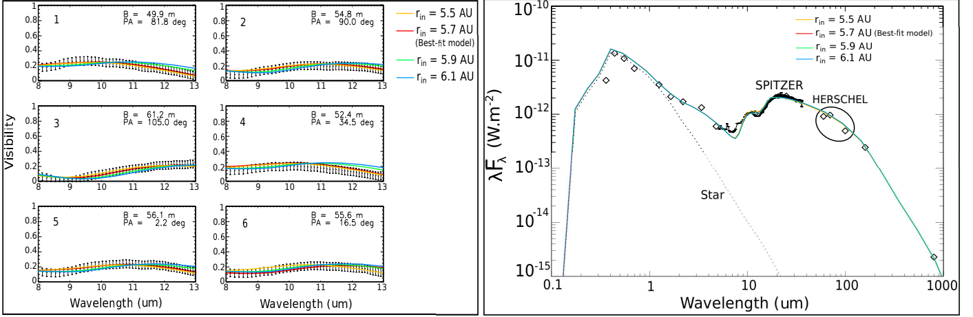
Fig. A.5. Same as in Fig. A.1 but focusing on the effect on a change of the inner radius of the outer disk r_{\text{in}} .
