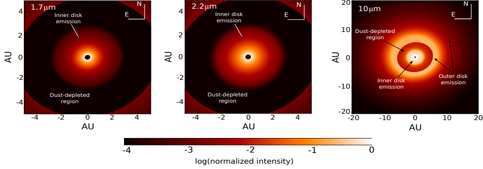
Fig. 5. Synthetic images of our best-fit RADMC3D model at \lambda = 1.7 \mu\text{m} (PIONIER), \lambda = 2.2 \mu\text{m} (AMBER), and \lambda = 10 \mu\text{m} (MIDI). For each image, the intensity is normalized to one at maximum and represented on logarithmic scale (central star is removed).
