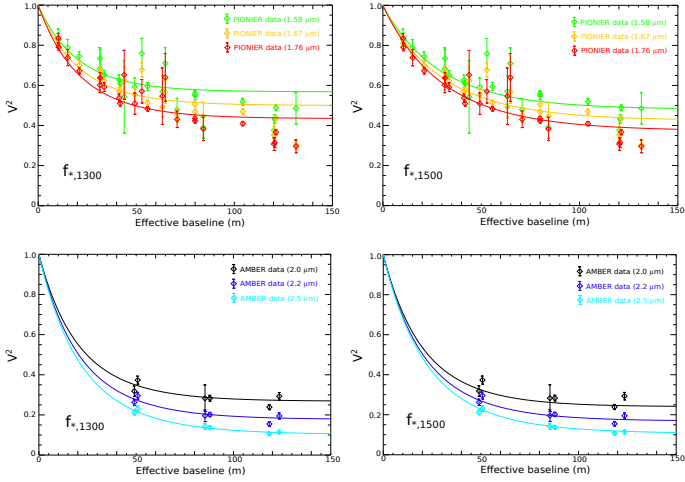
Fig. 2. Best-fit Lorentzian model (solid line) for PIONIER and AMBER overplotted on their measured V^2 , as a function of the effective baseline (see Eq.1). For clarity, we only plot the AMBER V^2 at \lambda = 2.0 \mu\text{m} , 2.2 \mu\text{m} , and 2.5 \mu\text{m} .
