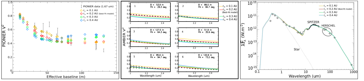
Fig. A.1. Effect on a change of the inner disk's inner radius r_{in} . We show the modeled H -band V^2 at 1.67 \mu\text{m} (left), K -band V^2 (middle), and SED (right), overplotted on the measured PIONIER V^2 , AMBER V^2 , and SED, respectively. The best-fit model is shown in red.
