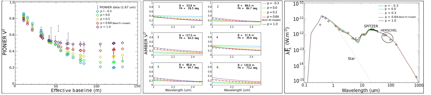
Fig. A.2. Same as in Fig. A.1 but focusing on the effect on a change of the p -exponent of the power-law profile of the inner disk's dust surface density.
