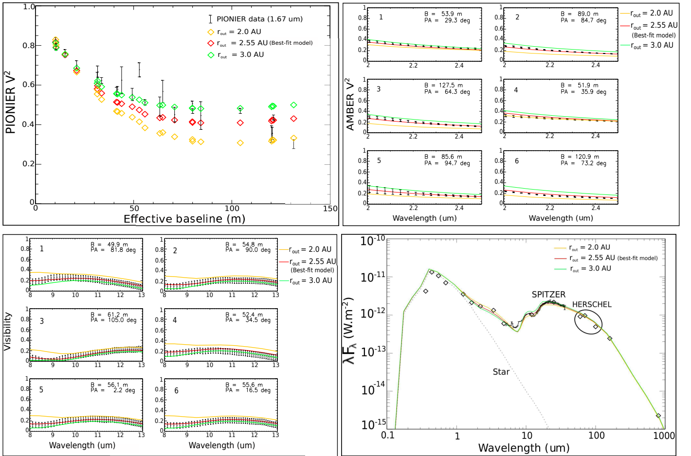
Fig. A.3. Same as in Fig. A.1 but focusing on the effect on a change in the outer radius of the inner disk r_{out} . We also included the modeled N -band visibilities, overplotted on the measured MIDI visibilities (bottom left).
