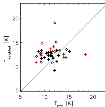
Fig. 8. T_{\text{ECC}} vs T_{\text{weighted}} distribution. Red symbols indicate the clumps without 70\ \mu\text{m} point sources. Plus signs indicate the clumps in the outer part of the Galaxy, diamonds indicate the sources in the inner Galaxy.
