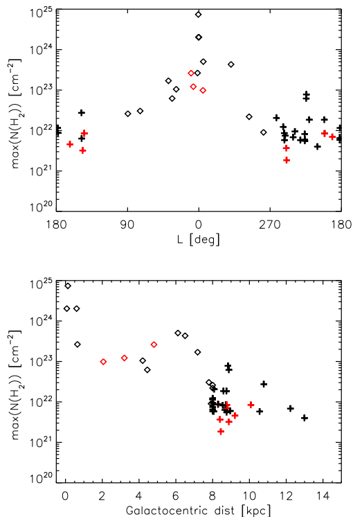
Fig. 6. Peak \text{H}_2 column density distribution of the ECC clumps as a function of Galactic longitude for the 48 objects (top) and Galactocentric distance for the 40 clumps with available distance estimates (bottom). Red symbols indicate the clumps without 70\ \mu\text{m} point sources.
