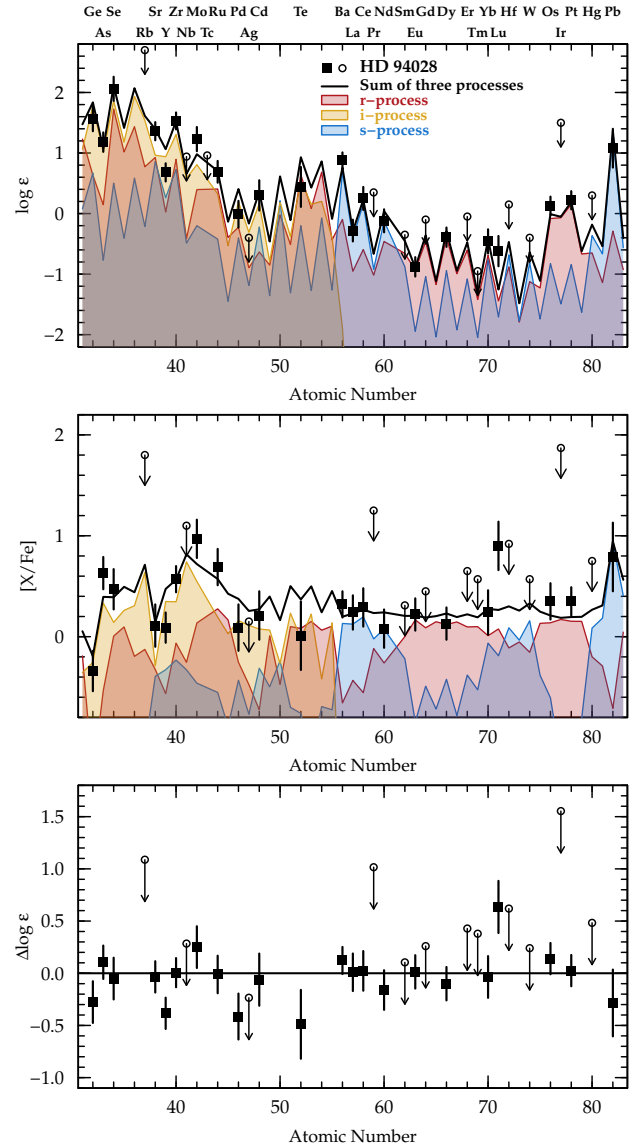
FIG. 7.— Comparison of the observed abundance pattern in HD 94028 and contributions from the s -process (blue), r -process (red), and i -process (gold) models. The s -process component is taken from the 1.7 M_{\odot} TP-AGB model discussed in Section 5.2. The r -process component is based on the solar r -process residuals and modified as described in Section 5.2. The i -process component is based on the trajectory from Bertolli et al. (2013) and tuned to maximize production in the As–Mo region as described in Section 5.4. The solid black line marks the sum of the three processes for each element. The overall normalization is expressed as \log \epsilon and [\text{X}/\text{Fe}] in the top and middle panels, and the bottom panel illustrates the residuals between the observed abundance pattern and the sum of the models.
