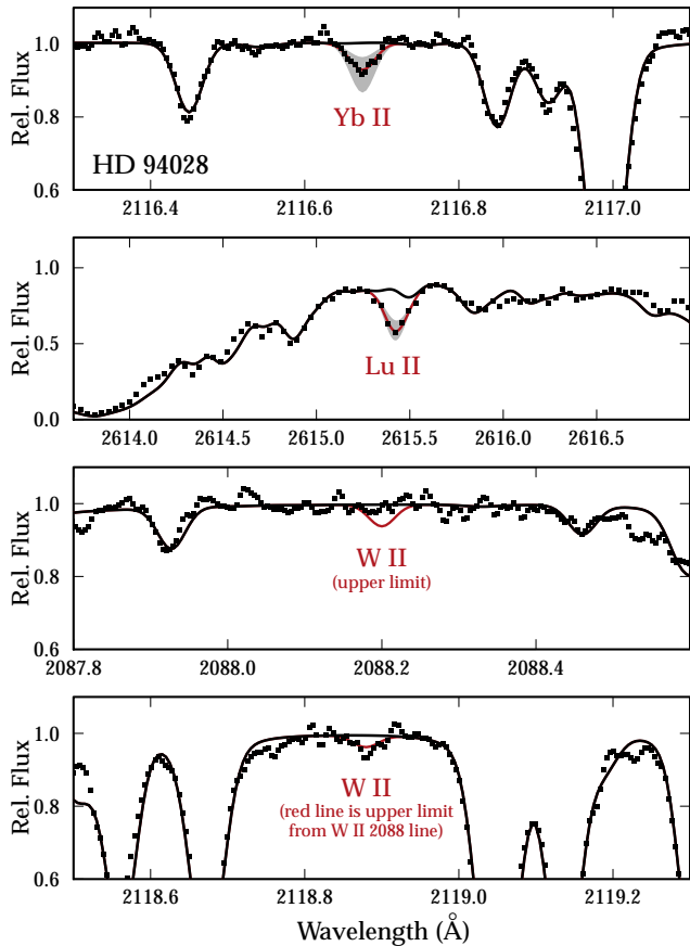
FIG. 3.— Comparison of observed and synthetic spectra for a selection of Yb II, Lu II, and W II lines. The squares mark the observed spectrum of HD 94028. For Yb II and Lu II, the red line marks the best-fit abundance, and the gray shaded region represents a change in the best-fit abundance by a factor of \approx two ( \pm 0.3 dex). For W II, the red line represents the upper limit derived from the line at 2088.20 Å. The bold black line represents a synthesis with no Yb, Lu, or W present.
