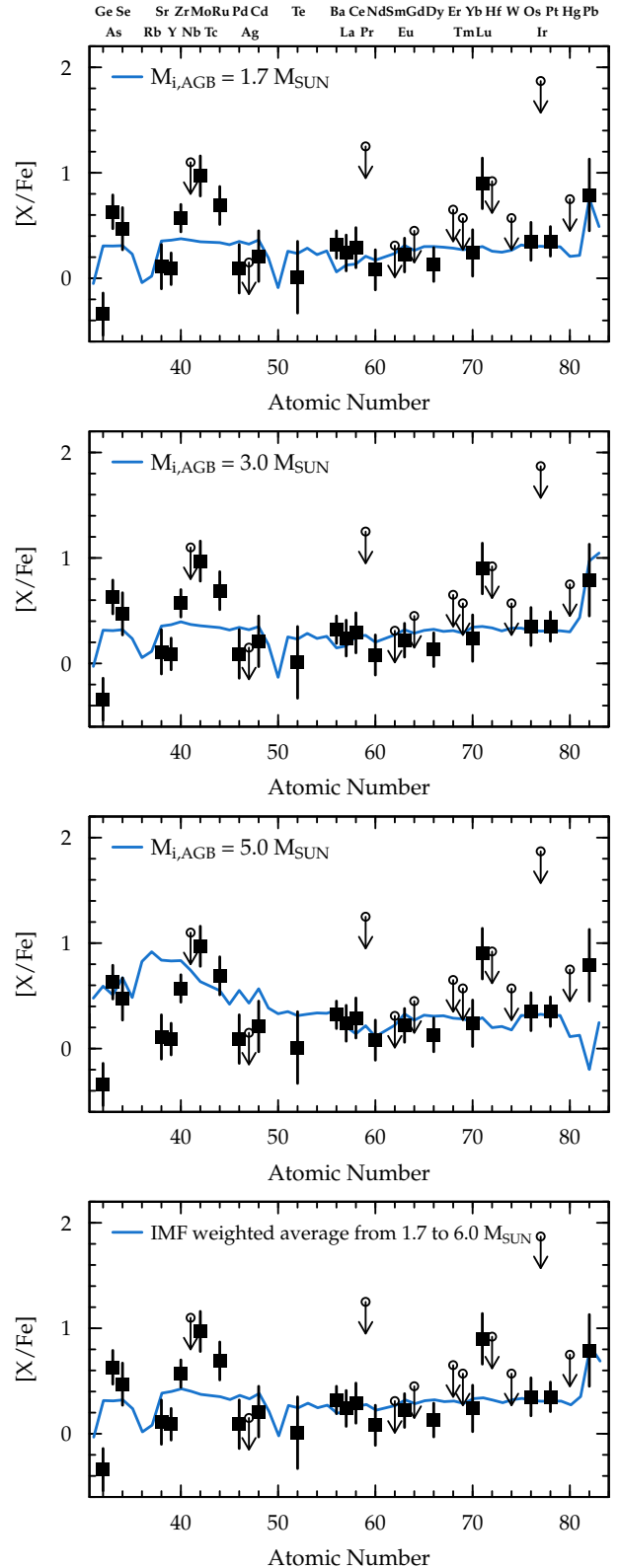
FIG. 5.— Comparison of derived abundances (black symbols) and four model fits (lines). The final ejected AGB s -process yields have been diluted by 1.2%, 1.2%, 13%, and 1.8% for the 1.7 M_{\odot} , 3.0 M_{\odot} , 5.0 M_{\odot} , and IMF-weighted models. An r -process component, scaled up by a factor of 2 relative to HD 108317, is included in each fit.
