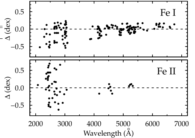
FIG. 1.— Fe abundance trends, relative to the mean abundance for transitions with \lambda > 3800 \text{ \AA} (dashed line), as a function of wavelength.
