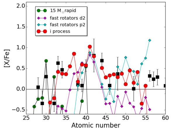
FIG. 6.— Comparison of the observed abundance pattern in HD 94028 with several model predictions for the mass region from Co to Ba. The observed abundance ratios are marked by black squares. The small green circles show the predictions for yields from the 15 M_{\odot} CCSN model (Pignatari et al. 2013), the purple and teal diamonds show the predictions for yields from the fast-rotating massive stars (Pignatari et al. 2008) multiplied (“p2”) and divided (“d2”) by a factor of 2, and the large red circles show the predictions for yields from the i process. Black squares mark the observed abundance ratios. The solid line marks the solar ratios.
