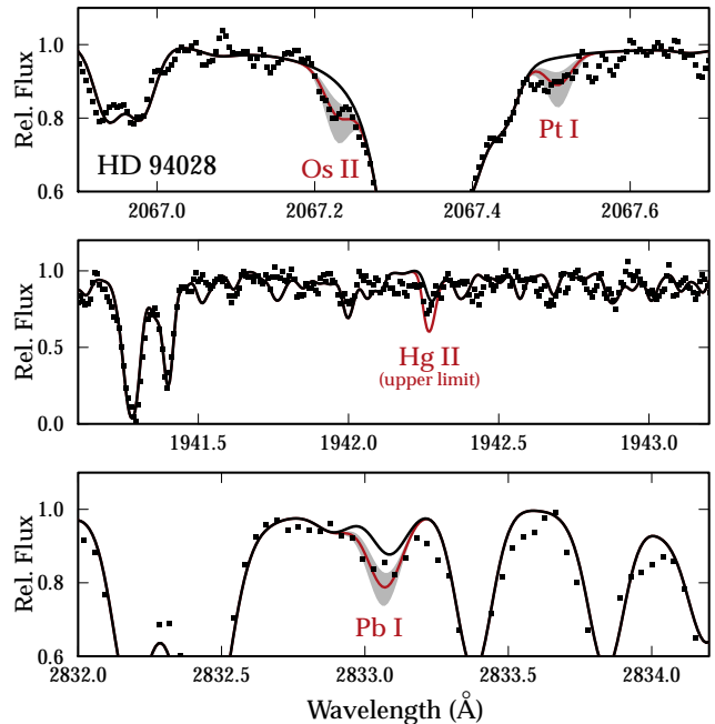
FIG. 4.— Comparison of observed and synthetic spectra for a selection of Os II, Pt I, Hg II, and Pb I lines. The squares mark the observed spectrum of HD 94028. For Os II, Pt I, and Pb I, the red line marks the best-fit abundance, and the gray shaded region represents a change in the best-fit abundance by a factor of \approx two ( \pm 0.3 dex). For Hg II, the red line represents the upper limit derived assuming Hg II is responsible for all absorption at 1942.27 Å. The bold black line represents a synthesis with no Os, Pt, Hg, or Pb present.
