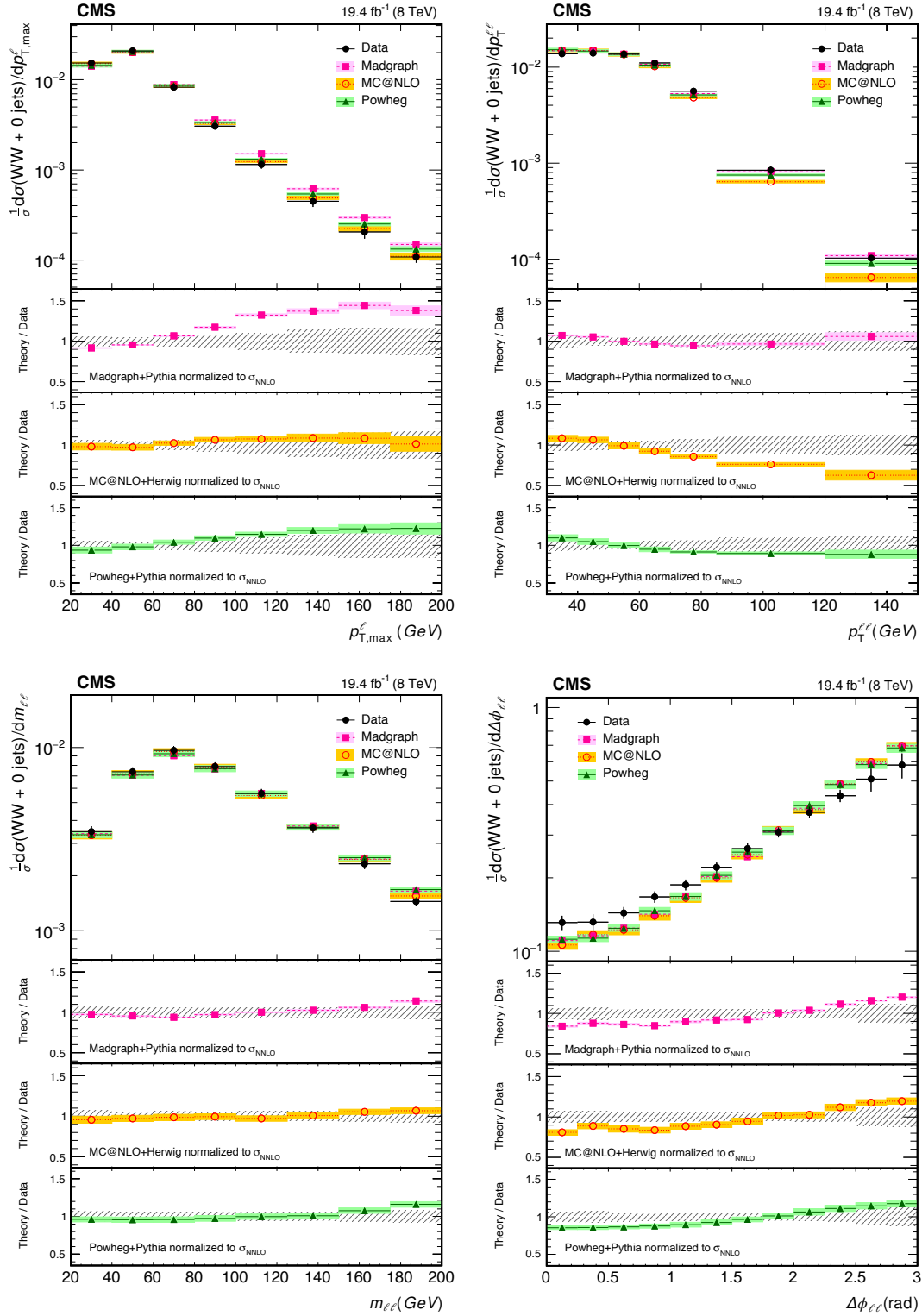
Figure 3: Normalized differential W^+W^- cross section as a function of the leading lepton p_T ( p_{T,\max}^{\ell} ) (top left), the transverse momentum of the dilepton system ( p_T^{\ell\ell} ) (top right), the invariant mass ( m_{\ell\ell} ) (bottom left) and the angular separation between leptons ( \Delta\phi_{\ell\ell} ) (bottom right). Both statistical and systematic uncertainties are included. The hatched area in the ratio plots corresponds to the relative error of the data in each bin. The measurement, including gg \rightarrow W^+W^- is compared to predictions from MADGRAPH, POWHEG, and MC@NLO.
