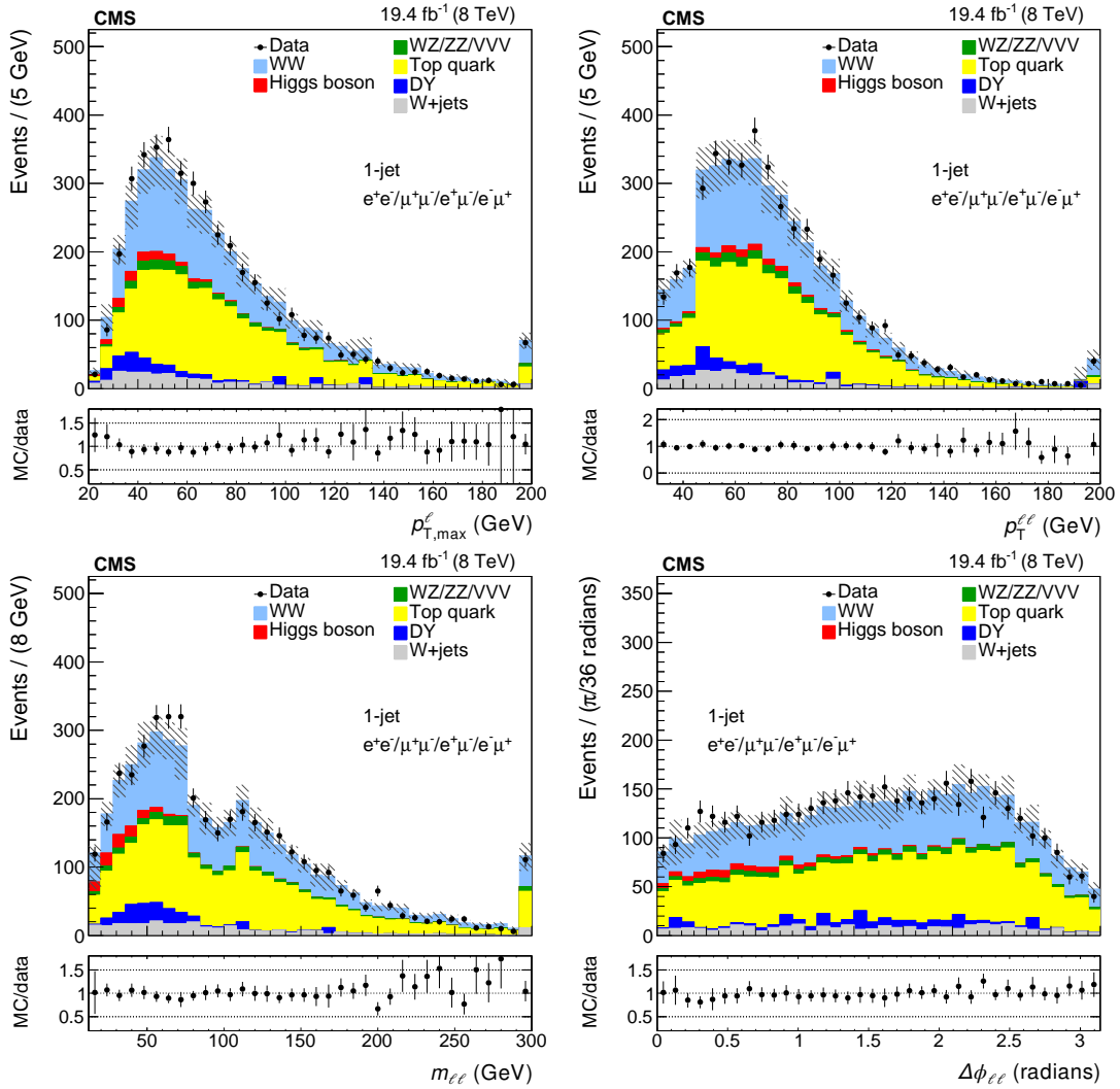
Figure 2: The data and MC distributions for the one-jet category of the leading lepton p_T ( p_{T, \max}^{\ell} ), the p_T of the dilepton system ( p_T^{\ell\ell} ), the dilepton invariant mass ( m_{\ell\ell} ) and the azimuthal angle between the two leptons ( \Delta\phi_{\ell\ell} ). The hatched areas represent the total systematic uncertainty in each bin. The error bars in the ratio plots are calculated considering the statistical uncertainty from the data sample and the systematic uncertainties in the background estimation and signal efficiency. The last bin includes the overflow.
