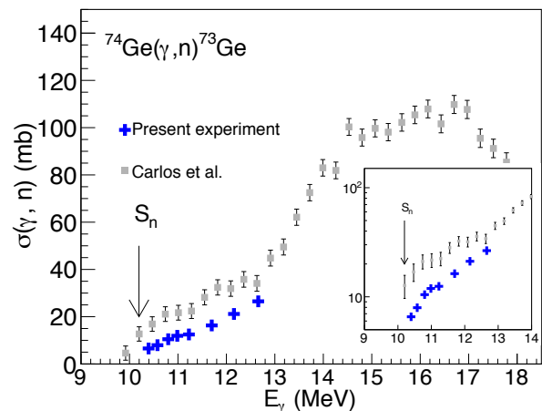
FIG. 2: (Color online) Cross sections for the ^{74}\text{Ge}(\gamma, n)^{73}\text{Ge} reaction from the current experiment (blue crosses) together with existing photo-neutron data [35].
