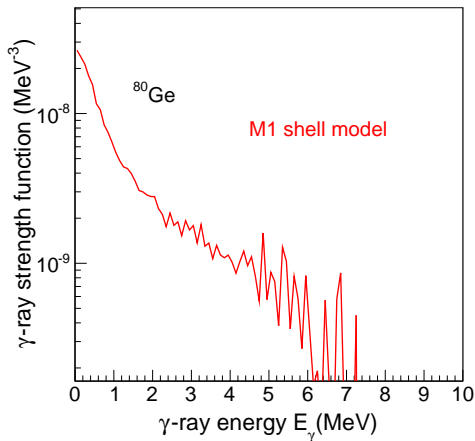
FIG. 7: (Color online) Shell model calculations of the M1 component of the \gamma SF of ^{80}\text{Ge} (red line).
