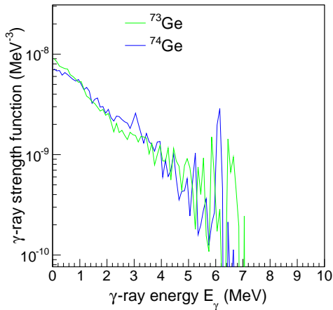
FIG. 6: (Color online) Shell model calculations of the M1 component of the \gamma SF of ^{74}\text{Ge} (blue line) and ^{73}\text{Ge} (green line).
