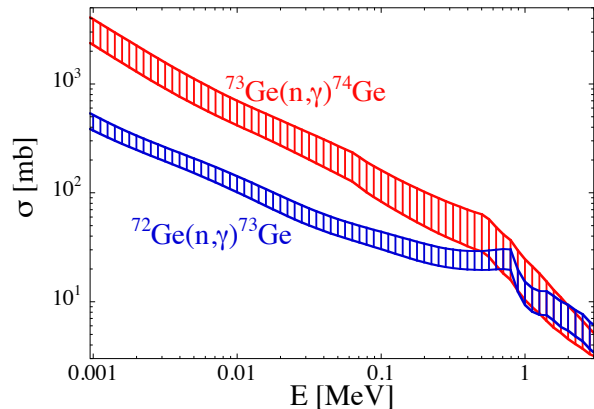
FIG. 8: (Color online) Neutron capture cross section, \sigma , as a function of neutron energy, E , for the ^{72}\text{Ge}(n, \gamma)^{73}\text{Ge} and ^{73}\text{Ge}(n, \gamma)^{74}\text{Ge} reactions. The calculations are performed using TALYS. See text for details.
