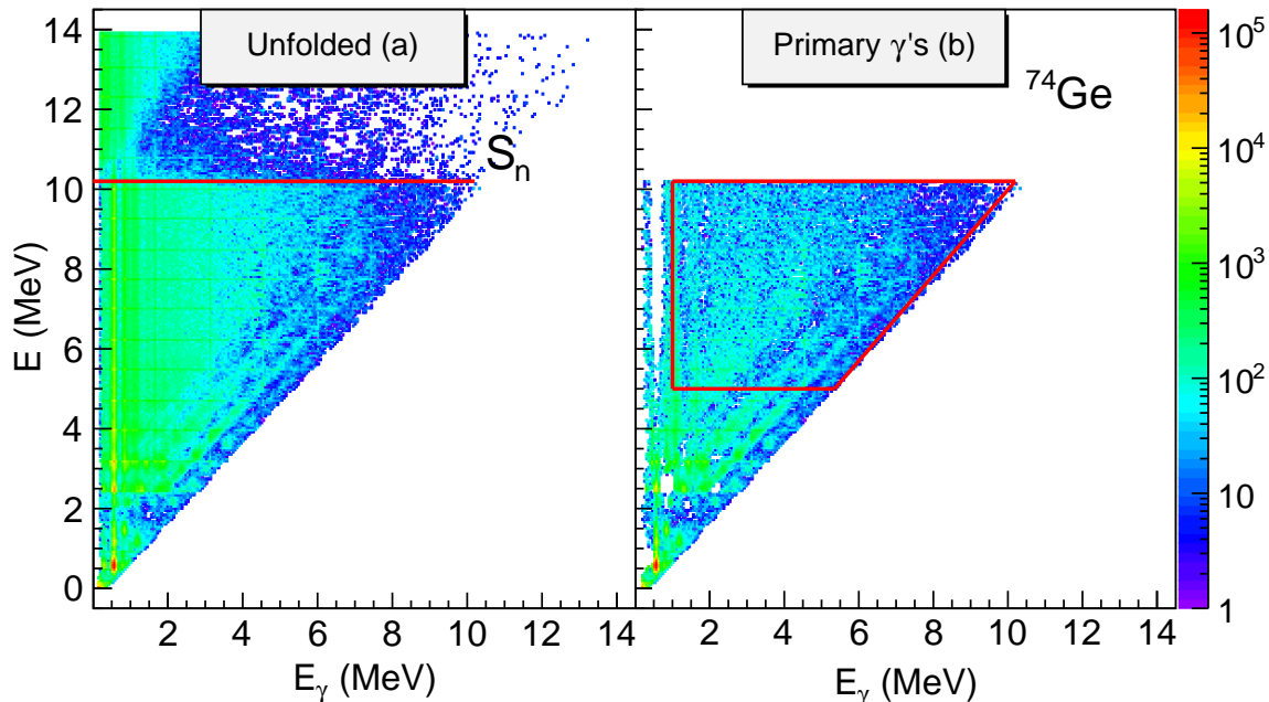
FIG. 1: (Color online) (a) Excitation energy- \gamma matrix from the ^{74}\text{Ge}(^3\text{He}, ^3\text{He}\gamma)^{74}\text{Ge} reaction. The NaI spectra are unfolded with the NaI response functions. (b) The first generation matrix from the same reaction.
