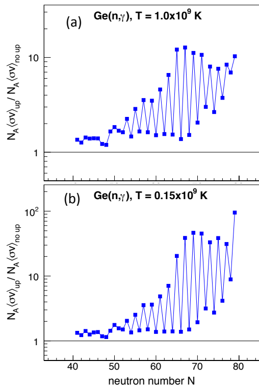
FIG. 9: (Color online) Ratio of Maxwellian-averaged (n, \gamma) reaction rates including and excluding the upbend for the Ge isotopic chain up to the neutron drip line for temperatures (a) T = 1 GK and (b) T = 0.15 GK.
