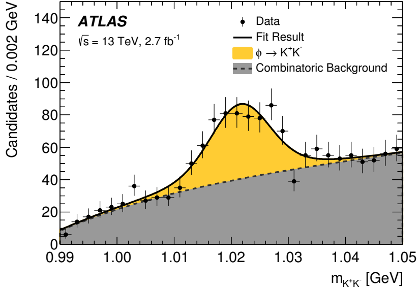
Figure 1: The m_{K^+K^-} distribution of selected \phi \gamma combinations with the complete event selection applied (see text), apart from the requirement on m_{K^+K^-} . The data are fitted with the convolution of a Breit-Wigner distribution, using the \phi width [34], and a Gaussian distribution to represent the experimental resolution, while the background is modeled with an analytical function, commonly used to describe a kinematic threshold [38].
