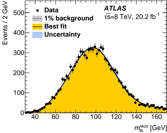
(c) Fit to m_{lb}^{\text{reco}} in data
