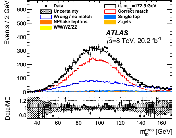
(b) m_{lb}^{\text{reco}} in data and simulation
