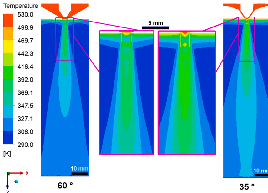
Fig. 7. Counter plots of air temperature profiles for the air knife with half-cone opening angles of 60° and 35° at the air pressure of 2 bar.
