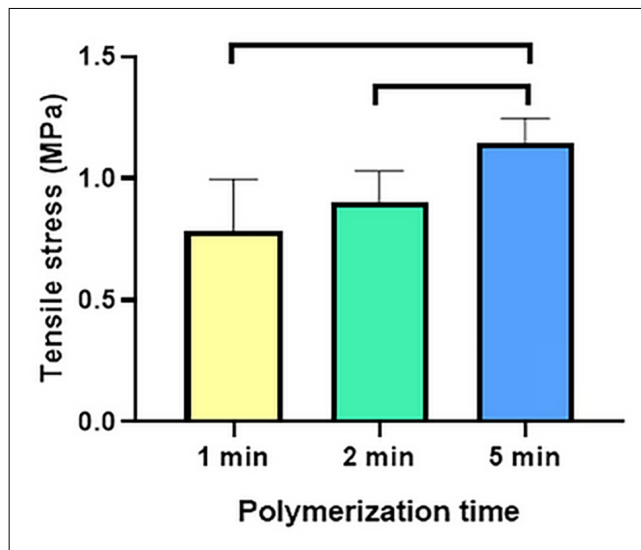
Figure 2: Tensile stress data (MPa) at different polymerization time
