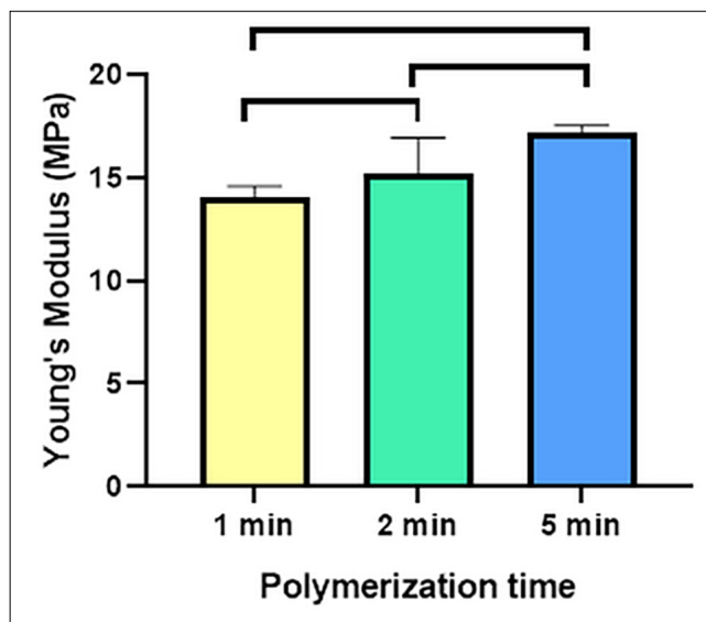
Figure 3: Young's Modulus (MPa) at different polymerization time
