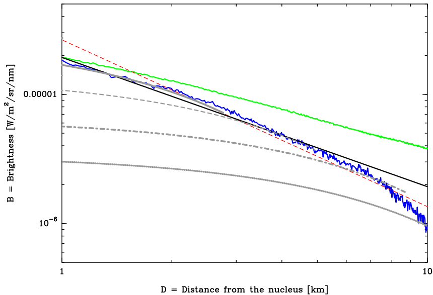
Figure 7. 2015-05-30T16:43:38 - In blue is the radial profile for the jet and in green are the radial profile for the coma background. In red is the D^{\beta} -fit for the jet. In grey are the result of sublimation of the aggregates of dirty grains with a radius at a = 5\mu\text{m} (Solid Line), a = 10\mu\text{m} (Dashed Line), a = 20\mu\text{m} (Dash-Dotted Line) and a = 50\mu\text{m} (Dotted Line). In black is the radial profile over a cone.
