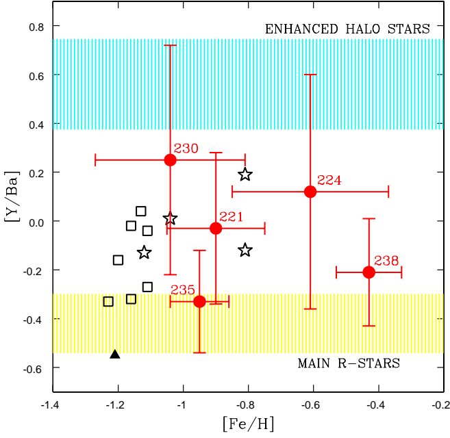
Fig. 13. [Y/Ba] vs. [Fe/H] diagram for the sample stars and results from literature. Symbols are the same as in Figs. 8. The yellow and cyan regions correspond to the main r-process signature and the abundance ratio from metal-poor stars enhanced in the lightest heavy elements (see text for details).
