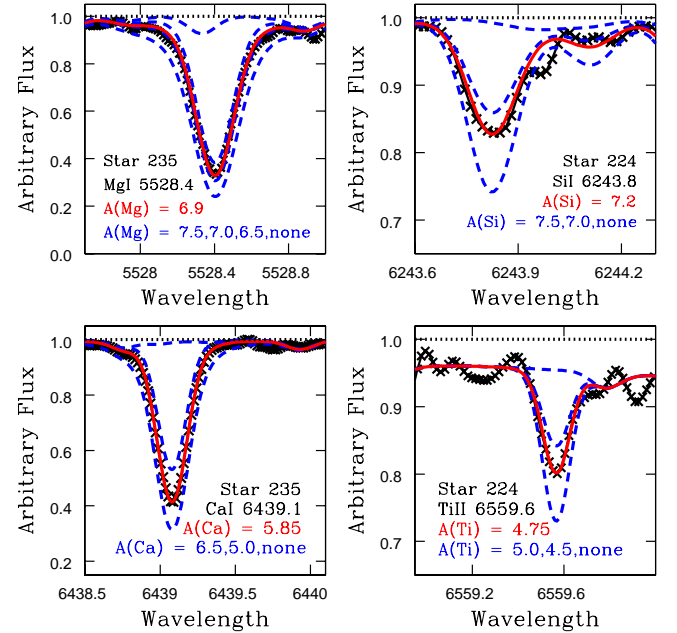
Fig. 6. Upper left panel: Fit to the Mg I 5528.4 \text{ \AA} line in star 235. Upper right panel: Fit to the Si I 6243.8 \text{ \AA} line in star 224. Lower left panel: Fit to the Ca I 6439.1 \text{ \AA} line in star 235. Lower right panel: Fit to the Ti II 6559.6 \text{ \AA} line in star 224. Symbols are the same as in Fig. 4 (upper panel).
