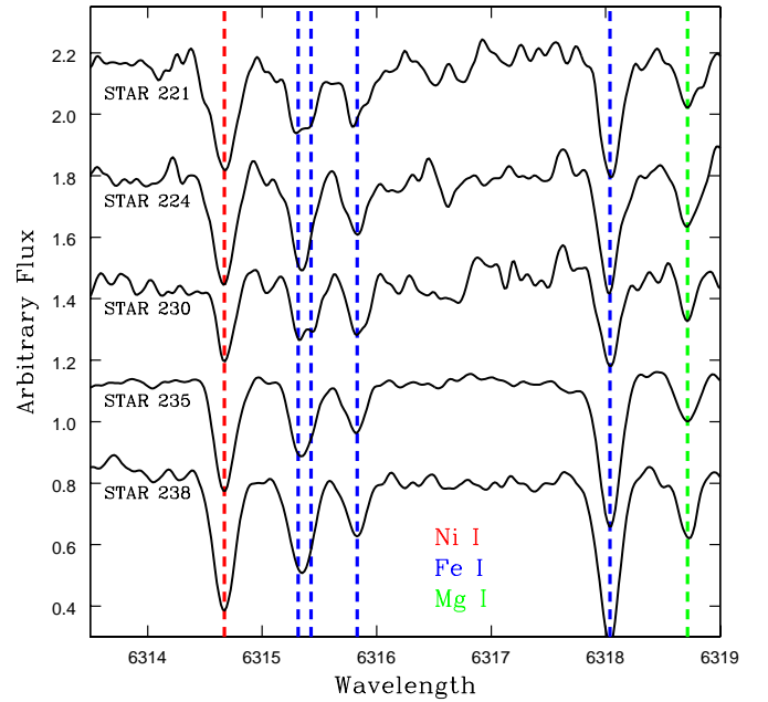
Fig. 1. Portion of the final data. The dashed lines show Ni I (red), Fe I (blue), and Mg I (green) lines located in this wavelength range.
