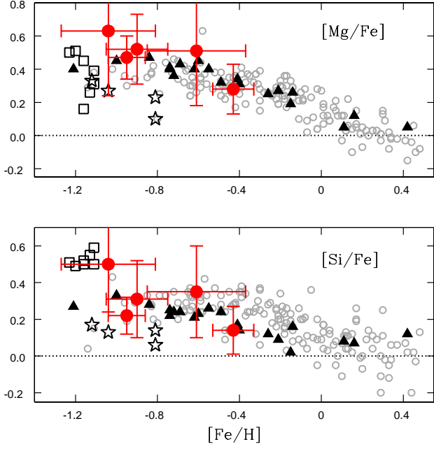
Fig. 9. [\text{Mg}/\text{Fe}] (upper panel) and [\text{Si}/\text{Fe}] (lower panel) abundance ratios as a function of the metallicity for the five sample stars, compared with literature abundances. Symbols are the same as in Fig. 8.
