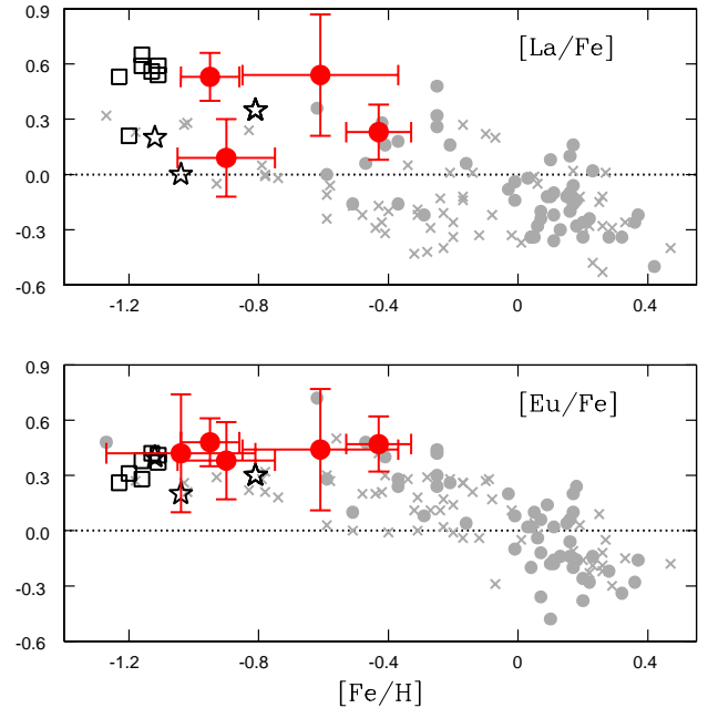
Fig. 12. [La/Fe] (upper panel) and [Eu/Fe] (lower panel) abundance ratios as a function of the metallicity for the five sample stars, compared with literature abundances. Symbols are the same as in Figs. 8 and 11.
