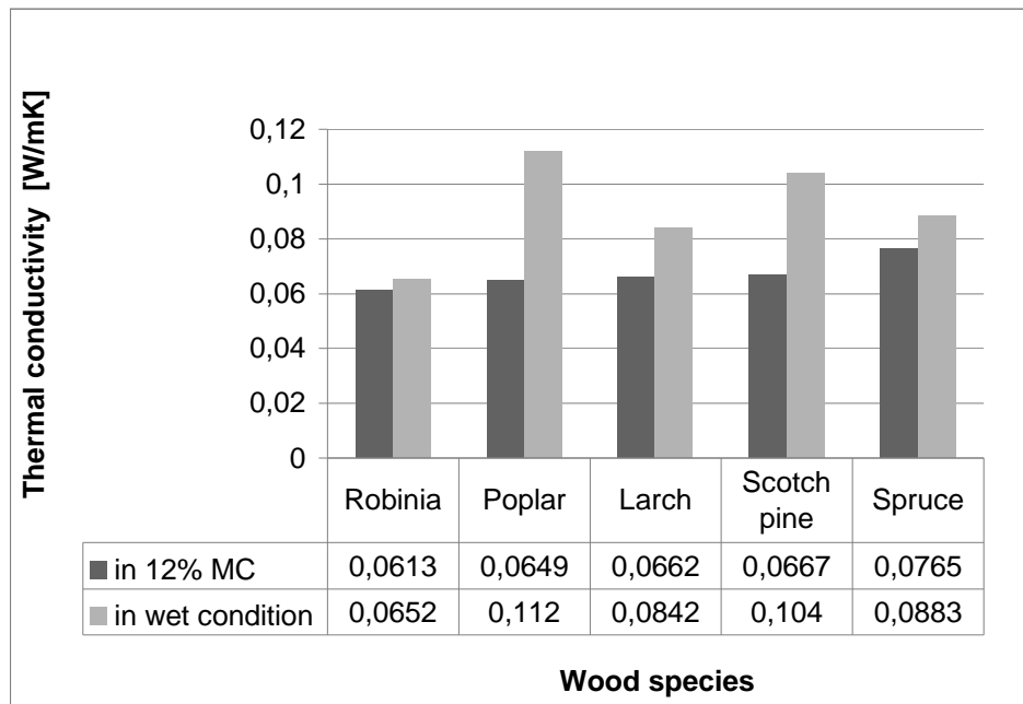
Figure 2. Thermal conductivity of different chipped wood barks in different moisture content
