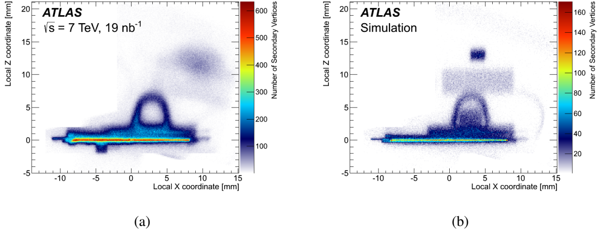
Figure 10: Number of selected secondary vertices in the local coordinate frame of the pixel module, for (a) data, and (b) MC simulation, in the first barrel layer. The data sample has more events than the simulated sample.
