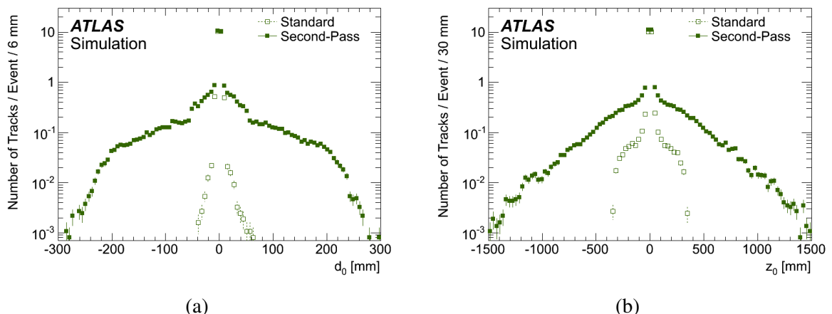
Figure 2: Distributions of (a) transverse ( d_0 ) and (b) longitudinal ( z_0 ) impact parameters of tracks in simulated events. Open squares show tracks reconstructed with the standard algorithm, closed squares show tracks reconstructed with either the standard or second-pass reconstruction algorithm.
