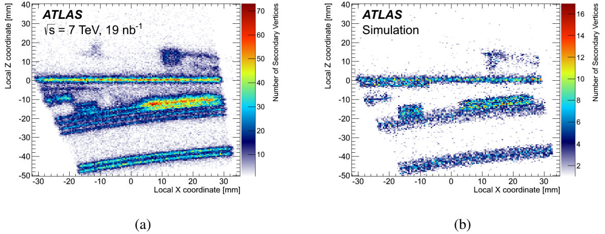
Figure 11: Number of selected secondary vertices in the local coordinate frame of the SCT module, for (a) data and (b) MC simulation, in the first barrel layer. The data sample has more events than the simulated sample.
