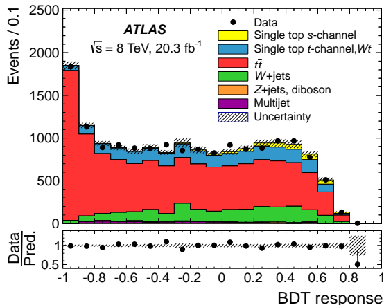
Figure 2: Observed and predicted distributions of the BDT response. The simulated distributions are normalized to the result of the binned maximum-likelihood fit. The hatched band represents the normalization uncertainty of all processes after the fit added in quadrature with the simulation statistical uncertainty. The lower panel shows the ratio of data to prediction.
