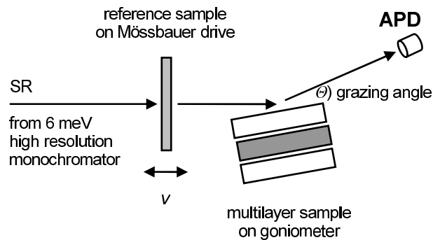
Fig. 1. Experimental setup for stroboscopic Synchrotron Mössbauer Reflectometry.
