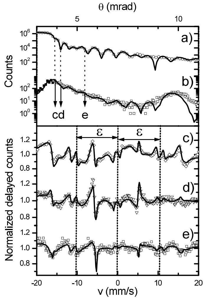
Fig. 2. Prompt electronic (a) and delayed nuclear reflectivity (b) curves as well as stroboscopic SMR spectra (c) to e), of a [\text{natFe}/^{57}\text{Fe}]_{10} isotopic multilayer at grazing angles indicated by the arrows. Vertical dotted lines in panels c) to e) indicate the center of the zero and \pm 1 order stroboscopic bands separated by \varepsilon \approx 10.93 mm/s for the applied observation window period.
