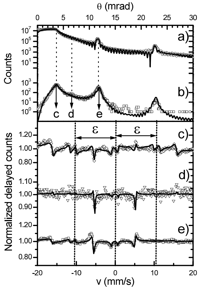
Fig. 4. Prompt electronic (a) and delayed nuclear (b) reflectivity curves as well as stroboscopic SMR spectra (c to e) of a ^{57}\text{Fe} (2.6 nm)/Cr (1.3 nm) _{20} /MgO anti-ferromagnetic multilayer at various angles indicated by arrows. The consecutive Fe layer magnetizations are aligned perpendicular to the SR beam. Vertical dotted lines in panels c) to e) indicate the center of the zero and \pm 1 order stroboscopic bands separated by \varepsilon \approx 10.93 mm/s for the applied observation window period.
