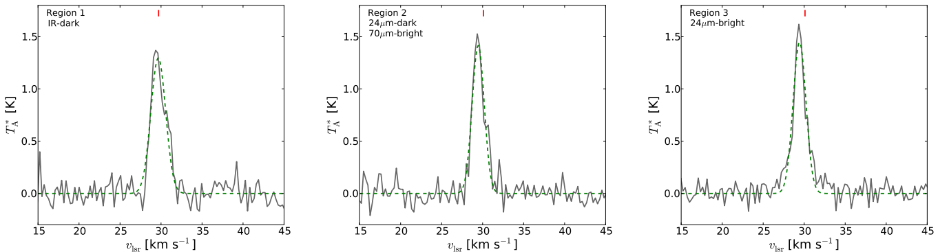
Fig. 4. Solid lines show spectra of \text{C}^{18}\text{O} (2-1) (green) from the IRAM 30-meter telescope averaged over the 12'' regions (see Table 1), and the dashed green lines show the best single component Gaussian fits to the data. The fit parameters are summarised in Table 3. The red vertical line indicates the velocity centroid from the fits to the PdBI+MOPRA \text{N}_2\text{H}^+ (1-0) data.
