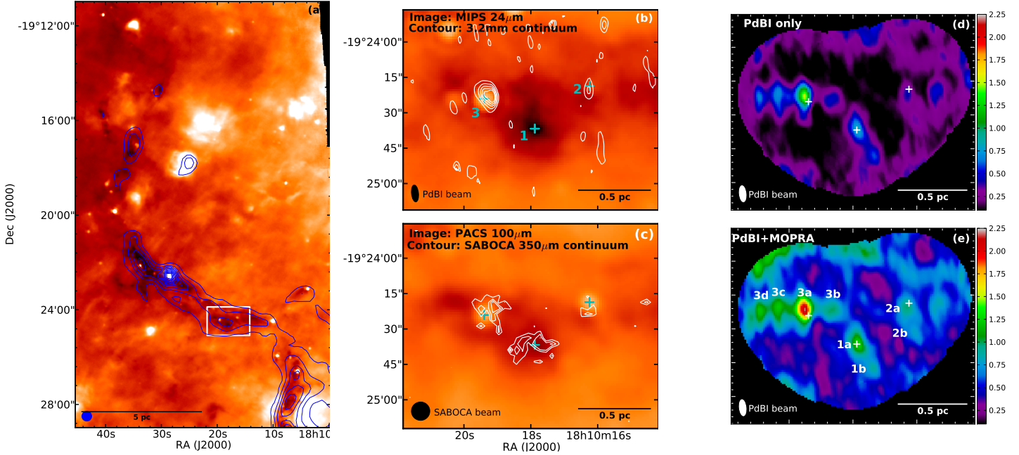
Fig. 1. (a): The full G11 filament seen at 70\ \mu\text{m} with Herschel /PACS with SPIRE 350\ \mu\text{m} contours over-plotted from 9\ \text{Jy beam}^{-1} increasing in steps of 3\ \text{Jy beam}^{-1} (adapted from Henning et al. 2010). The SPIRE 350\ \mu\text{m} beam (FWHM) is shown in the lower-left corner. The white rectangle marks the area shown in the rest of the panels. (b) MIPS 24\ \mu\text{m} image with 3.2\ \text{mm} continuum contours from a PdBI-only map. The contour levels are from 0.2 to 0.12\ \text{mJy beam}^{-1} in steps of 0.2\ \text{mJy beam}^{-1} . The synthesised beam is shown in the lower-left corner. (c) APEX-SABOCA 350\ \mu\text{m} continuum contours (Ragan et al. 2013) at 0.81, 1.08, 1.35\ \text{Jy beam}^{-1} plotted over the PACS 100\ \mu\text{m} image. The SABOCA 350\ \mu\text{m} beam (FWHM) is shown in the lower left. (d) Integrated intensity of \text{N}_2\text{H}^+ (1-0) from the PdBI-only map. (e) Integrated intensity of the combined PdBI+MOPRA map. Both (d) and (e) are integrated from 29 to 33\ \text{km s}^{-1} , and the units of the colourscale are \text{Jy beam}^{-1}\ \text{km s}^{-1} . The + signs indicate the positions of the main continuum cores identified in panel (b) and Table 1.
