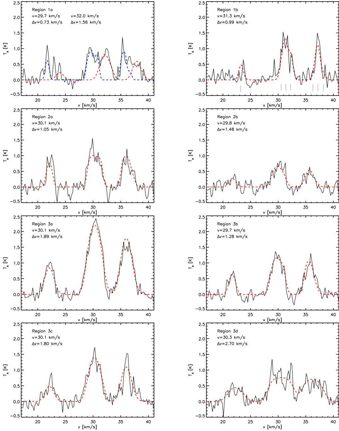
Fig. 2. \text{N}_2\text{H}^+ 1\rightarrow 0 spectra from the merged PdBI+MOPRA dataset (black lines) and the best fit parameters (red dashed lines, see Table 2). The positions seven hyperfine components (Caselli et al. 1995) are shown in the top-right panel.
