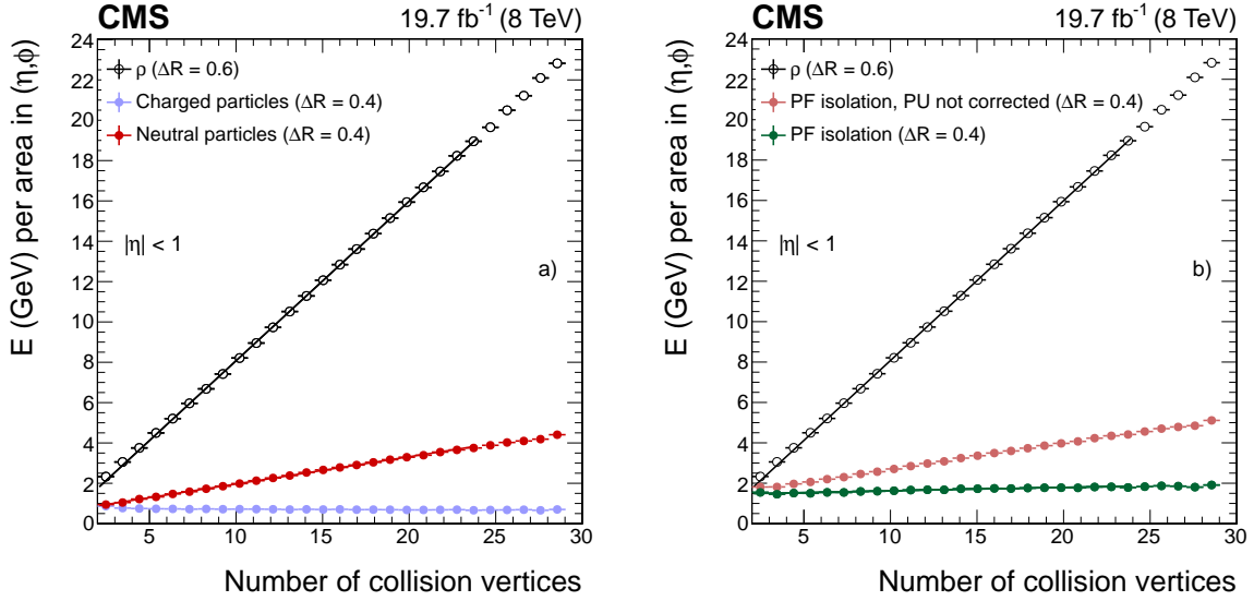
Figure 20: Average energy density as a function of the number of reconstructed proton-proton collision vertices, for electron candidates with p_T > 20 GeV and |\eta| < 1 from data dominated by Z \rightarrow e^+e^- events. The energy density \rho (open dots) is shown, along with each component of the particle isolation: a) neutral particles (red dots) and charged particles associated with the vertex (blue dots), and b) before (pink dots) and after (green dots) the correction for pileup on PF isolation.
