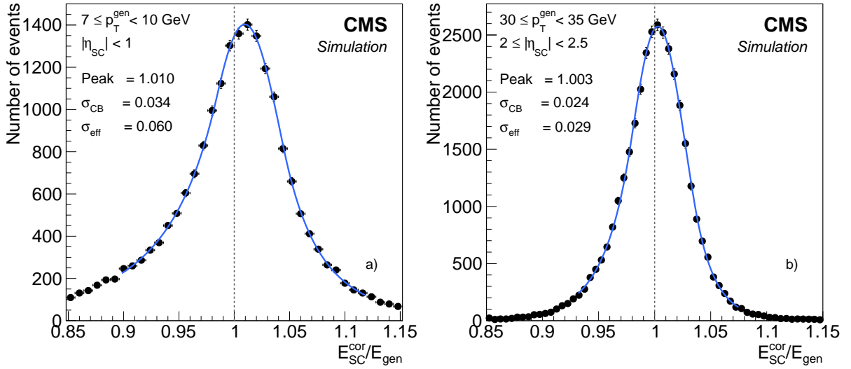
Figure 9: Example distributions of the ratio of corrected over generated supercluster energies ( E_{\text{SC}}^{\text{cor}}/E_{\text{gen}} ) and their (double Crystal Ball) fits, in two regions of \eta and p_{\text{T}} after implementing the regression corrections: for electrons a) with 7 \leq p_{\text{T}}^{\text{gen}} < 10 \text{ GeV} and |\eta_{\text{SC}}| < 1 , and b) with 30 \leq p_{\text{T}}^{\text{gen}} < 35 \text{ GeV} and 2 \leq |\eta_{\text{SC}}| < 2.5 , \eta_{\text{SC}} being defined relative to the centre of CMS. Electrons are generated with uniform distributions in \eta and p_{\text{T}} .
