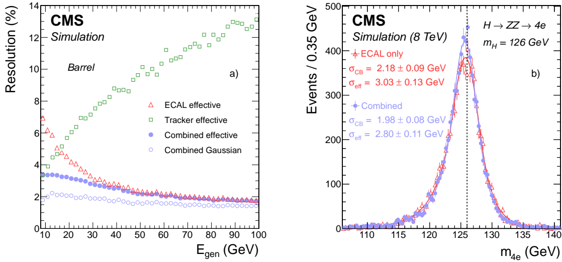
Figure 12: a) Effective resolution in electron momentum after combining E_{\text{SC}} and p estimates (solid circles), compared to those using the corrected SC energy (triangles), and the track momentum (squares), as a function of the generated energy for electrons in the barrel. Also shown is the resolution in momentum after combining E_{\text{SC}} and p estimates in terms of \sigma_{\text{CB}} (open circles), to illustrate the contribution of the Gaussian core of the distribution. Electrons are generated with uniform distributions in \eta and p_{\text{T}} . b) Reconstructed mass of the Higgs boson for H(126) \rightarrow ZZ^* \rightarrow 4e simulated events, using either the corrected SC energy (open triangles) or the electron momentum after combining E_{\text{SC}} and p estimates (solid dots) [9].
