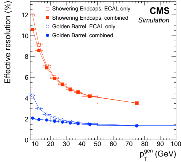
Figure 11: Effective resolution in electron momentum after combining the E_{\text{SC}} and p estimates (solid symbols), compared to that of the corrected SC energy (open symbols), as a function of the generated electron p_T . Golden electrons in the barrel (circles) and showering electrons in the endcaps (squares) are shown as examples. Electrons are generated with uniform distributions in \eta and p_T , and the resolution is shown after applying the resolution broadening.
