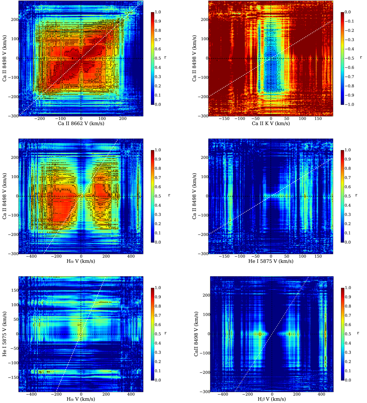
Fig. 3. Pixel-by-pixel velocity cross-correlations between different lines. From top to bottom, left to right: Ca II 8498 vs 8662Å, Ca II K vs Ca II 8498Å, Ca II 8498Å vs H \alpha , Ca II 8222Å vs He I 5875Å, H \alpha vs He I 5875Å and Ca II 8498Å vs H \beta . The correlation coefficient (estimated as a Spearman rank correlation with value r and false alarm probability p ) is shown on the right in the color scheme, with the contours marking the high significance ( p > 10^{-5} ) parts with r=0.6, 0.7, 0.8, 0.9 .
