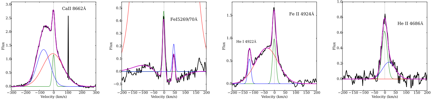
Fig. 4. Some of the multi-Gaussian fits for one of the dates (JD 2455674.82443). The normalised, continuum-subtracted observed spectra are displayed as thick black lines. Individual Gaussian components are plotted as thin lines (colours: green, red, blue, cyan). The combined fit is plotted as a magenta thick line. The zero velocities of the central line are also marked with a vertical dotted line. The plots are labelled with the line(s) elements and wavelength. Note that the very complex shape of the continuum around the Fe I 5269/70Å lines is better fitted by two strong Gaussians, one in emission and the other in absorption (partly out of the figure). These BC have no physical meaning/interpretation, but allow us to extract properly the strong NC of both lines.
