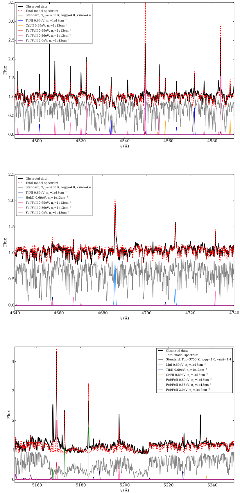
Fig. 11. Toy model for the narrow emission lines, obtained by considering an electron density 10^{13} \text{ cm}^{-3} and three different temperatures along the accretion column (8000, 10000, 23000 K). The rotationally-broadened standard star spectrum is shown in grey, and the individual lines are shown in various colors. The final model, including a constant veiling, is obtained by summing all three components.
