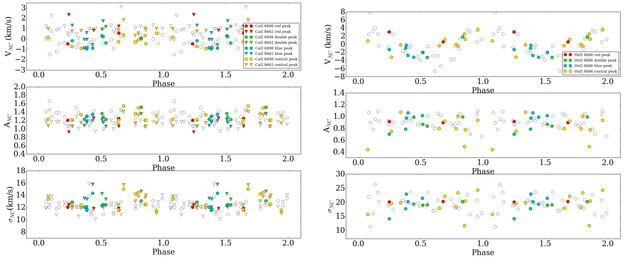
Fig. E.3. Shape of the BC (classified as "centred", "blueshifted", "redshifted", "double-peaked", see text) vs phase. Only data points with strong BC and a clear peak are classified.
