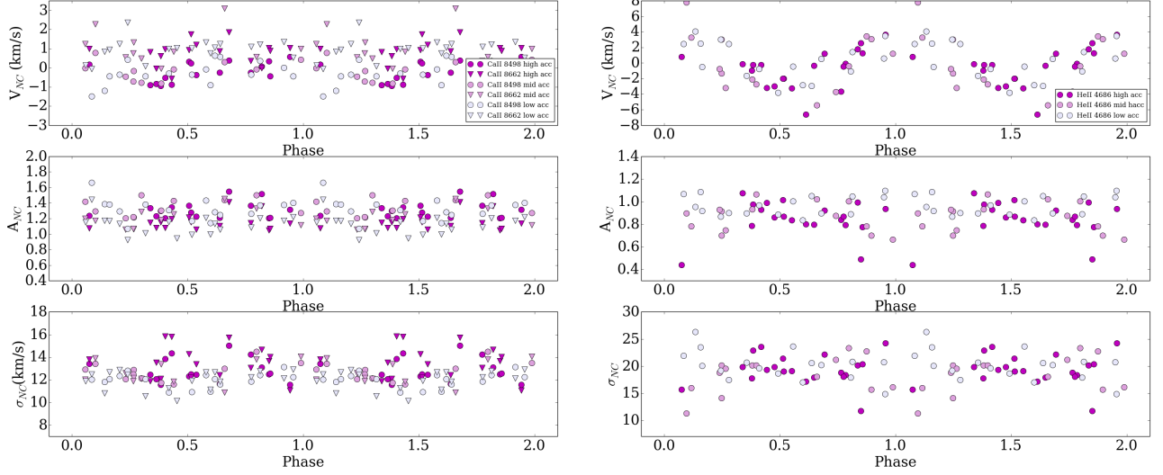
Fig. C.1. Line fit parameters for the NC of the Ca II IR (left) and He II lines (right), colour-coded according to their accretion rate (see text). The upper panel shows the radial velocity of the NC line ( V_{NC} ), the middle panel shows the amplitude of the NC line ( A_{NC} ), and the bottom panel shows the Gaussian width ( \sigma_{NC} ). There is no evident modulation of the RV with the accretion rate, and only the line width for the Ca II NC seems to be higher for the higher accretion rates, although this could be also an effect of the presence of a stronger underlying BC. The signatures observed in the NC are thus very robust with respect to variations of the accretion rate within one order of magnitude.
