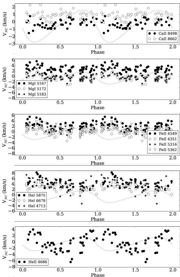
Fig. 6. Phase-folded curves (using the photospheric absorption line period and phase, which is nearly identical to the He II 4686Å one)) for several of the observed NC of lines. Note that two 7.417d periods are plotted for clarity. The dotted line represents the RV curve measured for the photospheric absorption lines (K14).
