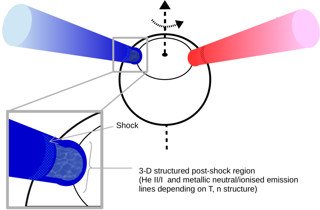
Fig. 8. A cartoon of a star with an accretion column that is visible at all times due to the stellar inclination and whose emission lines suffer Doppler shift as the star rotates (the observer is located perpendicular to the plane of the paper). The blue (red) column shows the position at which the lines originated in it would appear blueshifted (redshifted) to an observer looking from out of the page. The hashed areas mark the shock region. We suggest that the observed narrow emission lines are produced in the post-shock area, which is stratified in density and temperature. Lines produced in the shock region (He II, requiring very hot and dense conditions) originate in a nearly flat structure, so their periodic signatures are much stronger and less messy than other lines produced in the extended, infalling post-shock region. The BC is produced in the accretion column before the pre-shock region, showing higher velocity offsets as they rotate with/around the star. Not to scale: note that the shock region is at a very small distance over the photosphere, compared to the stellar radius.
