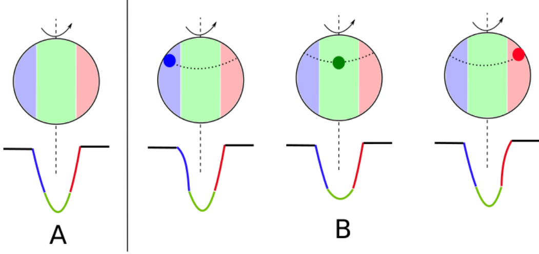
Fig. 7. A scheme of how the photospheric absorption lines are affected when a hot spot moves in and out of our line of sight when the star rotates. In A we show the different parts of the stellar photosphere that produce the photospheric absorption lines. B shows how the line is affected when a hot spot is included. When the absorption deficit associated to the spot appears blueshifted, the centre of the photospheric lines seems to move towards the red. When the spot appears redshifted, the centre of the absorption line appears shifted towards the blue. Small emission lines are visible within some of the photospheric absorption lines, tracking the local rotational velocity of the part of the stellar surface where the line originates. Non-photospheric lines or lines that are particularly strong on the spot could appear simply as emission lines over the continuum, without any underlying absorption.
