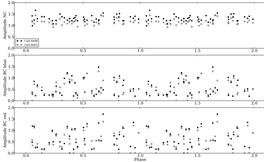
Fig. E.1. Phase-folded curves (using the photospheric absorption line period and phase, which is nearly identical to the He II 4686Å one) for the amplitude of the multi-Gaussian model used to fit the Ca II IR lines. Top: narrow component. Middle: blueshifted BC. Bottom: redshifted BC. There is a marginal amplitude modulation of the BC amplitude.
