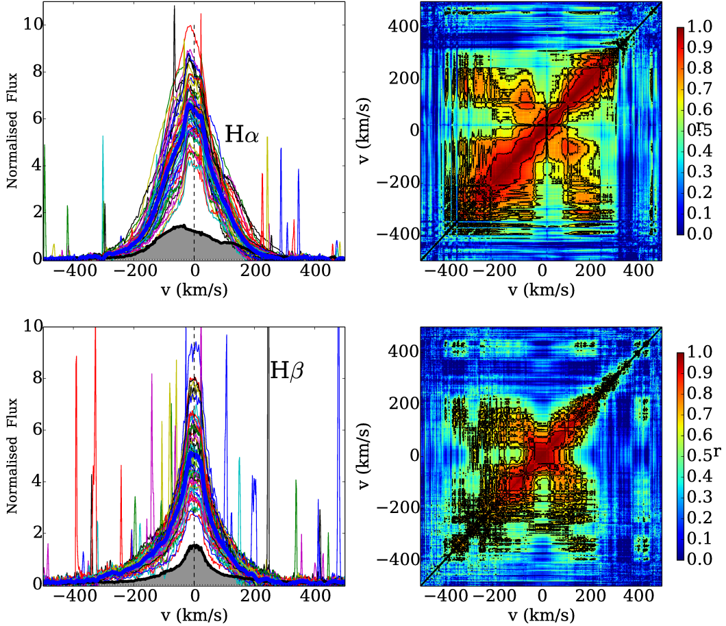
Fig. 1. H\alpha and H\beta line profile variability (left) and autocorrelation matrix (right). The pixel-by-pixel median of the line is shown as a blue thick line. The pixel-by-pixel rms is shown as the thick black line and shaded area. The zero velocities/wavelengths of the lines are marked as dashed vertical lines. The correlation coefficient (estimated as a Spearman rank correlation with value r and false alarm probability p ) is shown on the right in the color scheme, with the black contours marking the high significance ( p > 10^{-5} ) parts with r=0.6, 0.7, 0.8, 0.9 .
