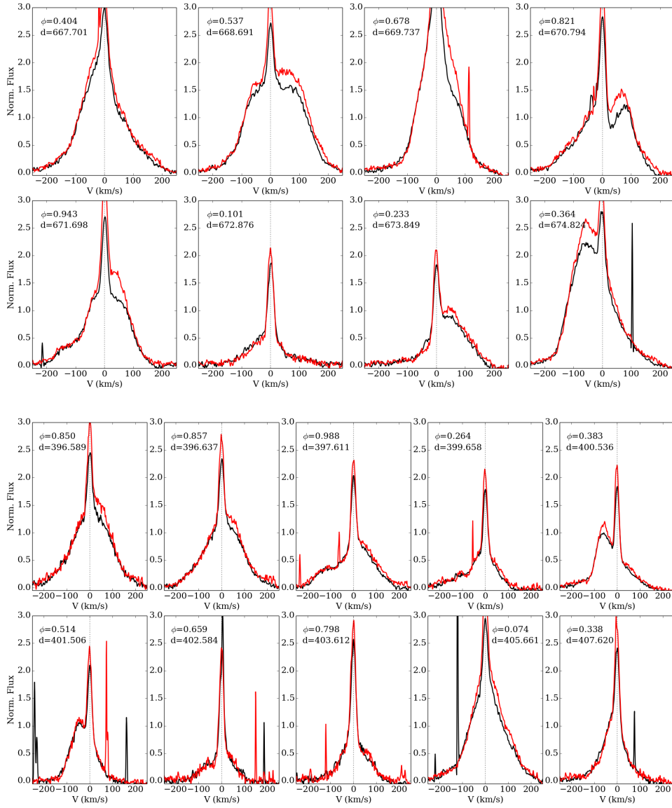
Fig. E.2. Some examples of day-to-day modulation of the BC of the Ca II lines (8498Å line in red, 8662Å line in black). For each set, phase ( \phi ) and date (d=JD-2455000) are given.
