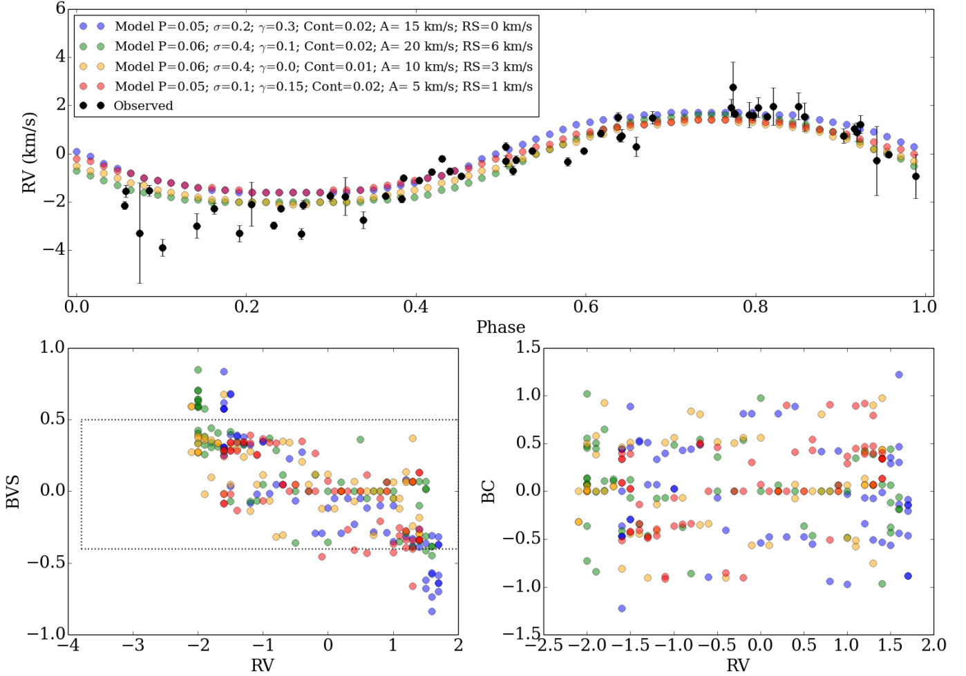
Fig. 9. Results of our toy model for the radial velocity signatures (upper panel), and bisector velocity shift (BVS) and curvature (BC; lower panels). It shows the kind of radial velocity modulations that can be induced on a photospheric absorption line by an emission component (broader than the absorption line) that shows a rotational modulation. 'P' denotes the peak value of an emission component with a Voigt profile with Gaussian width \sigma and Lorentzian contribution \gamma . 'Cont' marks the classical veiling continuum added to the model. 'A' denotes the radial velocity amplitude of the emission line (maximum RV offset for a sinusoidal modulation), and 'RS' is the zero-point redshift of the line. The dashed line box shows the values of the bisector velocity as measured by K14, which are similar to those derived from the toy model. Although there is a slight BVS slope, the typical errors at this level can make it very hard to distinguish.
