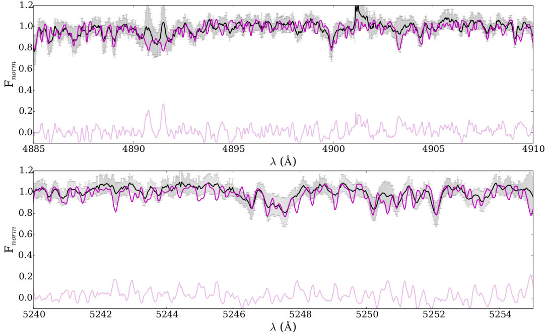
Fig. 10. An example of the attempt to reproduce the median EX Lupi spectrum (black line, with standard deviation per pixel marked in grey) by using a rotationally-broadened standard veiled by a continuum emission (magenta). The difference between the observed and veiled spectra is shown in pink. A constant veiling cannot reproduce the depths of all lines, even if we only consider a very small wavelength range. The differences are too large to be explained by the standard deviation or time variation observed between the different spectra.
