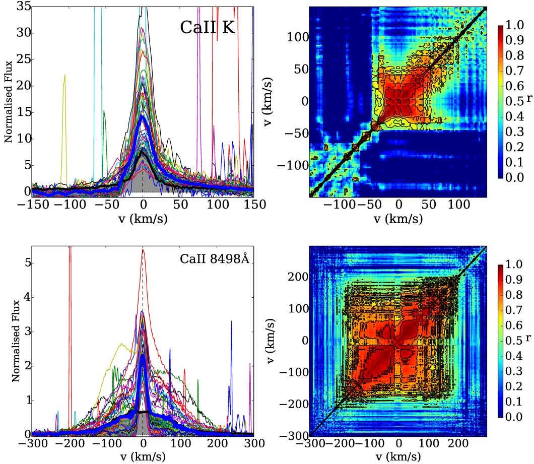
Fig. 2. Same as Figure 1 for the Ca II K (top) and 8498Å (bottom) lines. The pixel-by-pixel median of the line is shown as a blue thick line. The pixel-by-pixel rms is shown as the thick black line and shaded area. The zero velocities/wavelengths of the lines are marked as dashed vertical lines. The correlation coefficient (estimated as a Spearman rank correlation with value r and false alarm probability p ) is shown on the right in the color scheme, with the black contours marking the high significance ( p > 10^{-5} ) parts with r=0.6, 0.7, 0.8, 0.9 .
