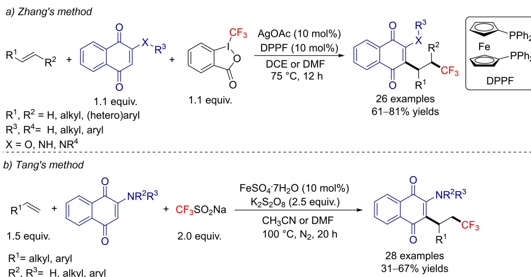
Scheme 20. Intermolecular trifluoromethyl-alkenylation reactions of alkenes with 2-amino- and 2-hydroxy-1,4-naphthoquinone derivatives.
