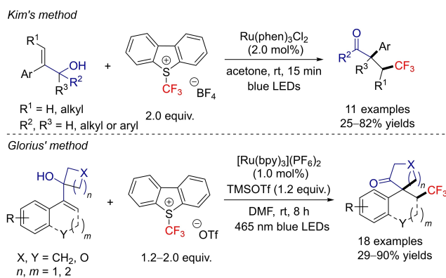
Scheme 52. Photoredox-catalyzed syntheses of trifluoromethylated cyclic ketones with Umemoto's reagent by Kim and Glorius
