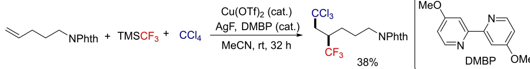
Scheme 39. Copper-catalyzed trifluoromethylation-trichloromethylation of alkene with \text{TMSCF}_3 and \text{CCl}_4 .
