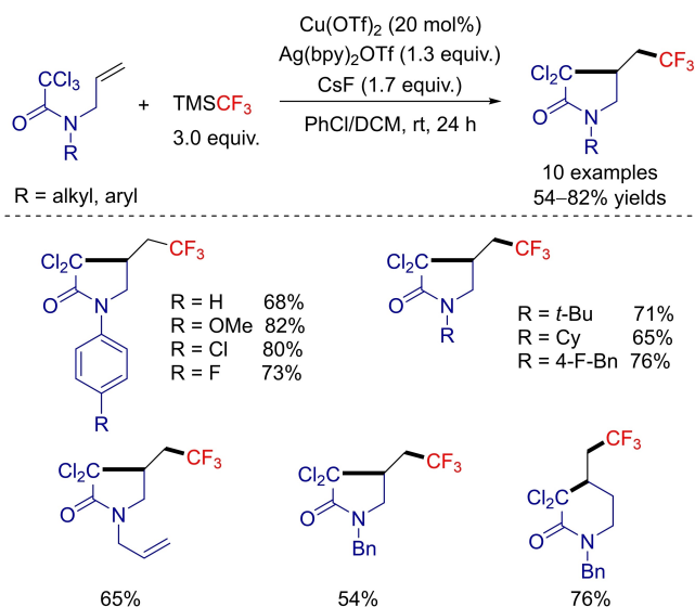
Scheme 31. Copper-catalyzed cyclization-trifluoromethylation of N -substituted N -allyltrichloroacetamides with TMSCF 3 .
