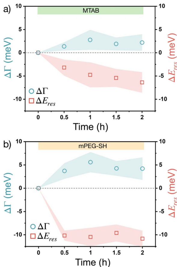
Fig. 4 Localised surface plasmon resonance broadening ( \Delta\Gamma ) and peak shift ( \Delta E_{res} ) of gold nanoprisms obtained by the surface adsorption of different thiol molecules: 10 \mu M MTAB (a) and 100 \mu M mPEG-SH (b).
