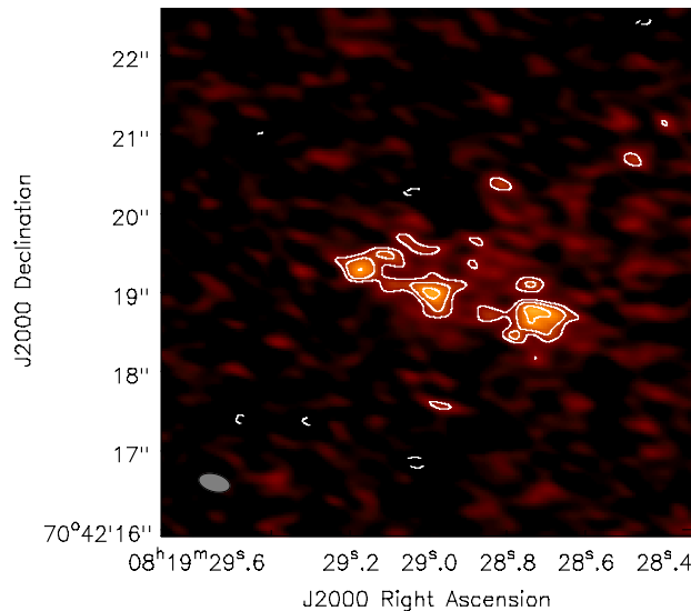
Figure 2. The VLA image of Ho II X-1 in X band, using Briggs robust=1 weighting. The lowest contours start at three times the rms noise level, at \pm 6.6 \mu\text{Jy beam}^{-1} . Contours are increased by factors of \sqrt{2} . The peak brightness is 15 \mu\text{Jy beam}^{-1} . The Gaussian restoring beam size is 0.41'' \times 0.22'' at a major axis position angle of 75^\circ E of N. The background colour image is arbitrarily scaled.
