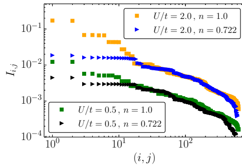
FIG. 6. Two-site mutual information I_{i,j} for the ground state of the 6 \times 6 Hubbard model in momentum space for different U values and different fillings n . The values are sorted in descending order. We include only unique entries of I_{i,j} , i.e., take i > j .
