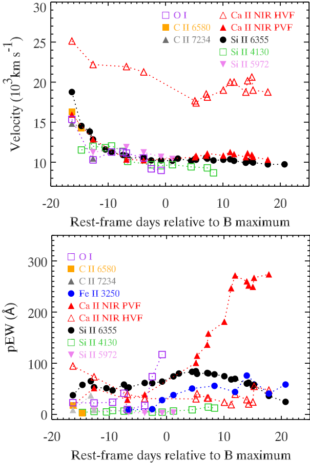
Figure 9. Top: The SN ejecta velocity as a function of phase for various spectral features. Bottom: Same as top panel, but using pEWs instead.
