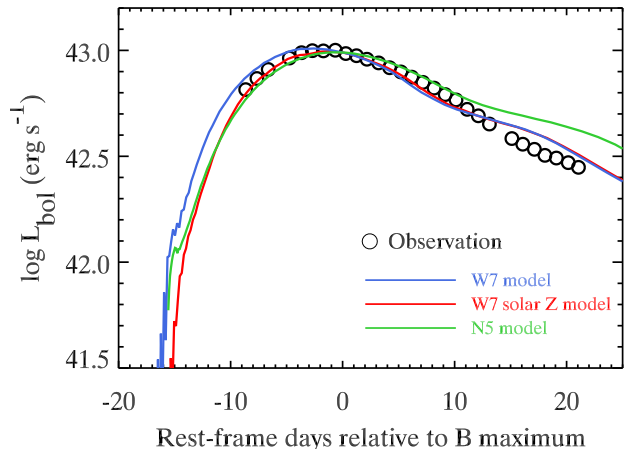
Figure 17. The UVOIR bolometric light curve of SN 2013dy (same as Figure 6) is shown in open circles. We compare the data to model light curves generated from W7 model (blue curve), solar-metallicity polluted W7 Z_{\odot} model (red curve) and the three-dimensional delayed-detonation N5 model (green curve), respectively. Here the model light curve shown for N5 model is angle-averaged. The model light curves are shifted to match the bolometric flux of SN 2013dy at the time of B -band maximum.
