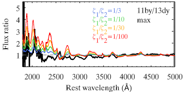
Figure 13. Same as the right panel of Figure 12, but using the flux-ratio spectrum of SN 2011by and SN 2013dy instead.
