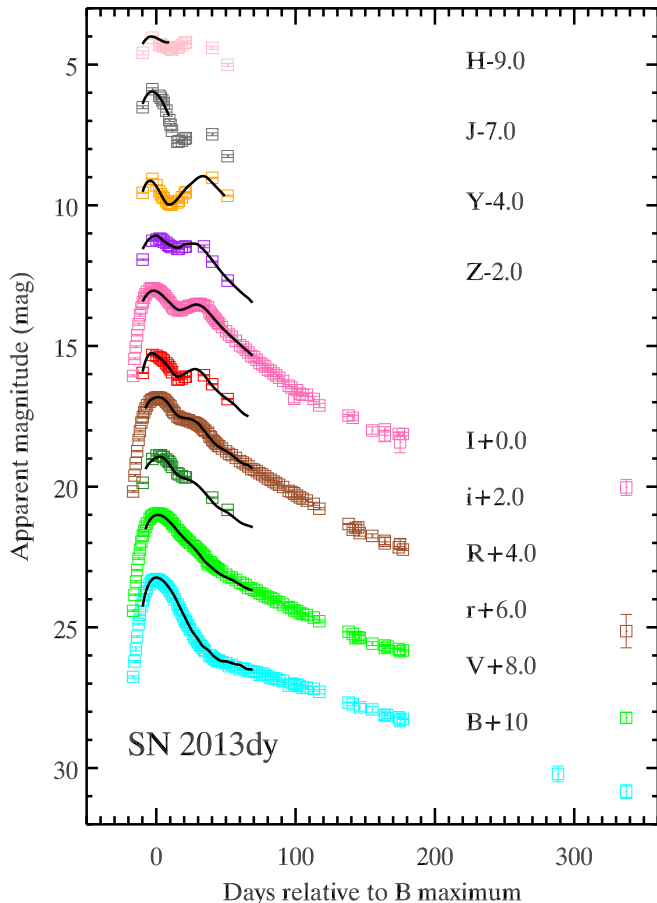
Figure 1. The KAIT BVRI and RATIR riZYJH light curves of SN 2013dy. The solid lines represent the best fit (from SNooPy ) to the observed light curves.
