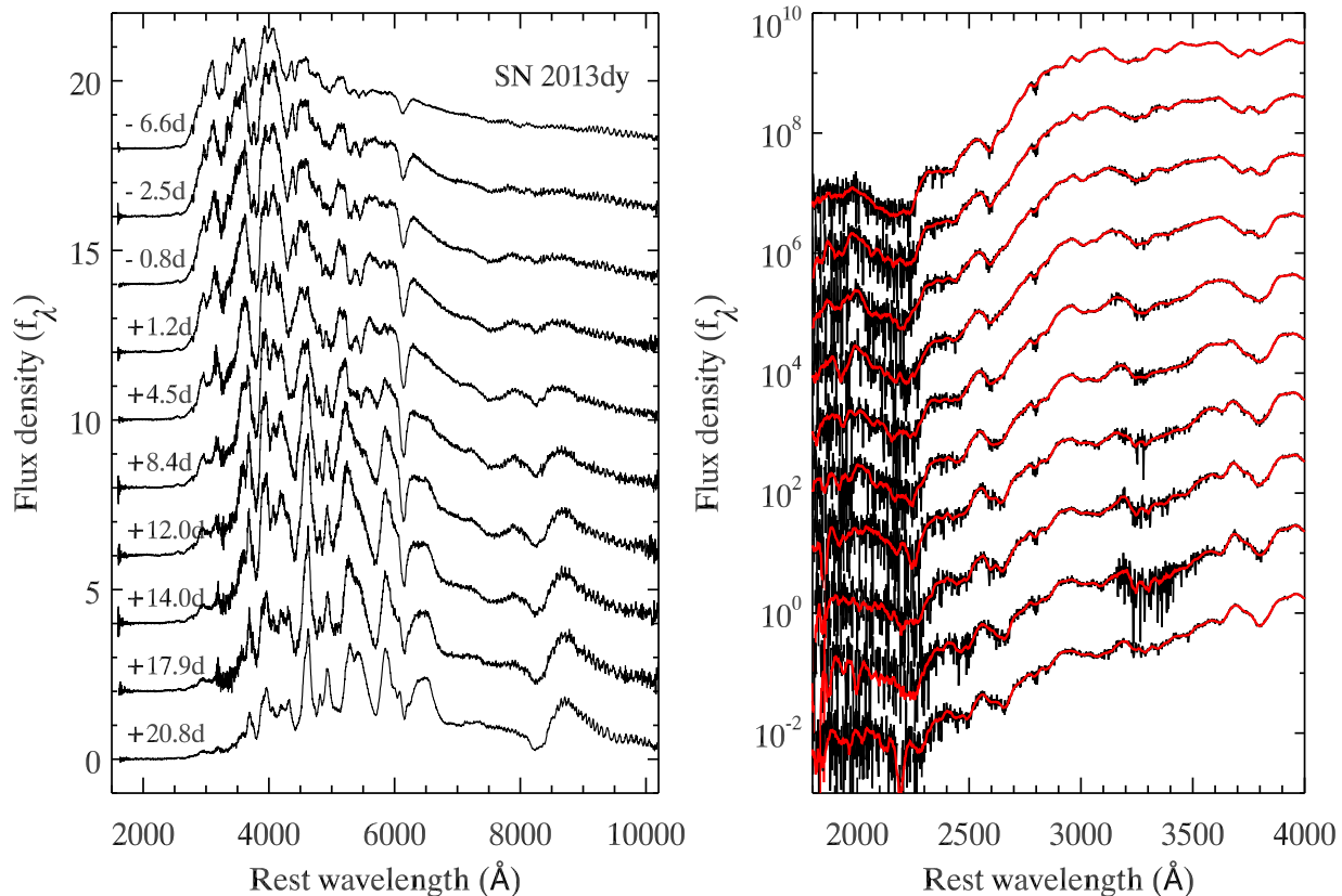
Figure 2. Left: Spectra of SN 2013dy taken with HST /STIS, with arbitrary vertical offsets for clarity. Right: Same as left panel, but a closer look at the UV region. The spectra smoothed with a Savitzky-Golay filter (Savitzky & Golay 1964) are shown in red curves.
