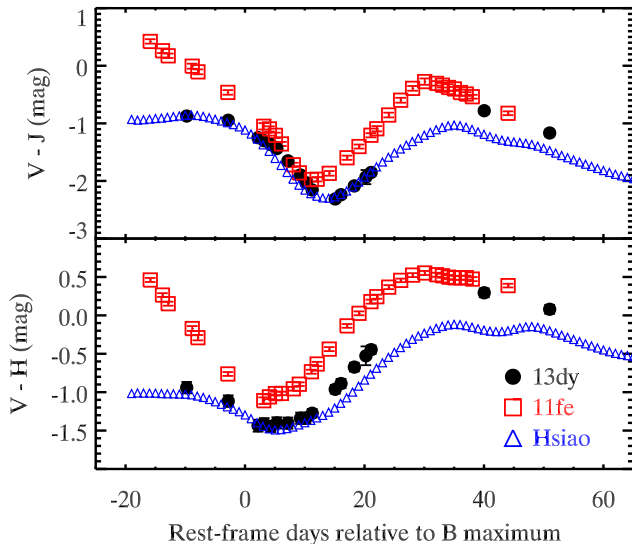
Figure 5. The same as Figure 4, but using V - J and V - H color instead.
