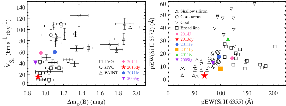
Figure 16. Left: The gradient of Si II \lambda 6355 velocity ( \text{km s}^{-1} \text{day}^{-1} ) as the function of B -band decline rate \Delta m_{15}(B) . The sample and subclasses studied in Benetti et al. (2005) is overplotted. The sample is split into three different subclasses: ‘low-velocity gradient’ (LVG; open squares), ‘high-velocity gradient’ (HVG; open circles) and ‘FAINT’ (open triangles). Right: Si II \lambda 5972 pEW as the function of Si II \lambda 6355 pEW. The sample and subclasses studied in Branch et al. (2009) is overplotted. The sample is split into four different subclasses: ‘shallow silicon’ (open triangles), ‘core normal’ (open circles), ‘cool’ (open downward triangles) and ‘broad line’ (open squares). The position of SN 2013dy is represented by the red filled star. We also mark the positions of a variety of SNe Ia for comparison.
