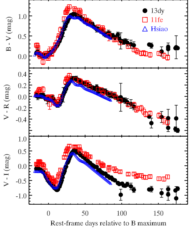
Figure 4. The color curves of SN 2013dy. From top to bottom: The B - V , V - R , and V - I color as a function of phase. The filled circles are the data in this work. The color curves from SN 2011fe (red open squares) and the Hsiao et al. (2007) templates (blue open triangles) are compared.
