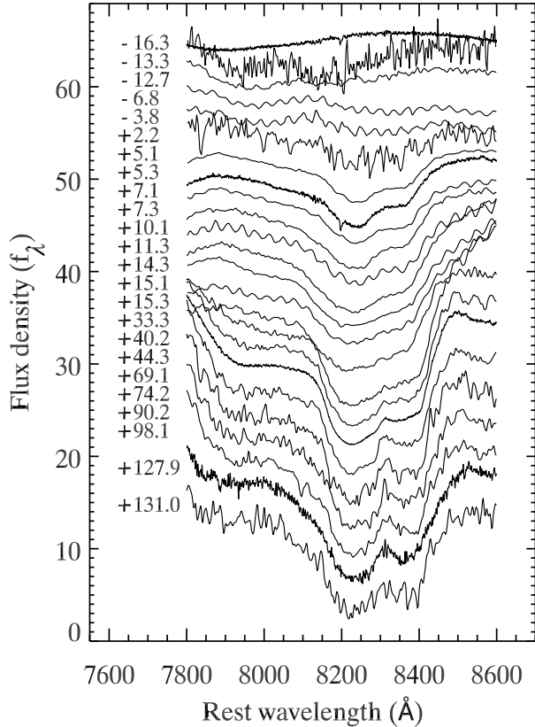
Figure 10. The evolution of the Ca II NIR triplet with phase.
