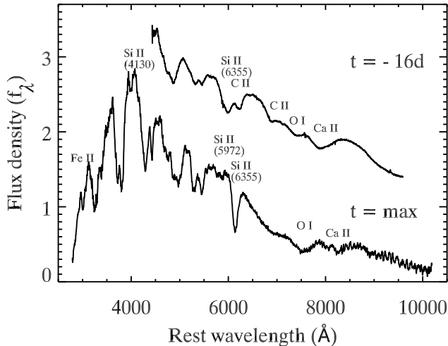
Figure 7. Spectra at t = -16 d and +0 d demonstrating the key spectral features measured in this work.
