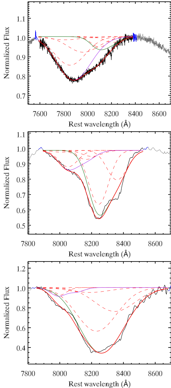
Figure 8. From top to bottom: The Ca II NIR absorption at -16 , +5 and +15 days, respectively. The black curve shows the range we fit the line profile. The blue continuum regions near the left and right side of the line profile are the regions we select to fit the pseudo-continuum. The red solid line is the best fit to the line profile, which is the superposition of all the line components used for the fitting (represented in dashed lines). The green curve represents the superposition of all the components in Ca II NIR photospheric-velocity feature (PVF). The purple curve represents the superposition of all the components in the Ca II NIR high-velocity feature (HVF).
