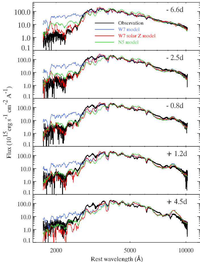
Figure 18. The HST spectra at different epochs (black curves). We compare the data to model spectra generated from W7 model (blue curves), solar-metallicity polluted W7 Z_{\odot} model (red curves) and the three-dimensional delayed-detonation N5 model (green curves), respectively. The model spectra are scaled with the same multiplicative factor used to shift the model bolometric light curve in Figure 17.
