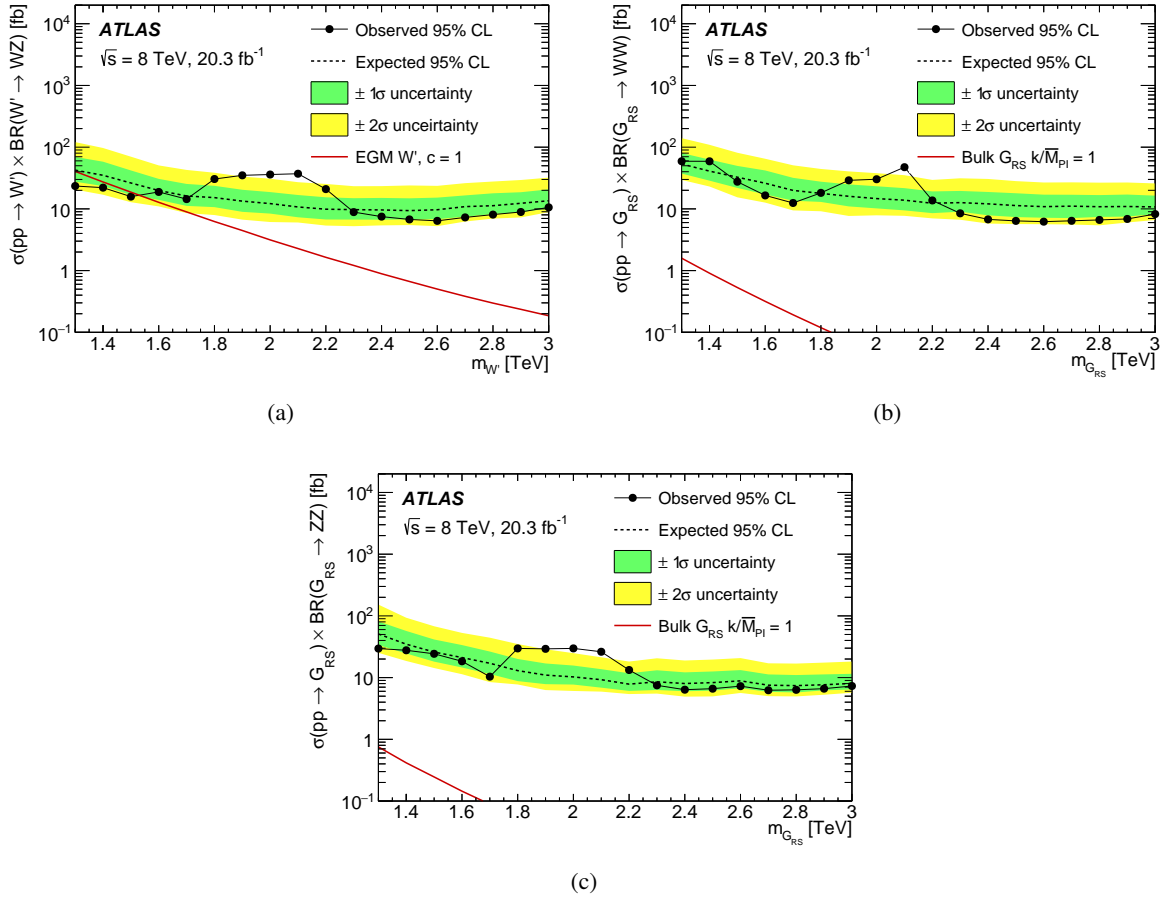
Figure 6: Upper limits, at 95% C.L., on the section times branching ratio limits for the WZ window selection as a function of m_W , and for the WW window selection and the ZZ window selections as a function of m_{G_{RS}} . The solid red line in each figure displays the predicted cross section for the W' or G_{RS} model as a function of the resonance mass.
