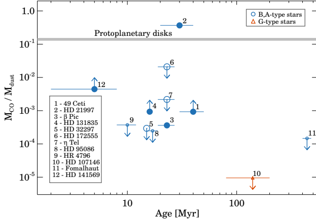
Figure 8. CO to dust mass ratio as a function of age for debris disks and for HD 141569. Debris disks with known gas component are marked by larger symbols, those where CO gas was detected are shown by filled symbols. Their CO /dust mass data and ages were taken from Table 4 and 5. HD 32297 was placed at its lower age limit proposed by Rodigas et al. (2014). For Fomalhaut and HD 107146 we used data from the literature (Matrà et al. 2015; Ricci et al. 2015, and references therein), in the latter case the CO upper mass estimate derived from the secondary disk scenario were taken into account. In the case of HD 141569 and HR 4796 the CO mass and upper limit were computed by adopting an excitation temperature of 20 K and using the CO (3–2) line fluxes from Dent et al. (2005); Hales et al. (2014). Their dust masses were computed from their submillimeter fluxes (Sheret et al. 2004) using the standard way. Age estimate of HD 141569 was taken from Weinberger et al. (2000). As a member of the TW Hya association, for HR 4796 we applied the age of the group (Torres et al. 2008; Gagné et al. 2014). The data of HD 95086 are from Table 1 and Moór et al. (2015). The typical M_{CO}/M_{dust} ratio for protoplanetary disks (horizontal line) was calculated by assuming a total gas to dust mass ratio of 100 and taking a canonical CO to H_2 abundance ratio of 10^{-4} .
