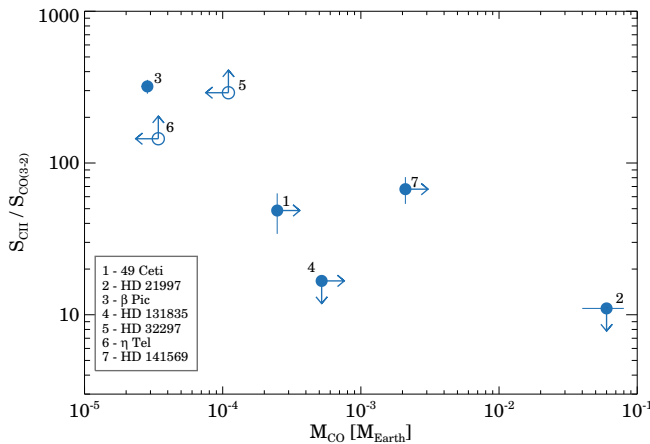
Figure 9. S_{CII}/S_{CO(3-2)} ratio as a function of total CO mass for gaseous debris disks (apart from HD 172555 where neither of CO , nor C II were detected) and HD 141569. C II line flux data for HD 131835 and HD 21997 were taken from Sect 2.3.1 and from Juhász et al. (in prep.) For the other targets S_{CII} values were from 49 Ceti – Roberge et al. (2013); \beta Pic – Cataldi et al. (2014); HD 32297 – Donaldson et al. (2013); \eta Tel – Riviere-Marichalar et al. (2014); HD 141569 – Meeus et al. (2012). References for the S_{CO(3-2)} data are summarized in Fig. 7 caption.
