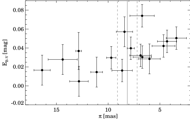
Figure 3. Derived reddening values as a function of trigonometric parallaxes taken from the Hipparcos catalogue for 16 stars located within 3^\circ from HD 131835. The solid and dashed vertical lines show the measured parallax and its uncertainty for HD 131835.
