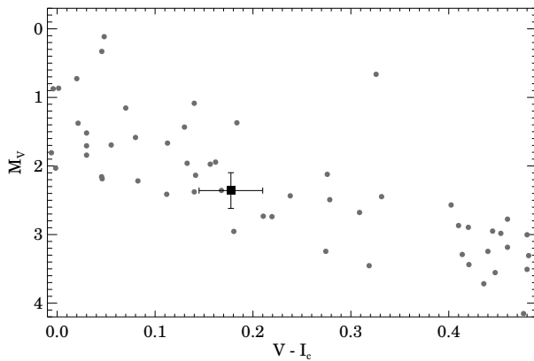
Figure 4. Absolute V band magnitude versus V-I_c color indices for known members of UCL (the member list was taken from de Zeeuw et al. 1999) located within 150 pc and having parallax error <10\% (gray dots) and for HD 131835 (black square). Photometric data were taken from the Hipparcos catalog and dereddened using extinction values from Chen et al. (2011, 2012) and, for HD 131835, based on our result.
