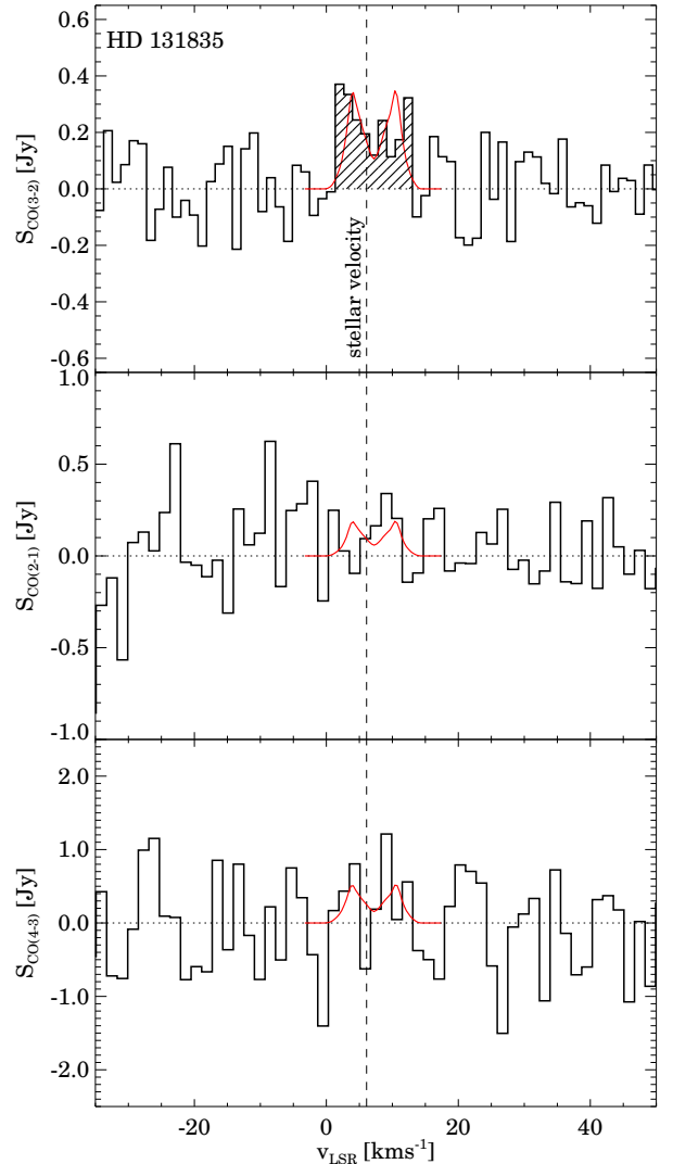
Figure 1. APEX CO(3–2), CO(2–1), and CO(4–3) spectra of HD 131835. The dashed line marks the radial velocity of the star. In the upper panel the hatched area shows the part of the spectrum considered in the line flux integration (Sect. 2.2). The best fit model spectra (see Sect. 3.3) are plotted by red lines.
