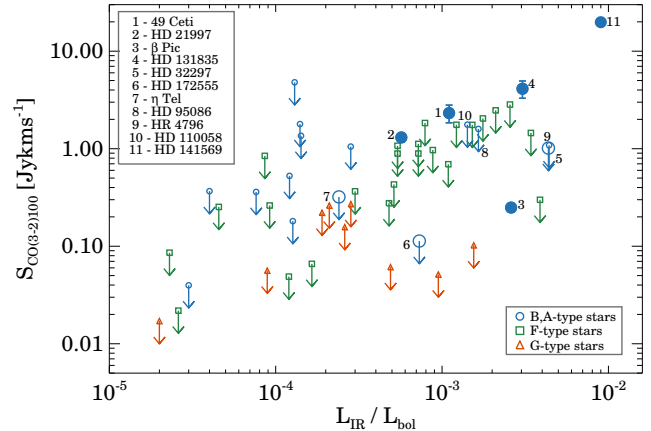
Figure 7. Integrated CO(3–2) fluxes or upper limits for debris disks and the transitional disk around HD 141569 normalized to 100 pc are plotted against fractional luminosities. Fractional luminosities and integrated line fluxes for the annotated sources were taken from: 49 Ceti – Moór et al. (2015), Dent et al. (2005); HD 21997 – Moór et al. (2015), Kóspál et al. (2013); \beta Pic – Rhee et al. (2007), Dent et al. (2014); HD 32297 – Chen et al. (2014), Moór et al. (2011a); HD 172555 – Riviere-Marichalar et al. (2012), Moór et al. (2011a); HR 4796 – Chen et al. (2014), Greaves et al. (2000); HD 110058 – Chen et al. (2014), Moór et al. (2011a); HD 141569 – Meeus et al. (2012), Dent et al. (2005); HD 131835, \eta Tel, HD 95086 – Table 1. For the rest of the objects the data are from Ballering et al. (2013); Chen et al. (2005, 2014); Dent et al. (2005); Fajardo-Acosta et al. (1998); Hales et al. (2014); Moór et al. (2011b,a, 2015); Najita & Williams (2005); Patel et al. (2014); Pascucci et al. (2006); Rhee et al. (2007). Disks with known gas component are denoted by larger symbols.
