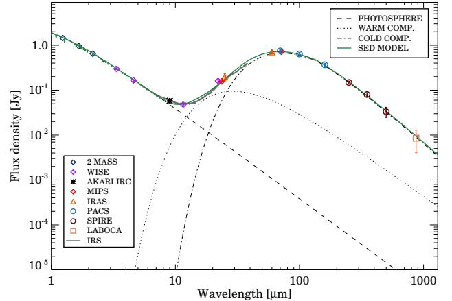
Figure 5. Color corrected SED of HD 131835 overplotted by the fitted simple two-component model.
