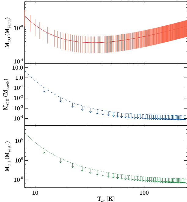
Figure 6. Gas mass versus excitation temperature for CO, C II, and O I in HD 131835, assuming optically thin gas emission. For C II and O I the plotted values are upper limits.
