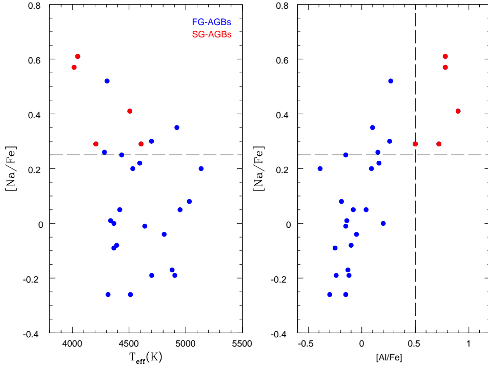
Fig. 3.— Literature [Na/Fe] abundances (corrected for NLTE) for our APOGEE sample of FG- and SG-AGB stars (blue and red dots, respectively) shown against stellar effective temperature T_{\text{eff}} (left panel) and Al abundances (right panel). The horizontal and vertical lines mark [Na/Fe]=+0.25 dex and [Al/Fe] = +0.50 dex, respectively and separate the FG-AGBs from the SG ones. The Na limit is set to [Na/Fe] = 0.25 dex, corresponding to the average upper limit for the [Na/Fe] value for FG field stars in the metallicity range covered by the GCs in our sample (see e.g., Carretta 2013).
