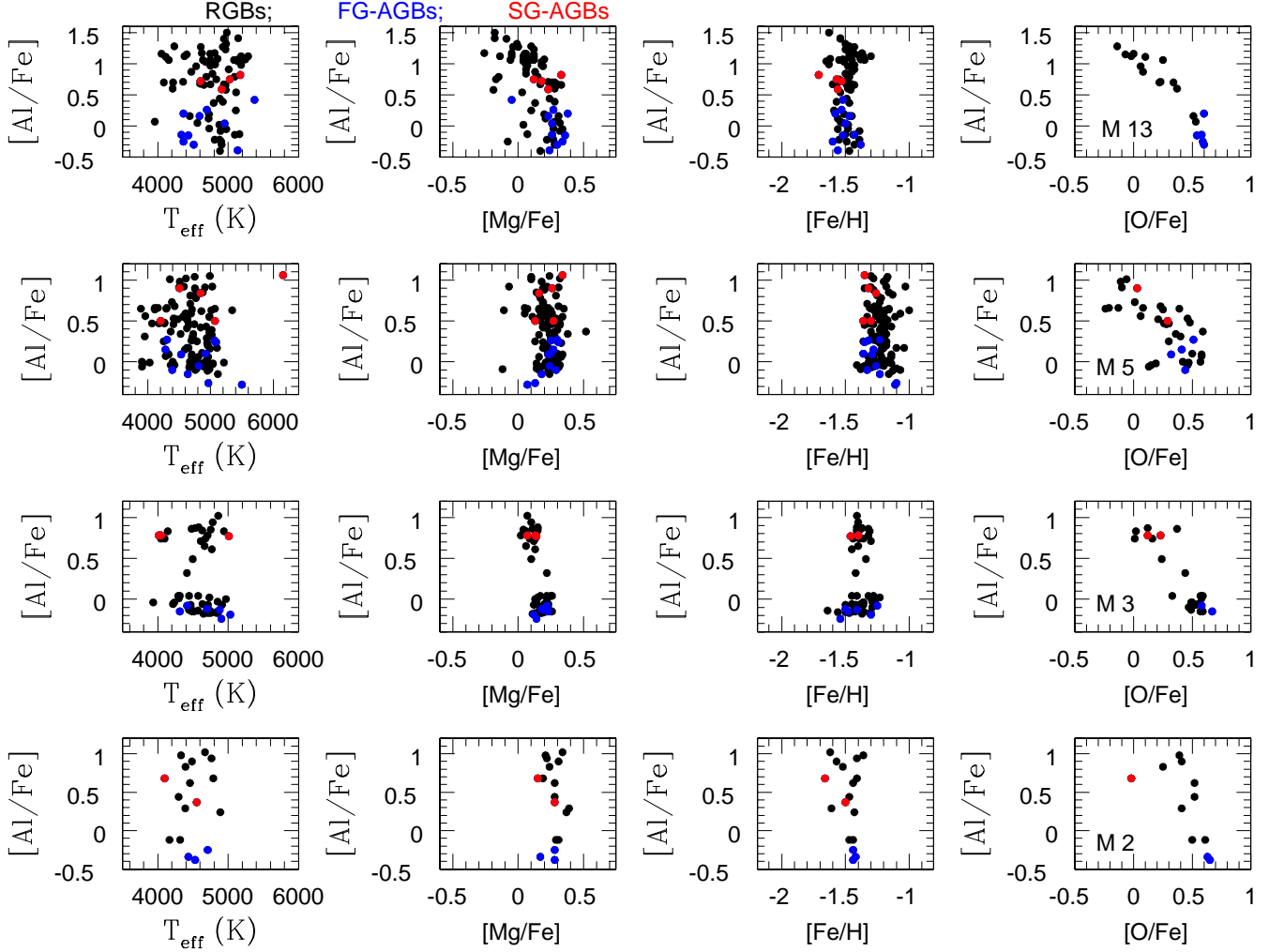
Fig. 2.— [\text{Al}/\text{Fe}] for our APOGEE sample of FG- and SG-AGB stars (blue and red dots, respectively) in metal-poor GC stars (from top to bottom: M 13, M 5, M3, and M 2) shown against (from left to right) stellar effective temperature T_{\text{eff}} , [\text{Mg}/\text{Fe}] , [\text{Fe}/\text{H}] , and [\text{O}/\text{Fe}] . The APOGEE abundances are precise to the \sim 0.1 dex level. For comparison, the RGB stars (black dots) observed by APOGEE are also displayed. Note that the spread in [\text{Fe}/\text{H}] is bigger in RGB than in AGB stars because of the presence of warm stars, which lead to bigger uncertainties (consequently [\text{Al}/\text{Fe}] is determined with higher accuracy in AGB than in RGB stars).
