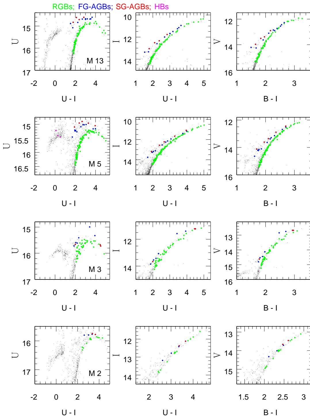
Fig. 1.— Color-magnitude (CMD) diagrams U vs. (U - I) (left panels), I vs. (U - I) (middle panels), and V vs. (B - I) (right panels) for metal-poor GCs (from top to bottom: M 13, M 5, M 3, and M 2). Ground-based photometry for the cluster stars is indicated with black dots, while the RGB, FG-AGB, and SG-AGB stars observed by APOGEE are indicated with green, blue, and red dots, respectively. The three M 5 stars marked with magenta dots (left panel) are HB stars.
