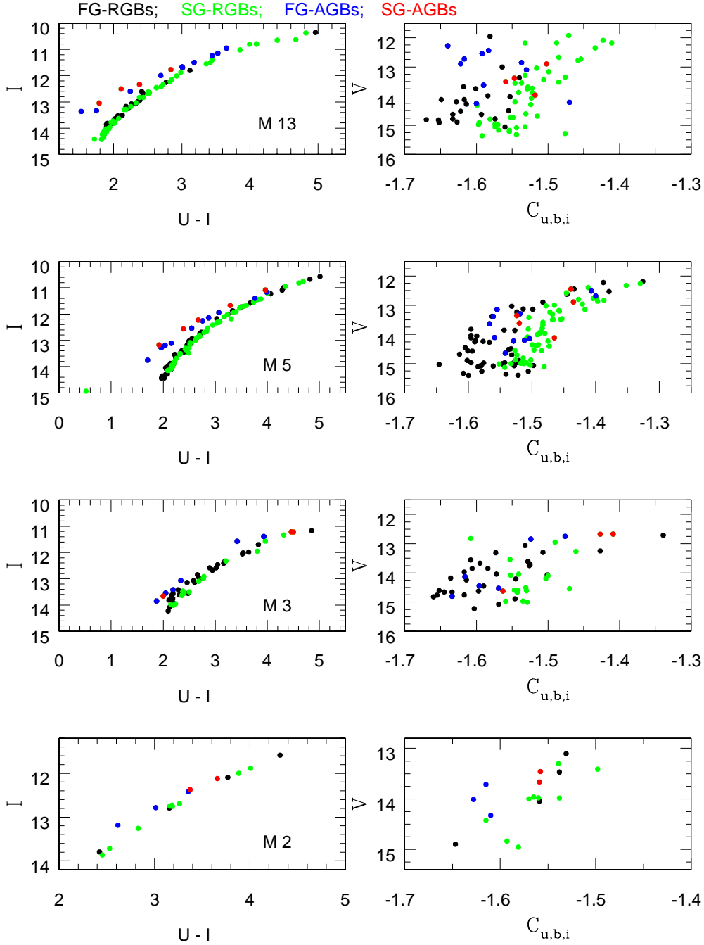
Fig. 4.— Color-magnitude (CMD) diagrams I vs. (U - I) (left panels) and the (V, C_{u,b,i}) pseudo-CMDs (right panel) for the metal-poor GCs (from top to bottom: M 13, M 5, M 3, and M 2) observed by APOGEE. FG- and SG-AGB stars are marked (blue and red dots, respectively). For comparison, the FG- and SG-RGB stars (black and green dots, respectively) are also displayed.
