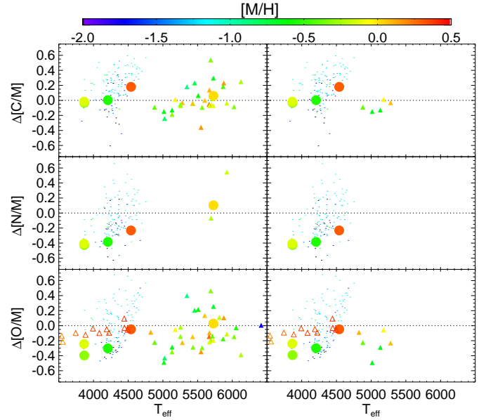
Figure 8. Same as Figure 7 for CNO abundances.
