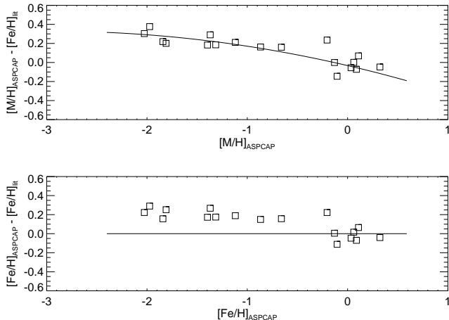
Figure 6. External elemental abundance calibration.
