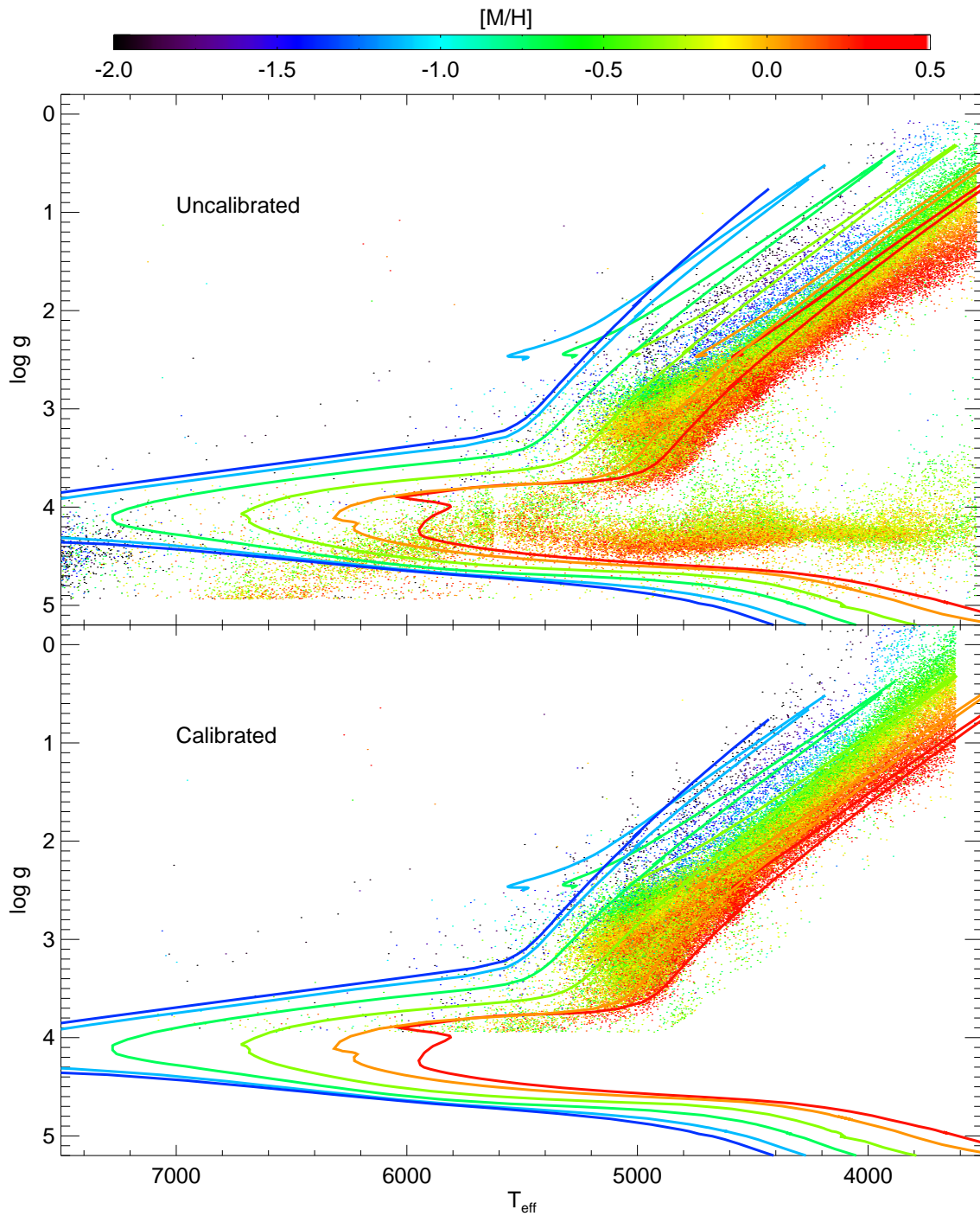
Figure 12. Effective temperature - surface gravity - metallicity distributions for uncalibrated full APOGEE sample (top) and for calibrated giant sample (bottom). Isochrones from Bressan et al. (2012) for a 4 Gyr population are overlaid.
