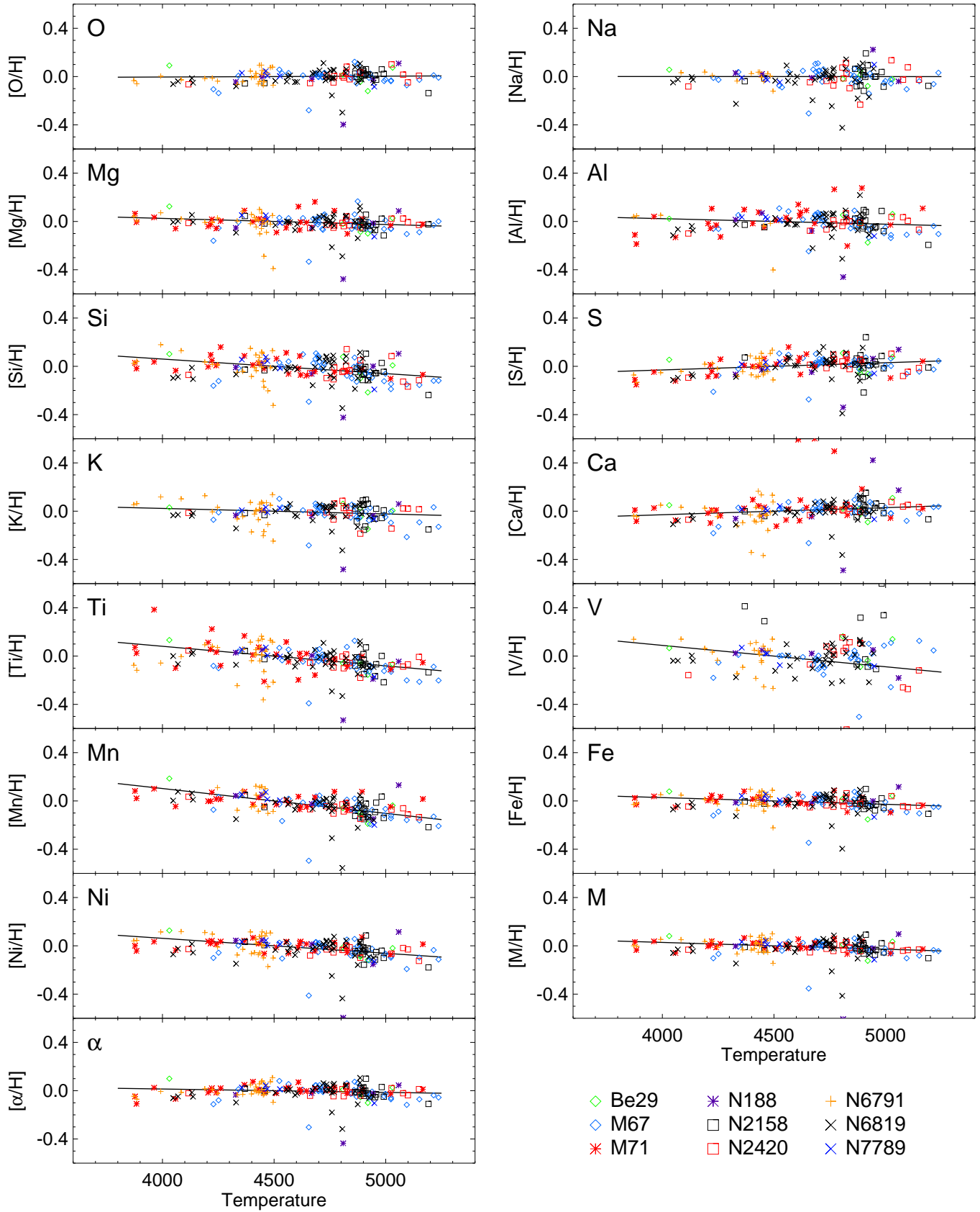
Figure 5. Internal elemental abundance calibrations. Plots show deviations of individual elements relative to the cluster means as a function of temperature; different symbols are for different clusters, as noted in lower right. Lines show the adopted temperature calibrations. Carbon and nitrogen are not shown because we cannot assume homogeneous abundances within clusters.
