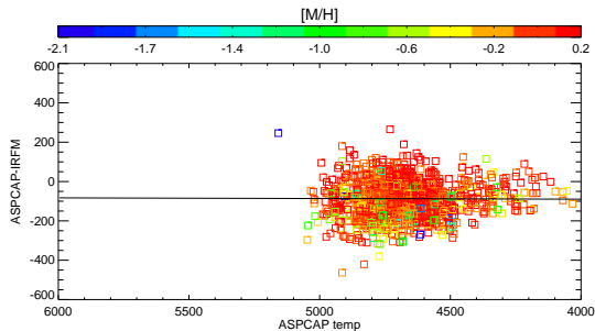
Figure 3. Temperature calibration, derived from low-reddening sample with photometric temperatures.
