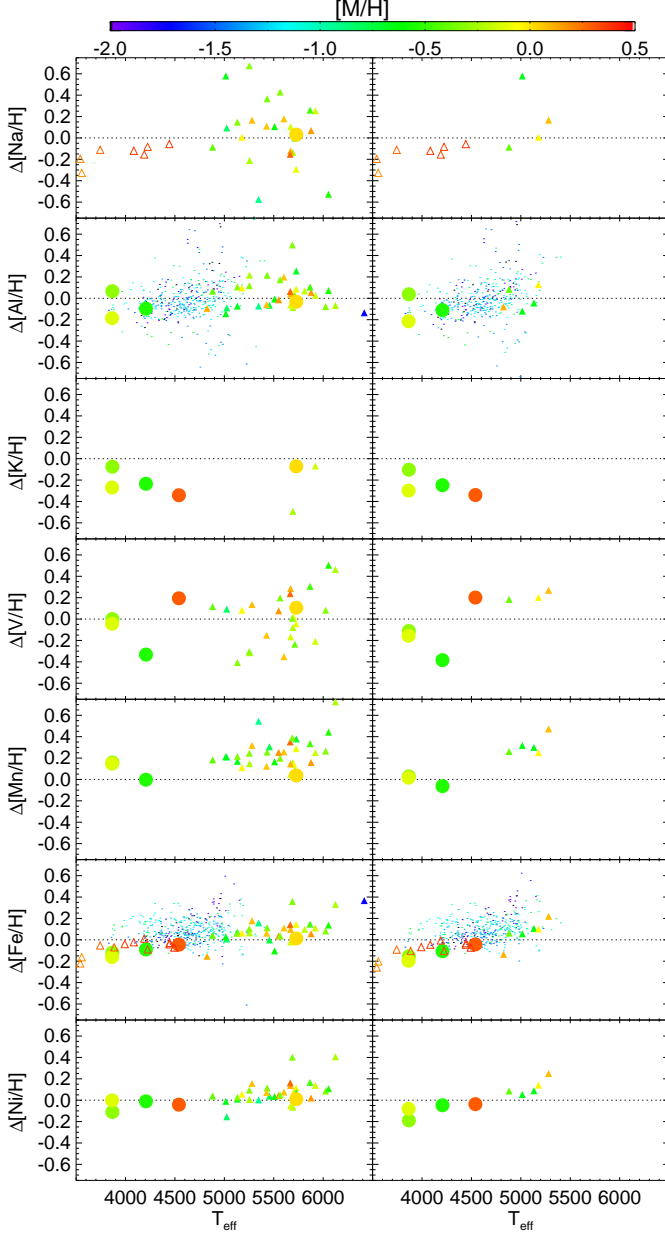
Figure 10. Same as Figure 7 for Na, Al, K, V, Mn, Fe, and Ni. with the line list, will be amplified at cooler temperatures.
