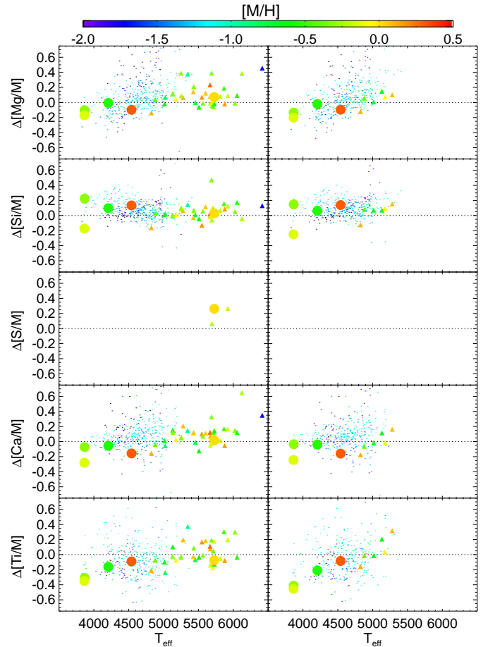
Figure 9. Same as Figure 7 for \alpha -element abundances (Mg, Si, S, Ca, Ti).
