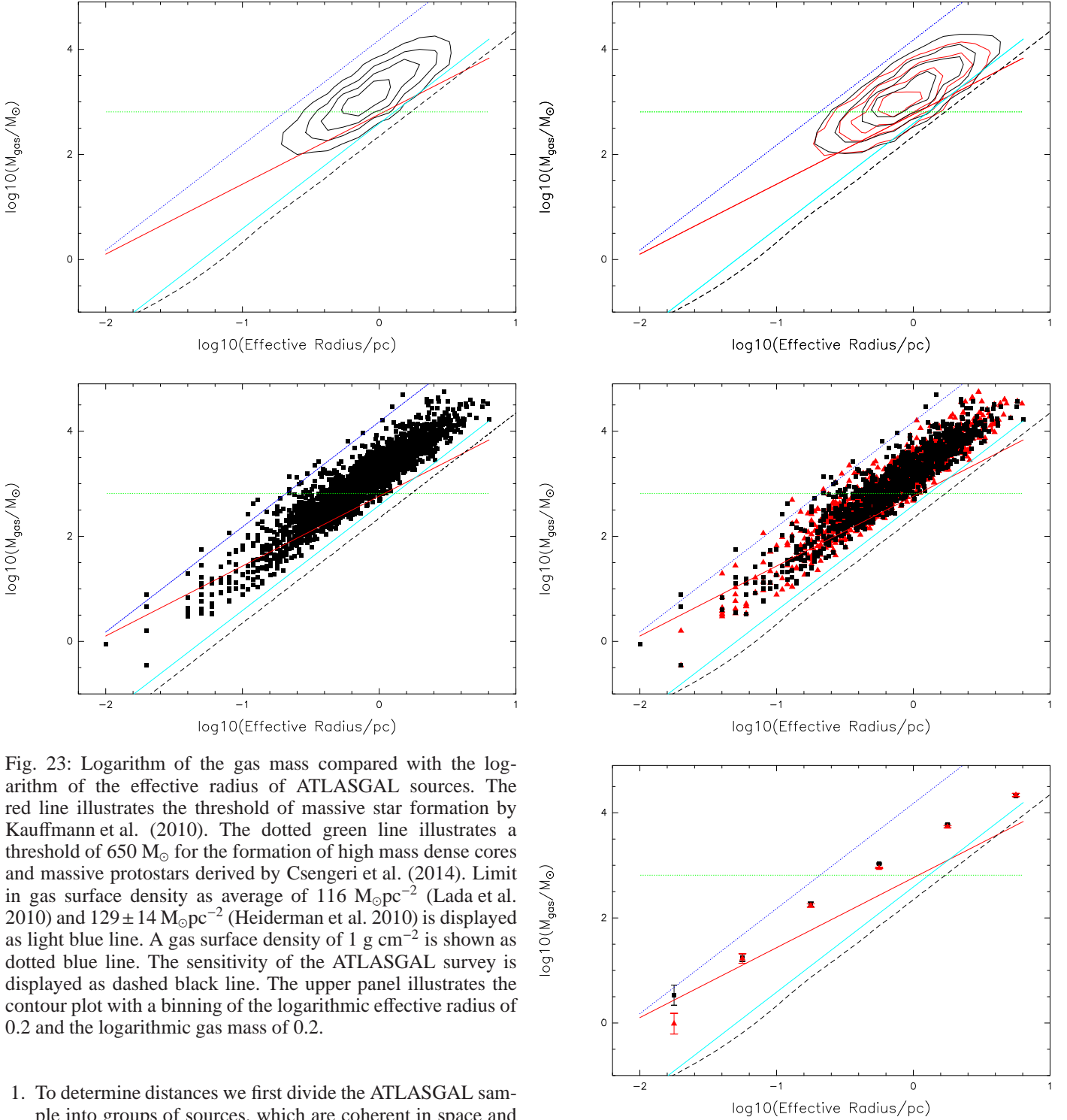
Fig. 24: The mass-size relation for a cold and a warm ATLASGAL subsample (see Sect. 7.5) is shown as a red and black contour plot in the top panel, bins of 0.25 are used for the logarithm of the effective radius and bins of 0.2 for the logarithm of the gas mass. The scatter plot with the cold subsample as red triangles and the warm sources as black points is displayed in the middle panel. Mean values of the logarithm of the gas masses and of the effective radii are plotted in the bottom panel. The lines are the same as described in Sect. 7.5.
