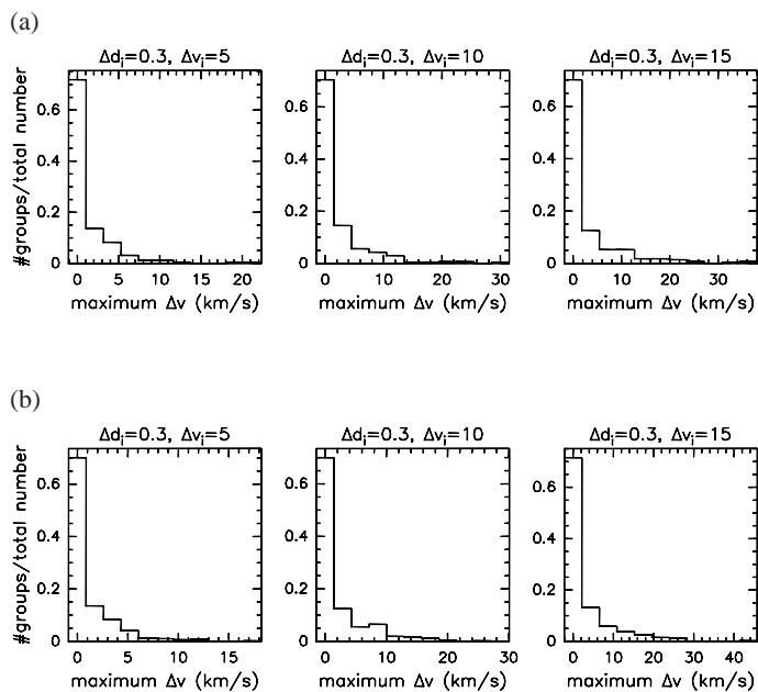
Fig. A.2: Relative number distribution of ATLASGAL groups in the first quadrant in panel a ) and groups in the fourth quadrant in panel b ) with the maximum velocity difference in a group for different input values of the velocity interval to search for associated sources in a group, \Delta v_i . We use 5 to 15 km s -1 for that and a fixed maximum distance between individual sources in a group, \Delta d_i , of 0.3°.
