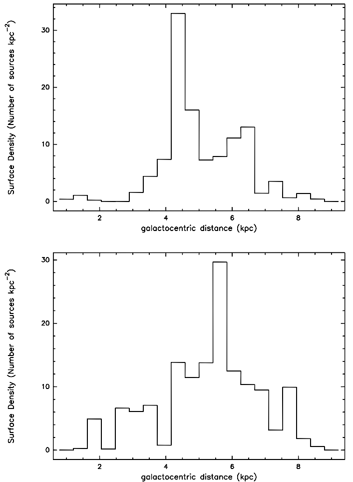
Fig. 6: Number distribution of ATLASGAL sources with galactocentric radii, the clumps in the first quadrant are plotted at the top and the sources in the fourth quadrant at the bottom.
