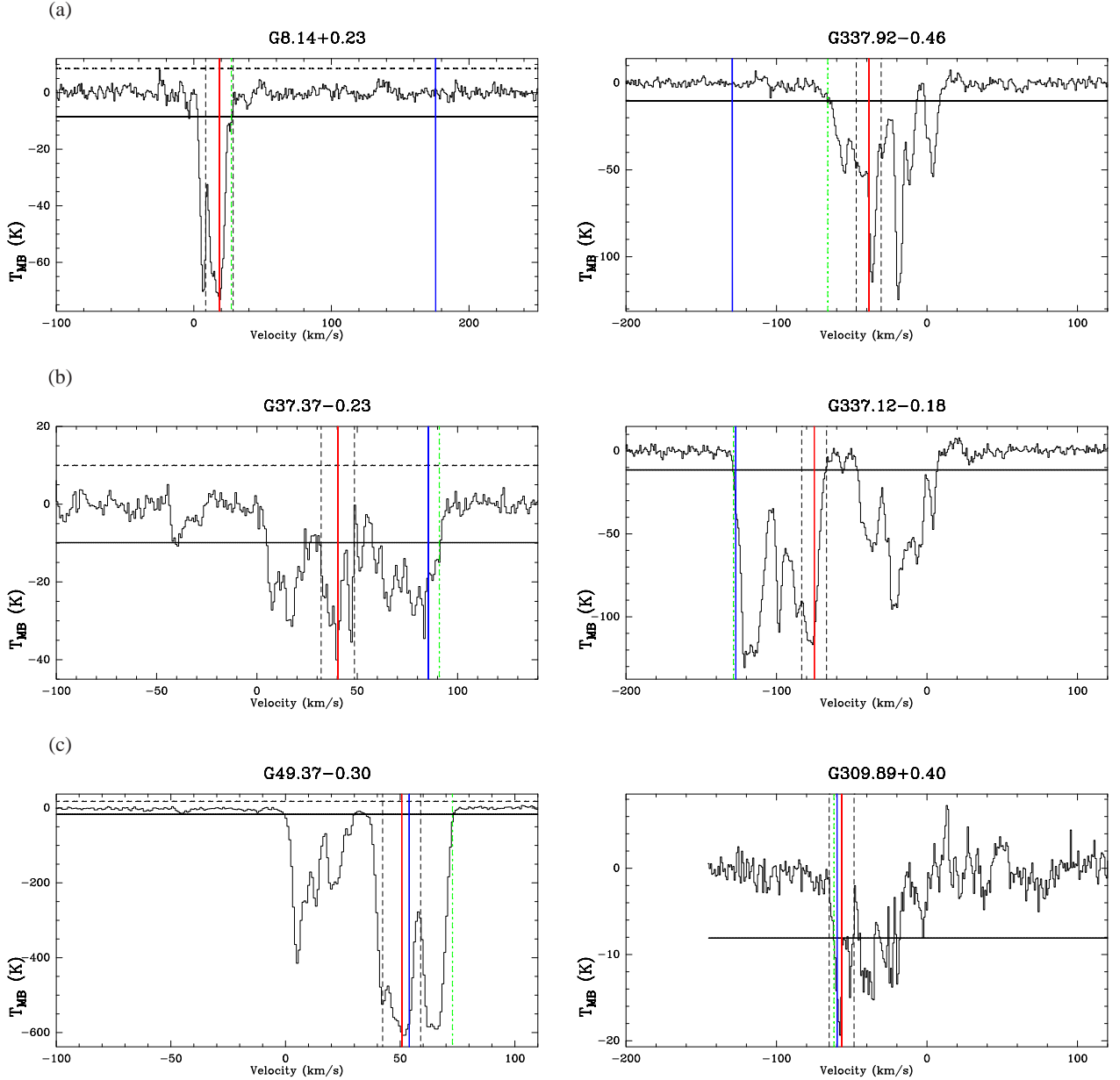
Fig. 3: Example of HI spectra towards HII regions in the first and fourth quadrant extracted from 21 cm line cubes from the VGPS and SGPS. The source velocity is illustrated as solid red vertical line, the tangent point velocity as solid blue vertical line, and the velocity, at which the absorption is below 5\sigma , as dashed-dotted green vertical line. This limit of -5\sigma is indicated by the solid black horizontal line. In addition, the maximum positive intensity of HII regions in the first quadrant must be lower than 5\sigma , which is shown as dashed black horizontal line. The dashed black vertical lines \pm 8.28 \text{ km s}^{-1} around the source velocity display its variation because of the velocity dispersion of clouds and streaming motions (see Sect. 5.4). Examples of sources in the first quadrant are shown on the left and of clumps in the fourth quadrant on the right. a) There is a large difference between the tangent point velocity and the velocity, up to which HI absorption is seen and which is close to the source velocity for G8.14+0.23 and G337.92-0.46, which are thus located at the near distance. They are located in the diagonal right region in Fig. 4 (red points) confined by the amount of streaming motions. b) Our analysis reveals HI absorption at velocities close to the tangent point velocity for G37.37-0.23 and G337.12-0.18, which are assigned to the far distance and indicated as blue points in the horizontal right part in Fig. 4. c) We locate G49.37-0.30 and G309.89+0.40 at the tangent point because the source velocity is within 8.28 \text{ km s}^{-1} around the tangent point velocity. They are displayed as purple points in Fig. 4.
