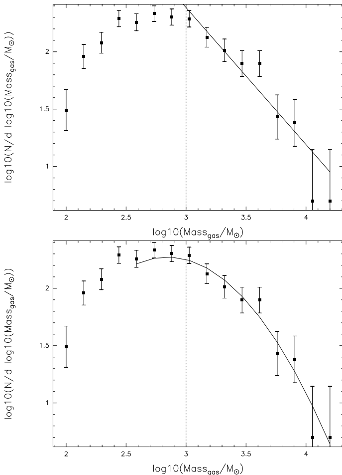
Fig. 12: Differential clump mass function of ATLASGAL sources with distances from 2 to 5 kpc fitted to masses above 1000 M_{\odot} in the upper panel yields a power-law exponent of -2.19 \pm 0.11 . The vertical line displays the completeness limit of 1000 M_{\odot} . A lognormal function is fitted to the mass distribution of this ATLASGAL subsample resulting in A = 188 , M_{\text{peak}} = 700 M_{\odot} , and \sigma = 0.49 . M_{\text{peak}} is below the completeness limit and the peak itself is thus not well constrained.
