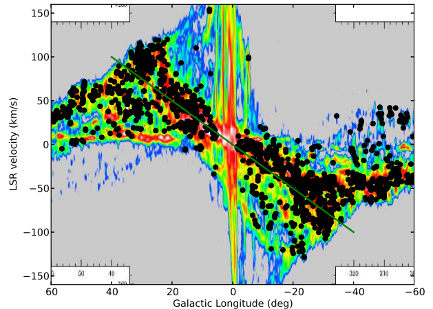
Fig. 1: Galactic longitudes of ATLASGAL sources are compared with the radial velocities with CO (1–0) emission in the background (Dame et al. 2001). The green line indicates the 5 kpc molecular ring (Simon et al. 2006).
