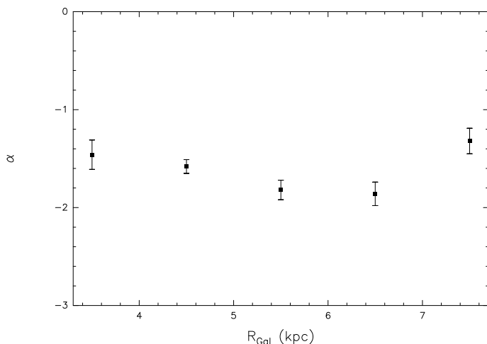
Fig. 22: Fitting of the differential mass distributions of ATLASGAL clumps above 1000 M_{\odot} within 1 kpc over the range of galactocentric radii from 3 to 8 kpc gives similar power-law exponents, \alpha . There is a slightly decreasing slope of \alpha with increasing galactocentric radius out to \sim 7 kpc and an increasing slope to \alpha = -1.3 at 8 kpc.
