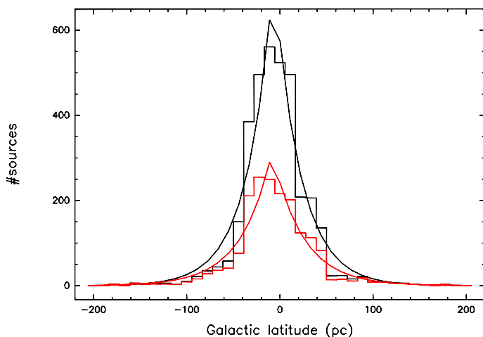
Fig. 7: Number distribution of ATLASGAL subsamples in the first and fourth quadrant with the height above Galactic plane is plotted in black. The histogram of sources with masses above the completeness limit of 1000 M_\odot is shown in red.
