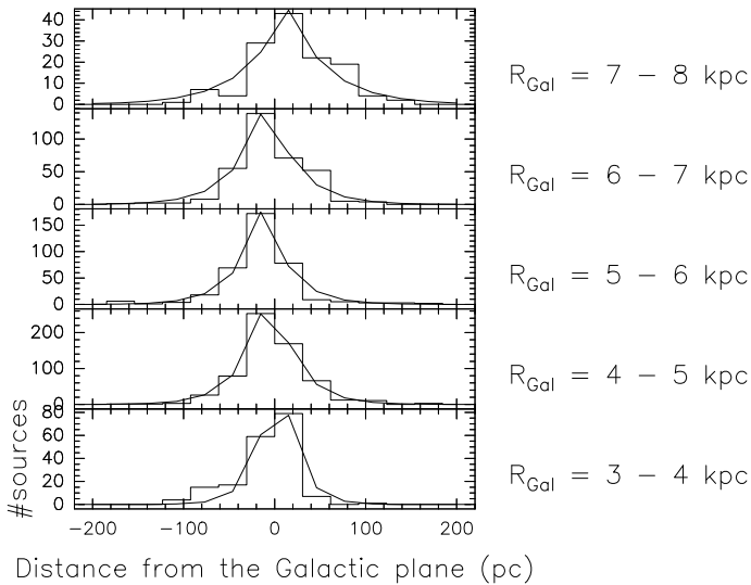
Fig. 16: Histograms of the height above Galactic plane for every bin in galactocentric radius of the subsamples in the first and fourth quadrant. The distributions are fitted by an exponential.
