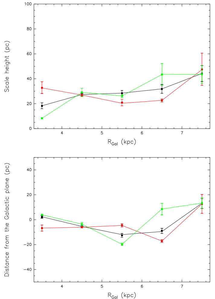
Fig. 17: Dependence of scale height on the galactocentric radius in the top panel and the distance from the disk of the Milky Way shown against galactocentric radii in the lower panel. The subsample in the first quadrant is indicated in red, sources in the fourth quadrant in green, and the two combined in black.
