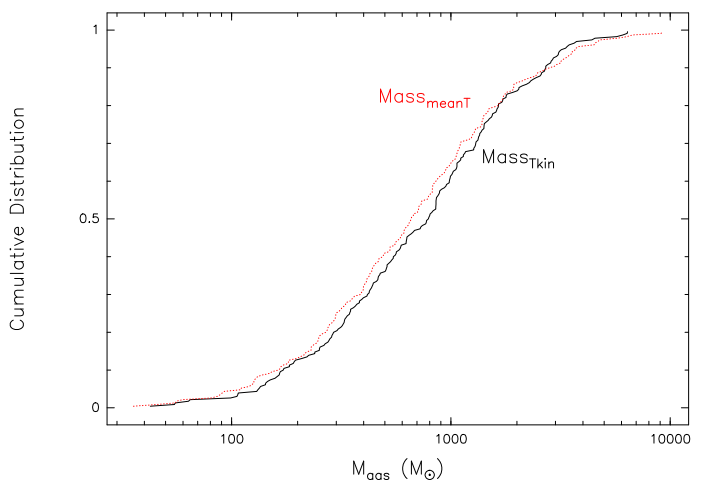
Fig. 11: Cumulative distribution function of the gas mass, which is computed using the observed kinetic temperature of each source shown as solid black line and using the average kinetic temperature of the sample illustrated as dotted red line.
