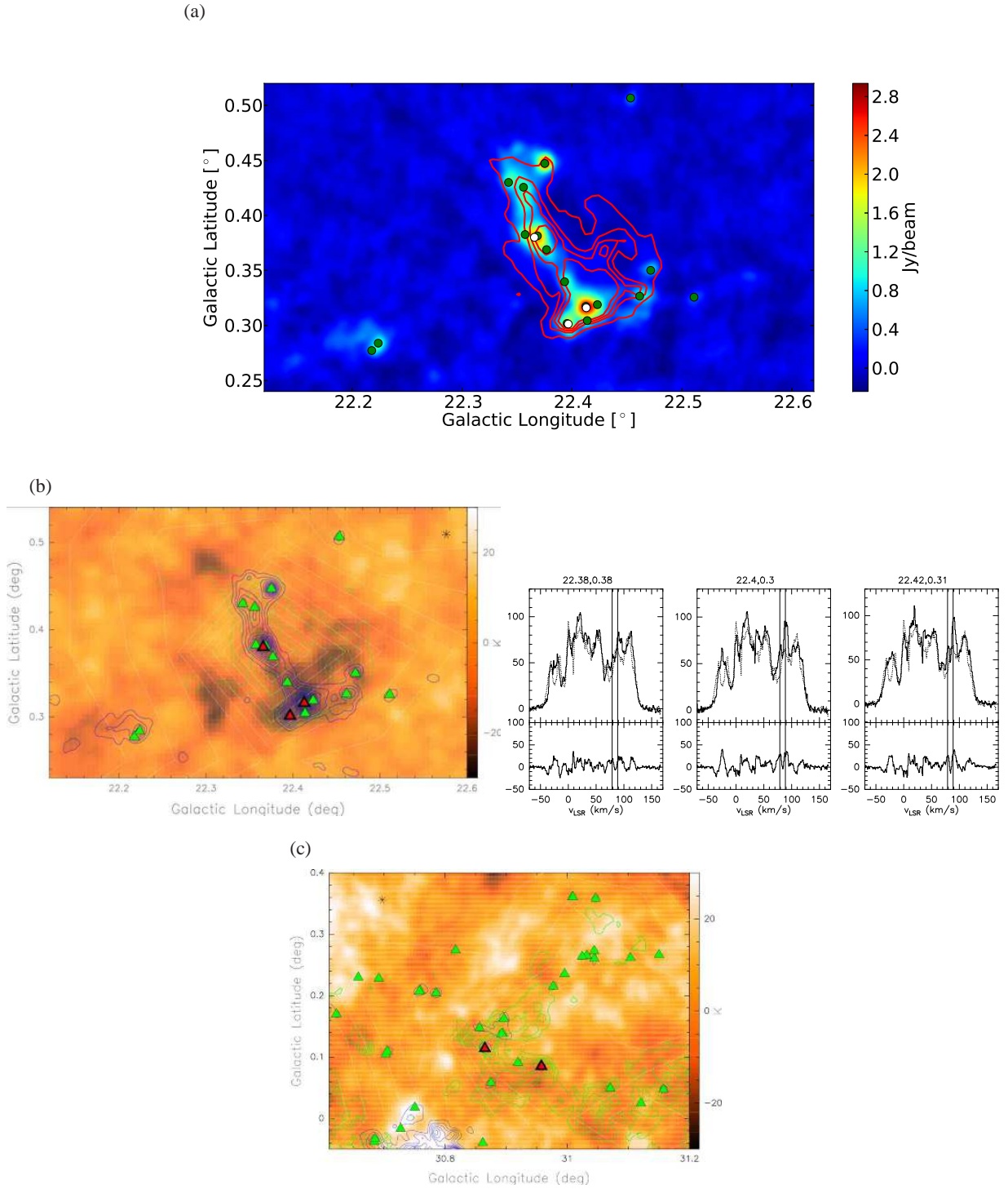
Fig. 2: a) Example of a complex in the first quadrant: The 780\ \mu\text{m} dust continuum is shown in the background probing the small-scale molecular cloud structure. We illustrate ATLASGAL sources with observed velocities of \sim 84\ \text{km s}^{-1} as white dots and ATLASGAL sources without known velocities as green dots. The ^{13}\text{CO} emission at the velocity of the complex is indicated as red contours. b) The panel on the left displays the HI emission map of the region shown in a) : The HI intensity is integrated in the velocity interval around the group velocity and in intervals at smaller and larger velocities. The subtraction of these maps (see Sect. 5.2) reveals HI self-absorption plotted in the background with the 780\ \mu\text{m} dust continuum overlaid as blue contours, the ^{13}\text{CO} (1–0) emission as green contours, and the ^{12}\text{CO} intensity as white contours. We show ATLASGAL sources with measured velocities as red triangles and ATLASGAL sources without velocities as green triangles. We extracted HI lines at the location of observed source and at one offset position, which is indicated by the star on the map. The HI "on-source" spectra are illustrated as solid lines and the "off-source" spectrum as dashed line in the panel on the right. The labels on the top display the galactic coordinates of observed source positions. Vertical lines in the spectra indicate the variation of the source velocity resulting from the velocity dispersion of clouds or streaming motions. The difference of the on-source and off-source spectra is shown below the HI spectra. c) Example of another region, which illustrates HI emission. The HI map in the background is produced and overlaid with the same contours and symbols as described for panel b) .
