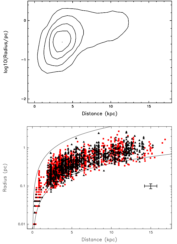
Fig. 10: Dependence of the source radius not deconvolved from the beam on the kinematic distance to the ATLASGAL sample in the first quadrant as black triangles and the clumps in the fourth quadrant as red points is shown as scatter plot in the lower panel. The lower curve indicates radii corresponding to the beam radius of 9'' , the upper curve illustrates radii computed with 1.3'' . The binning of the kinematic distance in the contour plot in the upper panel is 1.5 kpc and that of the logarithm of the radius is 0.5. The contour levels from 10 to 90% are shown in intervals of 20% of the peak source number per bin. The error bar indicates the average distance and radius errors.
