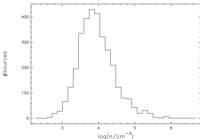
Fig. 14: Histogram of the \text{H}_2 volume density of the ATLASGAL sample. Most sources exhibit a volume density of 7842 \text{ cm}^{-3} .
