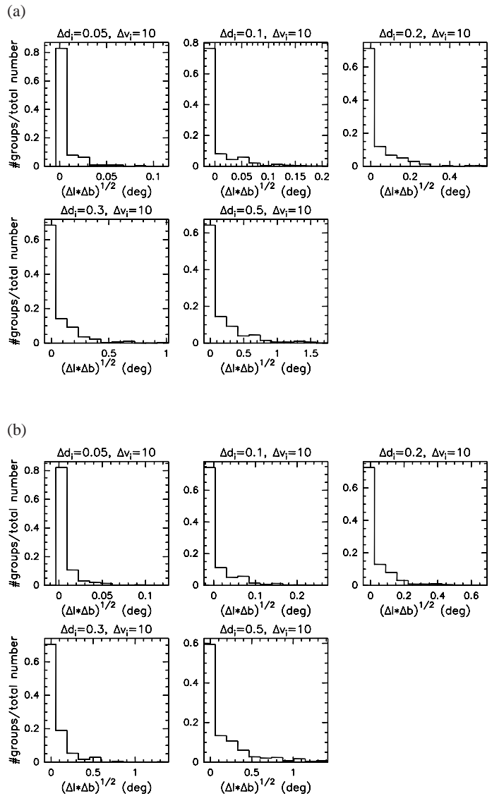
Fig. A.1: Relative number distribution of ATLASGAL groups with the size of a group for different input values of the maximum distance between individual sources within a group, \Delta d_i . This is varied between 0.05^\circ and 0.5^\circ with a fixed interval for velocities of neighbouring sources in a group, \Delta v_i , of 10 \text{ km s}^{-1} for the sample in the first quadrant in panel a) and the groups in the fourth quadrant in panel b).
