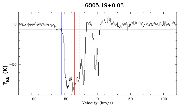
Fig. B.1: HI spectrum toward G305.19+0.03, an HII region in the high mass star forming complex G305 extracted from the SGPS. For explanation of the different lines see Fig. 3. The HI absorption method yields the far distance.
