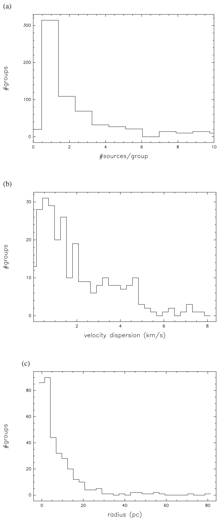
Fig. A.3: Number distribution of ATLASGAL groups with the number of sources per group in a ), the velocity dispersion in b ), and radius in c ).
