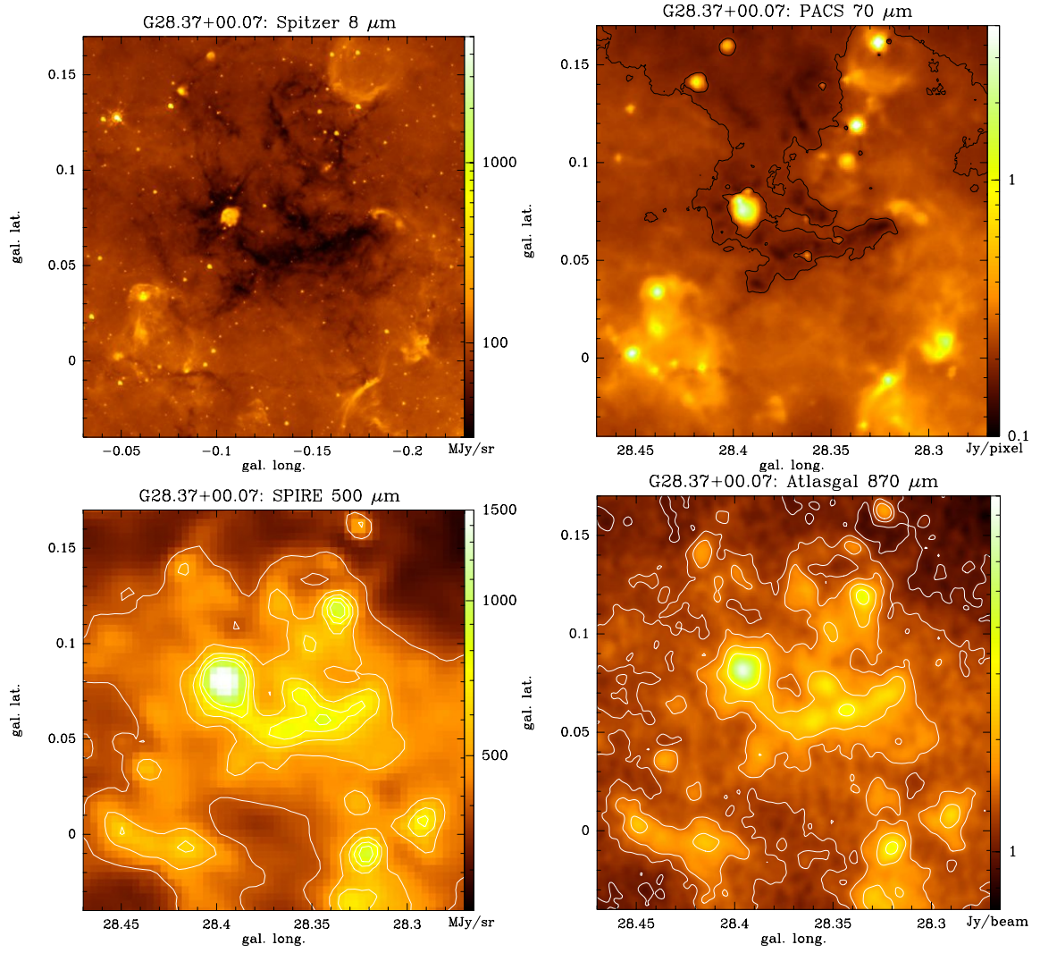
Fig. 1. Top: Spitzer 8 \mu\text{m} ( \sim 2.5'' resolution) and PACS 70 \mu\text{m} maps ( \sim 11'' resolution). The Spitzer/IRAC data were taken from the public available GLIMPSE archive. Bottom: SPIRE 500 \mu\text{m} map ( 36'' resolution) and ATLASGAL 870 \mu\text{m} maps ( 23'' resolution) of G28.37+0.07. The central dark feature in the Spitzer and PACS images is the IRDC, appearing bright at longer wavelengths (SPIRE and ATLASGAL).
