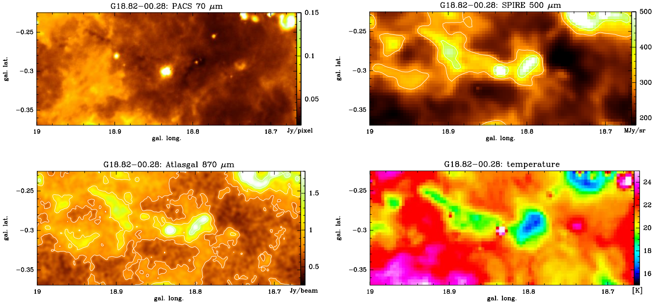
Fig. A.3. PACS 70 \mu\text{m} map, SPIRE 500 \mu\text{m} , and ATLASGAL 870 \mu\text{m} maps of IRDC G18.82-0.28 (Cloud A). The long filamentary structure is well visible as a dark (bright) feature in the 70 \mu\text{m} (500, 870 \mu\text{m} ) maps. Bottom right: temperature map from SED fit 160-500 \mu\text{m} .
