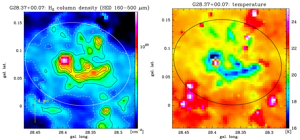
Fig. 2. Left: H 2 -column density map from an SED fit to Herschel fluxes at 160-500 \mu\text{m} . The black contours indicate the levels N_{dust}=4 to 7 \times 10^{22} \text{ cm}^{-2} in steps of 10^{22} \text{ cm}^{-2} , the white-dashed contour outlines the approximate completeness level ( \sim 3 \times 10^{22} \text{ cm}^{-2} ), and the white ellipse is taken from Simon et al. (2006b), defining the IRDC. Right: temperature map of G28.37+0.07.
