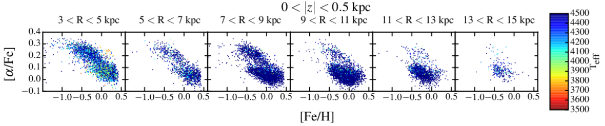
Figure B1. The distribution of stars in the [\alpha/\text{Fe}] vs. [\text{Fe}/\text{H}] plane color coded by T_{\text{eff}} for stars with |z| < 0.5 kpc. There is evidence for temperature trends in the [\alpha/\text{Fe}] abundance in the inner Galaxy ( 3 < R < 5 kpc). This figure is down-sampled and shows only 15% of the datapoints for R > 5 kpc.
