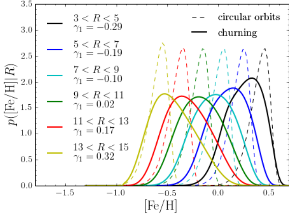
Figure 10. The MDF as a function of R with the inclusion of blurring and churning. The dashed lines show the initial MDF and the solid lines display the MDF including the effects of churning and blurring. The redistribution of guiding radii due to churning is able to significantly change the skewness compared to the initial MDFs and can explain the changes in skewness and its sign observed in the APOGEE sample.
