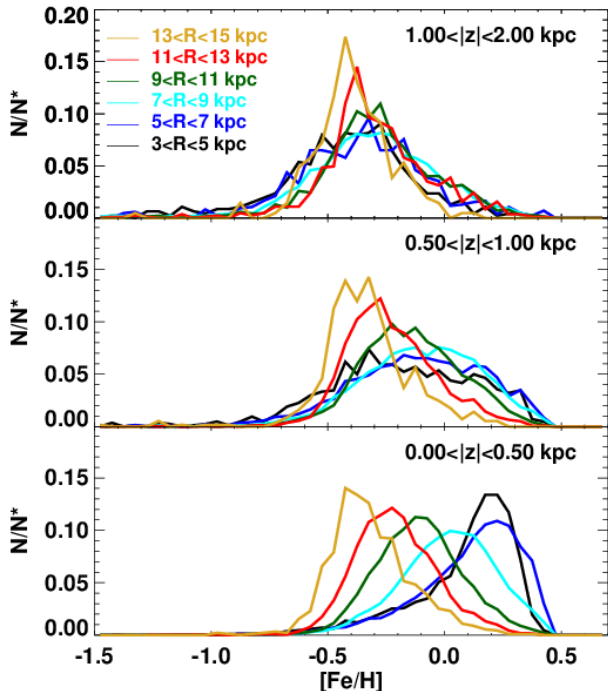
Figure 5. The observed MDF for the entire sample as a function of Galactocentric radius over a range of distances from the plane. The shape and skewness is a function of radius and height. Close to the plane, the inner Galaxy ( 3 < R < 5 kpc) is a negatively skewed distribution and a peak metallicity at \sim 0.25 dex, while the outer disk ( R > 11 kpc) has a positively skewed distribution with peak metallicity of \sim -0.4 dex. For |z| > 1 kpc, the MDF is fairly uniform across all radii.
