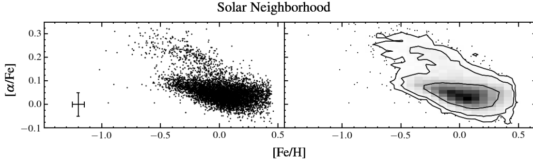
Figure 3. The observed [\alpha/\text{Fe}] vs. [\text{Fe}/\text{H}] distribution for the solar neighborhood ( 7 < R < 9 kpc, 0 < |z| < 0.5 kpc). The left panel is down-sampled and shows only 20% of the observed data points in the solar circle. The right panel shows the entire sample in the solar neighborhood, with contours denoting 1, 2, 3 \sigma of the overall densities. There are two sequences in the distribution of stars in the [\alpha/\text{Fe}] vs. [\text{Fe}/\text{H}] plane, one at solar- [\alpha/\text{Fe}] abundances, and one at high- [\alpha/\text{Fe}] abundances that eventually merges with the solar- [\alpha/\text{Fe}] sequence at [\text{Fe}/\text{H}] \sim 0.2 .
