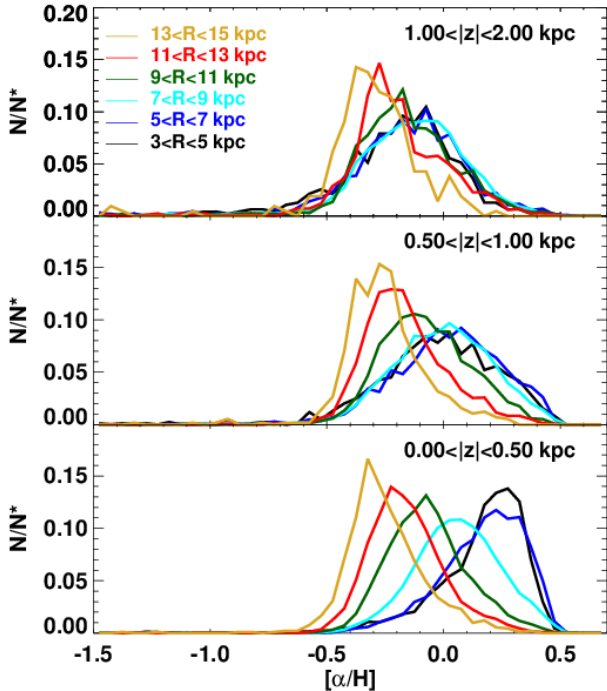
Figure 7. The observed distribution of [\alpha/\text{H}] for the entire sample as a function of Galactocentric radius over a range of distances from the plane. The results are quite similar to that of the MDF, except for stars with |z| > 1 kpc and R < 9 kpc, where the ADF has larger abundances than the MDF at the same locations.
