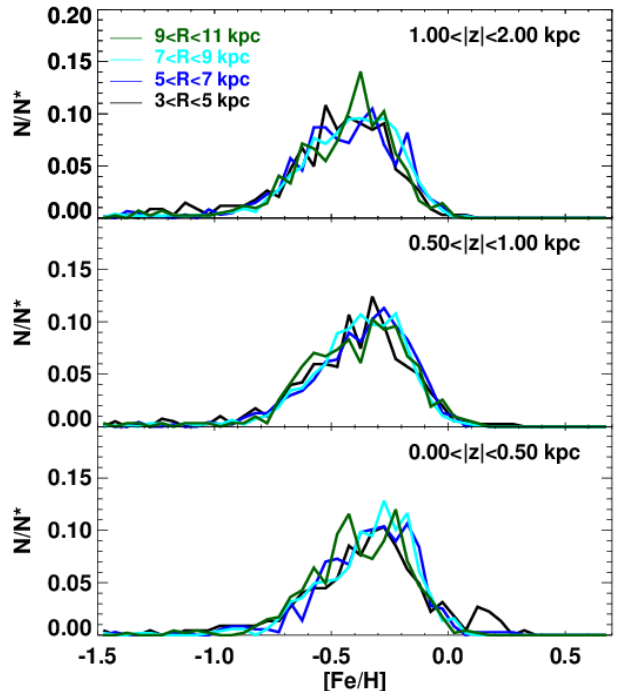
Figure 6. The observed MDF for stars with [\alpha/\text{Fe}] > 0.18 as a function of Galactocentric radius over a range of distances from the plane. There is little variation in the MDF with Galactocentric radius. There is a shallow negative vertical gradient, as stars with |z| > 1 kpc are slightly more metal-poor than stars close to the plane.
