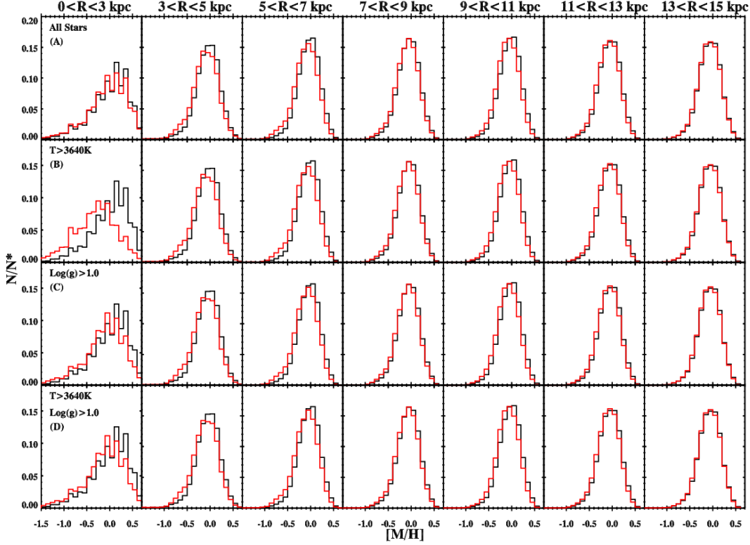
Figure A1. The observed mock MDF of giants (red) compared to the intrinsic MDF of giants (black) as a function of R . (A): Only targeting criteria (field placement, color cuts, magnitude limits) applied to the input simulations. (B): The observed MDF with the temperature restrictions imposed by the ASPCAP grid edge. (C): The observed MDF with a restricted surface gravity range. (D): The observed MDF with both the temperature and surface gravity restrictions. There is little difference between panels (C) and (D), the effects of the temperature grid-edge on the observed MDF has largely been mitigated due to the restriction in surface gravity, leading to a significantly less biased MDF.
