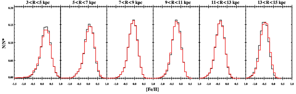
Figure A3. The mock targeted MDF (black) versus the mock observed MDF after applying distance errors to the TRILEGAL simulation (red). The difference between the two is negligible except for the very outer disk ( R > 13 kpc).
