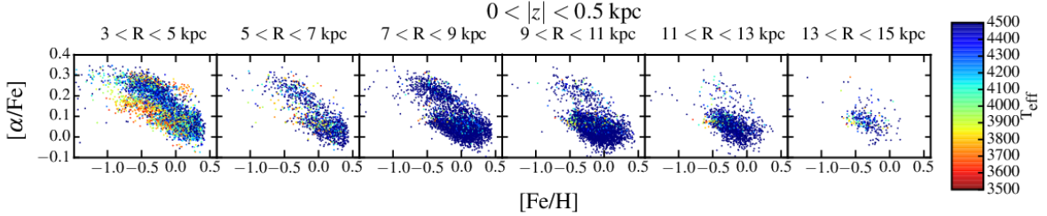
Figure B2. Similar to above, but with the surface gravity restrictions removed. The [\alpha/\text{Fe}] abundance trends with temperature are clear with the inclusion of the lower surface gravity stars. Cooler stars have lower [\alpha/\text{Fe}] abundances by \sim 0.1 dex.
