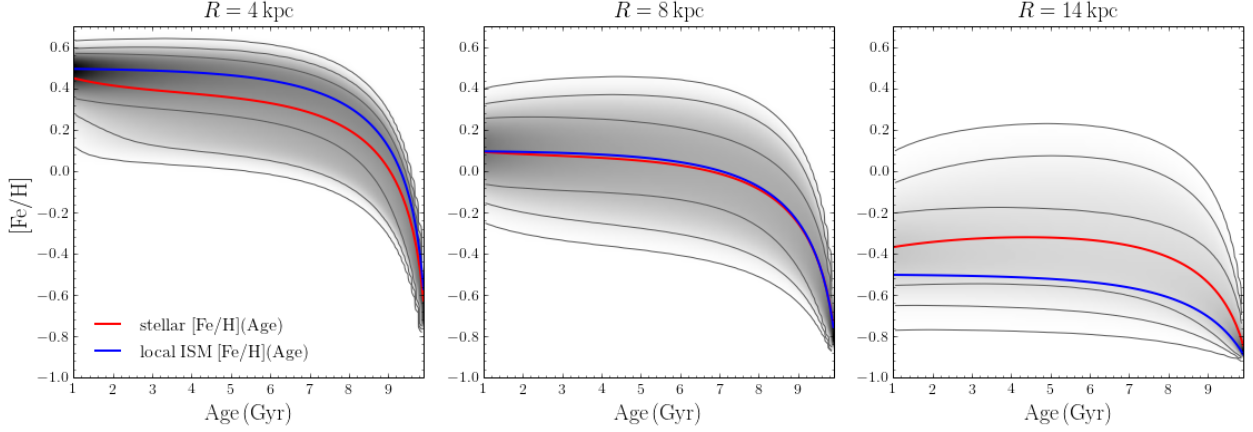
Figure 9. The age–metallicity relation at different radii for our simple model. The blue line shows the metallicity of the ISM as a function of age at different radii, while the solid black lines denote 1, 2, and 3\sigma of the distribution of stars in the age–metallicity plane respectively; the solid red line gives the mean metallicity as a function of age. The solar neighborhood and the outer disk both display a wide range of metallicities for all but the oldest stars.
