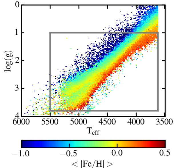
Figure 1. The spectroscopic H-R diagram for the full calibrated APOGEE sample, where the mean metallicity in each \log g , T_{\text{eff}} bin is shown. The gray box denotes the selected sample of 69,919 stars presented in this paper.
