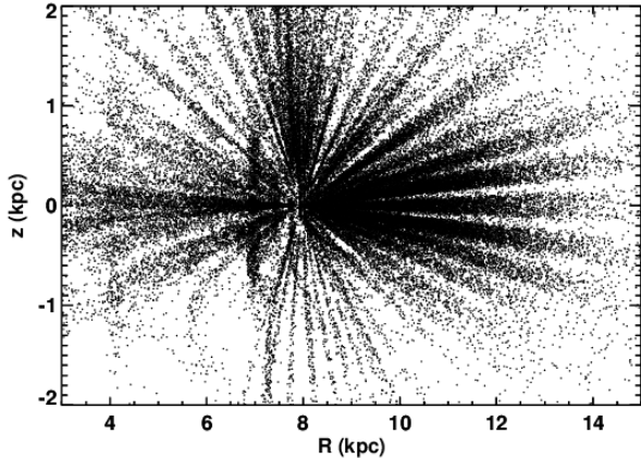
Figure 2. The Galactic R - z distribution for the sample of 69,919 stars used in this analysis. R is the projected planar distance from the Galactic center, while z is the distance from plane of the Galaxy. Each star is plotted at the location implied by the median of its distance modulus PDF.
