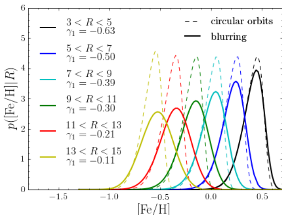
Figure 8. The MDF as a function of R for our simple blurring model. The dashed lines show the initial MDFs (which the stars on circular orbits would have) and the solid lines represent the MDFs including the effect of blurring. The skewness of the blurred MDFs are indicated. The magnitude of the skewness diminishes with radius, but it does not change sign.
