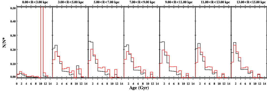
Figure A2. The intrinsic age distribution of giants in the TRILEGAL simulation (black) compared to the mock observed age distribution (red). The sample selection criteria does not induce a large bias in the observed sample, although the targeted sample is slightly older in general than the underlying age distribution of giants in the simulation.
