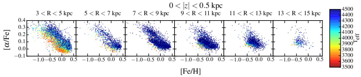
Figure B3. Similar to above, but with the [\alpha/\text{Fe}] measured by averaging the abundances for the individual \alpha elements. We find similar trends as in Figure. B2 above, with the cooler stars having lower- [\alpha/\text{Fe}] abundances than the warmer stars at the same metallicities.
