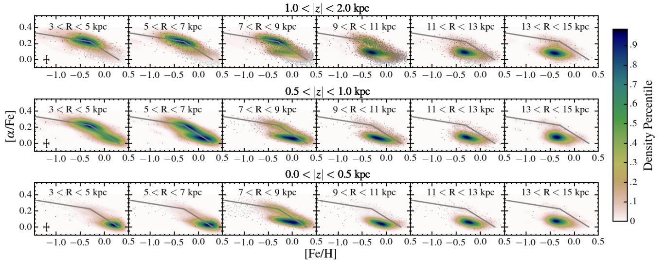
Figure 4. The stellar distribution of stars in the [\alpha/\text{Fe}] vs. [\text{Fe}/\text{H}] plane as a function of R and |z| . Top: The observed [\alpha/\text{Fe}] vs. [\text{Fe}/\text{H}] distribution for stars with 1.0 < |z| < 2.0 kpc. Middle: The observed [\alpha/\text{Fe}] vs. [\text{Fe}/\text{H}] distribution for stars with 0.5 < |z| < 1.0 kpc. Bottom: The observed [\alpha/\text{Fe}] vs. [\text{Fe}/\text{H}] distribution for stars with 0.0 < |z| < 0.5 kpc. The grey line on each panel is the same, showing the similarity of the shape of the high- [\alpha/\text{Fe}] sequence with R . The extended solar- [\alpha/\text{Fe}] sequence observed in the solar neighborhood is not present in the inner disk ( R < 5 kpc), where a single sequence starting at high- [\alpha/\text{Fe}] and low metallicity and ending at solar- [\alpha/\text{Fe}] and high metallicity fits our observations. In the outer disk ( R > 11 kpc), there are very few high- [\alpha/\text{Fe}] stars.
