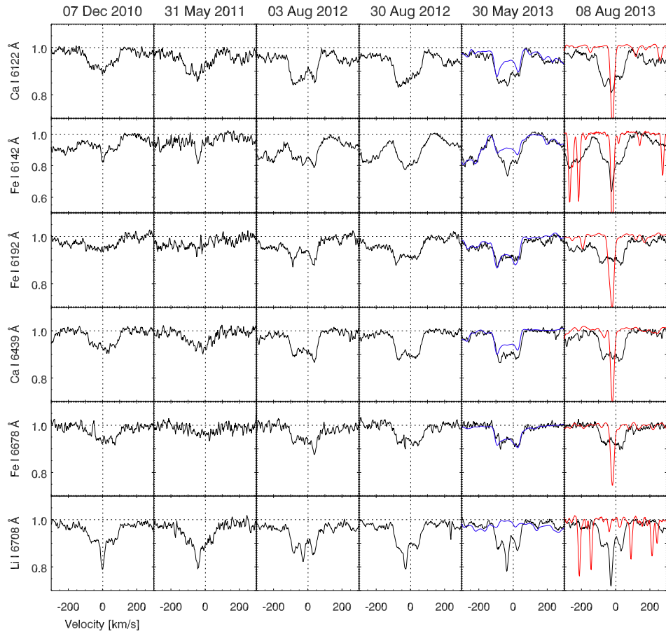
Fig. 2.— Time variation of the double-peaked absorption features in various lines, evidence of disk rotation. Only the HET-HRS spectra are presented because the BOES spectra have much lower signal-to-noise ratio. The dates in the columns are the same as those in Figure 1. The blue and red spectra are also the same as those in Figure 1.
