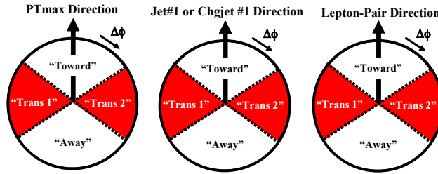
Figure 1: Illustration of the regions of \eta - \phi space that are defined relative to the direction of a “leading object” in the event. The “leading object” can be the highest p_{\text{T}} charged particle ( left ), the highest p_{\text{T}} charged-particle or calorimeter jet ( middle ), or the lepton-pair in Z-boson production ( right ). The relative azimuthal angle \Delta\phi = \phi - \phi_{\text{L}} , where \phi_{\text{L}} is the azimuthal angle of the leading object and \phi is the azimuthal angle of a charged particle. The “toward” region is defined by |\Delta\phi| < 60^\circ and |\eta| < \eta_{\text{cut}} , while the “away” region is |\Delta\phi| > 120^\circ and |\eta| < \eta_{\text{cut}} . The two “transverse” regions -120^\circ < \Delta\phi < -60^\circ , |\eta| < \eta_{\text{cut}} and 60^\circ < \Delta\phi < 120^\circ , |\eta| < \eta_{\text{cut}} are referred to as “transverse 1” and “transverse 2”.
