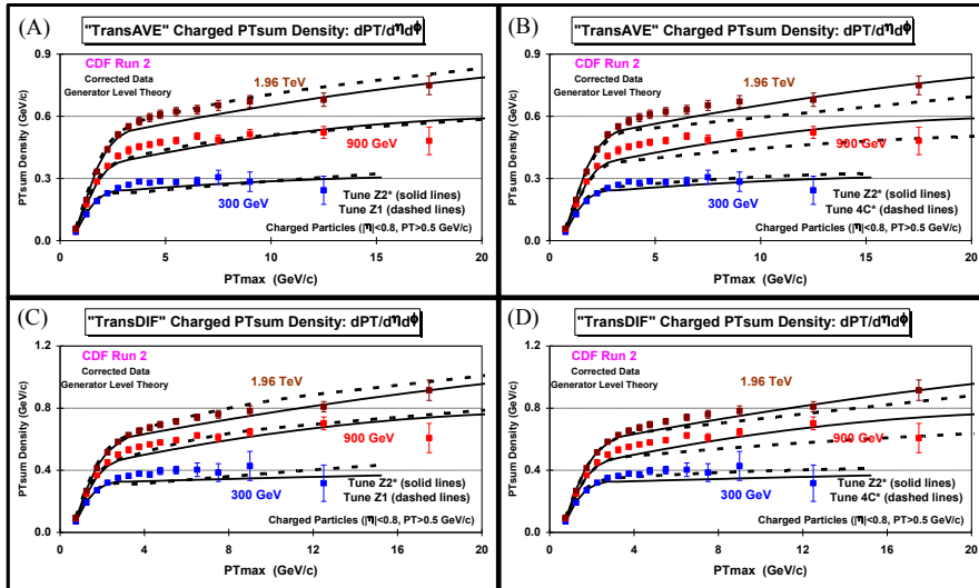
Figure 13. Data at 1.96 TeV, 900 GeV, and 300 GeV on the charged PTsum density ( p_T > 0.5 GeV/c, |\eta| < 0.8 ) in the transAVE (A,B) and transDIF (C,D) regions as defined by the leading charged particle, as a function of the p_T of the leading charged particle, PTmax. The data are corrected to the particle level with errors that include both the statistical error and the systematic uncertainty, and are compared with PYTHIA Tune Z1 and Z2* (A,C) and PYTHIA Tune Z2* and 4C* (B,D).
