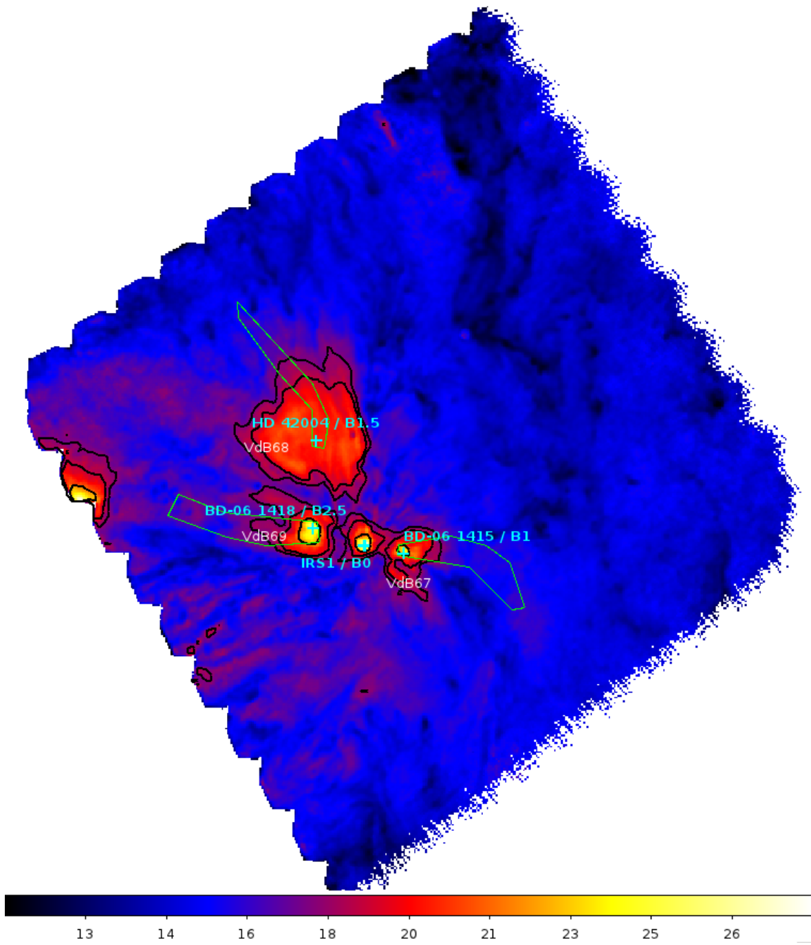
Fig. 13: Hot regions overall contours of profile extraction on temp. map. Spectral type are taken from Racine (1968).
