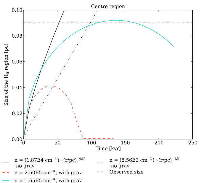
Fig. 10: Numerical simulations for the central UC H II region expansion. In black: without gravity and in an envelope of decreasing density, which is extrapolated from the observed one up to a constant density within r_c = 0.005 pc. In dotted black: without gravity in an envelope of decreasing density with a gradient typical of infall, \rho \propto r^{-1.5} . In cyan: with gravity and in an envelope with a constant density of 1.65 \times 10^5 \text{ cm}^{-3} , just allowing the observed size to be reached (black dashed line). In dashed red: with gravity and in an envelope with a constant density of 2.5 \times 10^5 \text{ cm}^{-3} , collapses again before reaching the observed size.
