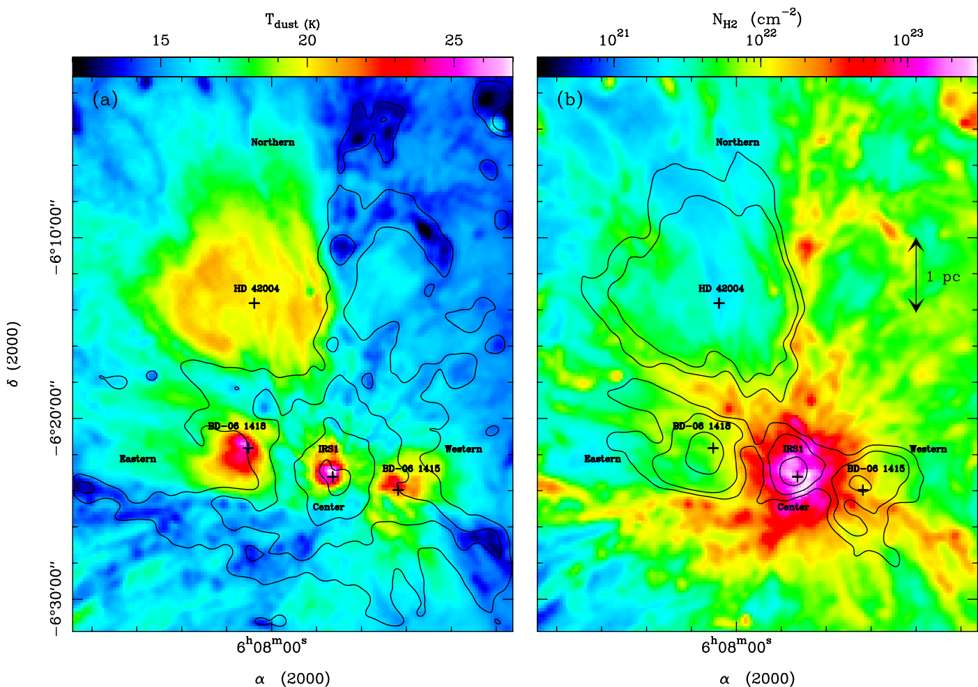
Fig. 2: Dust temperature (colours in a and contours in b ) and column density (colours in b and contours in a ) maps of the central part of the Mon R2 molecular cloud complex, covering the central, western, eastern, and northern H II regions with 36'' resolution. The heating sources of H II regions are indicated by a cross and with their name taken from Racine (1968) and Downes et al. (1975). Smoothed temperature and column density contours are 17.5, 18.5, and 21.5 K and 7 \times 10^{21} , 1.5 \times 10^{22} , 5 \times 10^{22} , and 1.8 \times 10^{23} \text{ cm}^{-2} .
