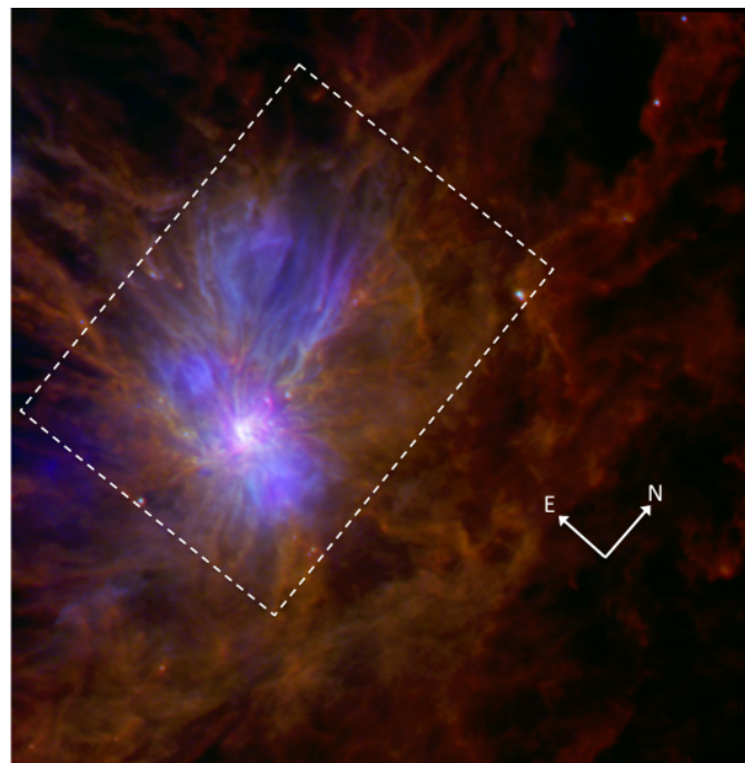
Fig. 1: Three-colour Herschel image of the Mon R2 molecular complex using 70 \mu\text{m} (blue), 160 \mu\text{m} (green), and 250 \mu\text{m} (red) maps. The shortest wavelength (blue) reveals the hot dust associated with H II regions and protostars. The longest wavelength (red) shows the cold, dense cloud structures, displaying a filament network. The dashed rectangle locates the four H II region area shown in Fig. 2
