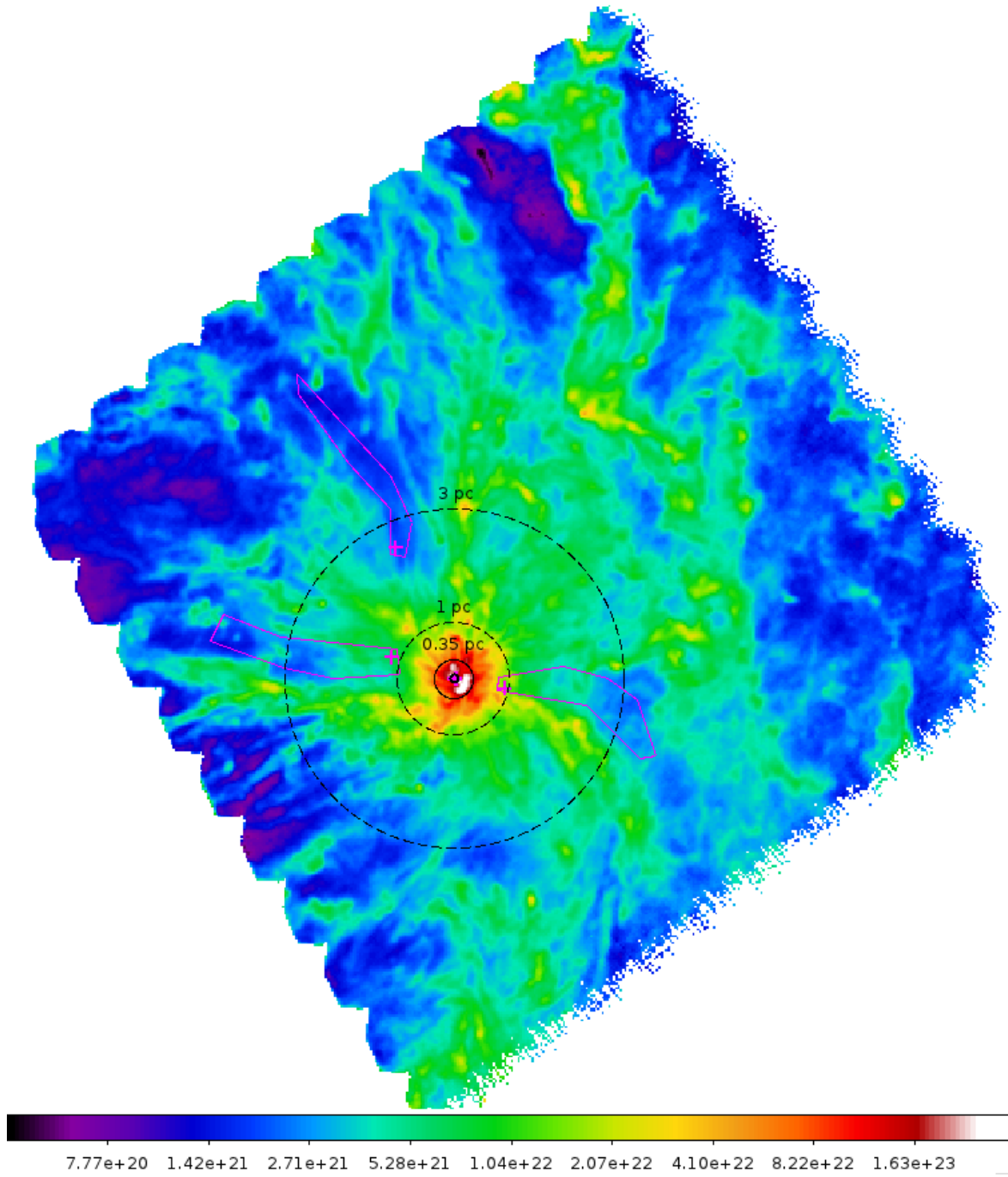
Fig. 12: Column density map showing the azimuthal selection of areas used to characterise the density profiles of the eastern, western, and northern H II region envelopes. The H II region bubble, the inner, and the outer envelopes of the central UCH II region are outlined with dashed circles, whose sizes are given in Tables 1-3.
