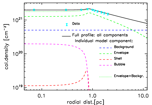
Fig. 8: Column density profile for northern H II region and its four components coded with the same colours as in Fig. 7. The dotted green line corresponding to the sum of the envelope and background contributions matches well with observed data.
