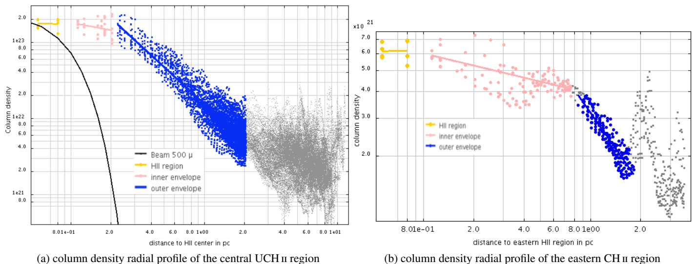
Fig. 6: H II region bubble (yellow line and points) surrounded by a neutral gas envelope splitting into slowly and sharply decreasing N_{H_2} parts (pink and blue lines and points). The background is defined by the lower limit of the clouds of grey points. The resolution corresponding to the Herschel beam at 500\mu\text{m} is illustrated by the black curve in a)
