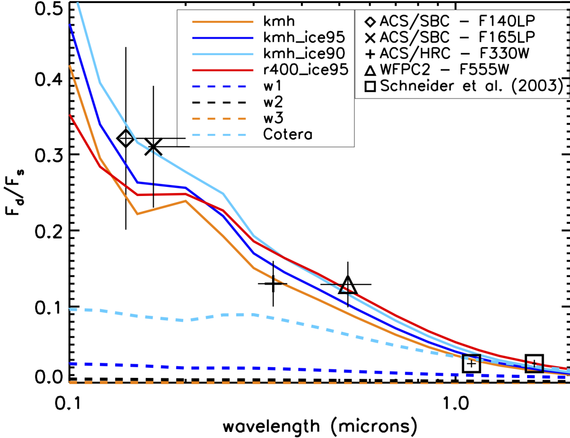
Fig. 7.— The disk scattering fraction at the disk surface F_{disk}/F_{star} as a function of wavelength has been measured and compared with grain opacity models that have varying grain size distributions. The w1, w2, w3, and Cotera models are model 1, 2, 3, and Cotera from Wood et al. (2002b) respectively, and they have size distributions dominated by large (micron-sized) grains or larger and result in gray scattering (flat curve). The r400_ice95 model is a standard one offered in the 2014 version of HOCHUNK3D (Whitney et al. 2013), adopted from Whittet et al. (2001) and modelling total-to-selective extinction of R_V = 4 , corresponding to dense regions of star-forming clouds with optical depth \tau_{3.0} for the 3 \mu\text{m} ice absorption feature. The r400 model and the kmh models have size distributions similar to that of the ISM, with variations in composition, and their scattering efficiency increases rapidly at shorter wavelengths. See § 3.3 for additional details.
