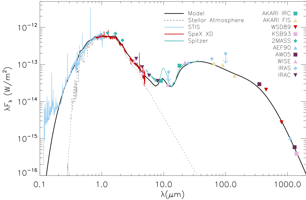
Fig. 8.— The SED of GM Aur using data discussed in § 2.4, and best-fit MCRT model ( solid black line ; see § 3.5). The X-ray flux is 6.82 \times 10^{-16} \text{ W m}^{-2} at \lambda \approx 0.0021 \mu\text{m} (Güdel et al. 2010), and would be consistent with an extrapolation of the UV flux; we do not plot it as it would crowd the other data points into one quadrant of the panel. Paper references are: WSD89 = Weintraub et al. (1989); KSB93 = Koerner et al. (1993); AEF90 = Adams et al. (1990); AW05 = Andrews & Williams (2005). The SPEX and STIS data are from 2011.
