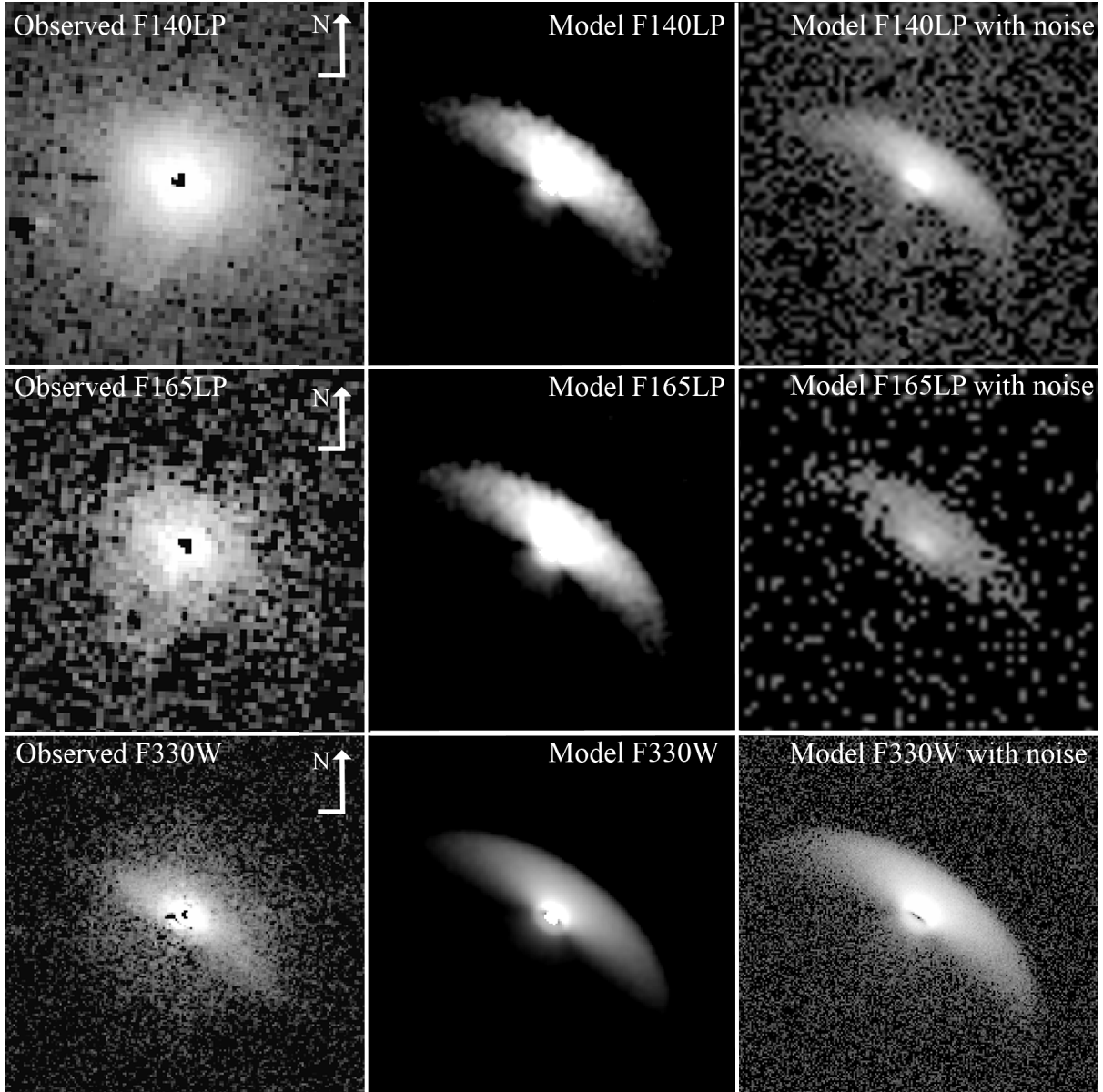
Fig. 10.— Comparison of PSF-subtracted ACS images for GM Aur (left panels) and Whitney code models rotated and scaled to match the images (right panels) for F140LP, F165LP and F330W (top to bottom). Field sizes are 600 AU for the models, and 4''0 for the images (600 AU at 148 pc). North is up and east to the left in all panels. The models and the images generated from them are consistent with the GM Aur SED (see text for details), with the possible exception of accounting for all of the UV excess (involving F140LP and F165LP). The emission to the SE of the disk in those two filters is apparent in the data, but not in the models.
