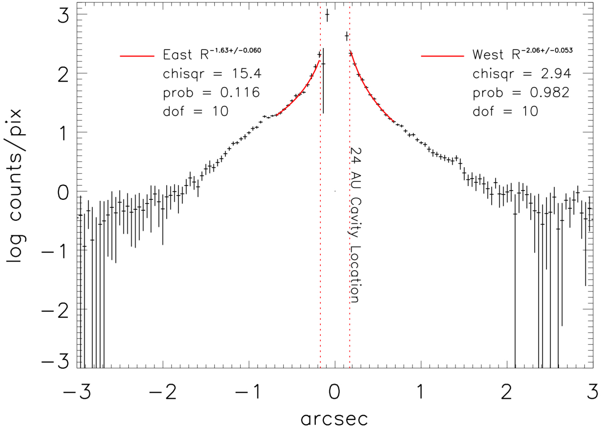
Fig. 5.— The radial surface brightness profile (in \log \text{ counts pixel}^{-1} ) as measured from north-east (left side) to south-west (right side) in the WFPC2 F555W data along the disk major axis \text{PA} = 58.8^\circ \pm 3^\circ . The resulting counts/pixel (surface brightness) vs. radius relation from 0''.15 to 0''.70 was fitted to a line in log-log space with the IDL linfit routine, to determine the power law index \gamma for surface brightness \Sigma \propto r^{-\gamma} (Table 4). The sub-mm cavity wall falls just within the IWA for the F555W profile. There is only one PSF star available, so we cannot show any uncertainty due to PSF template variations.
