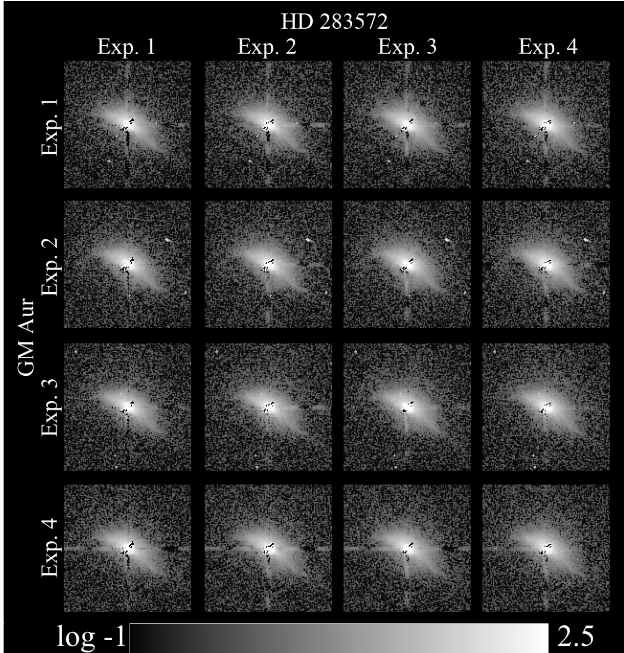
Fig. 1.— The four exposures of GM Aur in the F555W filter subtracted from each of the four exposures of HD 283572. We attribute the variation between exposures to environmental stresses on the spacecraft while in orbit. Images have been rotated to show N up and E to the left. The combination of GM Aur exposure 3 and HD 283572 exposure 4 were used for illustration in Fig. 4.
