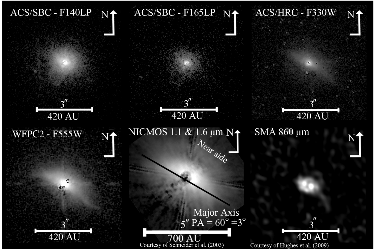
Fig. 4.— Top Row: PSF-subtracted HST imagery observed in the UV with the F140LP (left), F165LP (center), and F330W (right) filters. Bottom Row: PSF subtracted HST imagery observed in the optical with the F555W (left, from a single exposure pair, Fig. 1), the F110W & F160W combined image from Schneider et al. (center, 2003), and 860\ \mu\text{m} from the Submillimeter Array (right, Hughes et al. 2009). All panels show a 6'' \times 6'' FOV and are oriented with north up and east to the left. Hughes et al. (2009) noted an inner cavity of size \sim 20 AU in the 860\ \mu\text{m} data.
