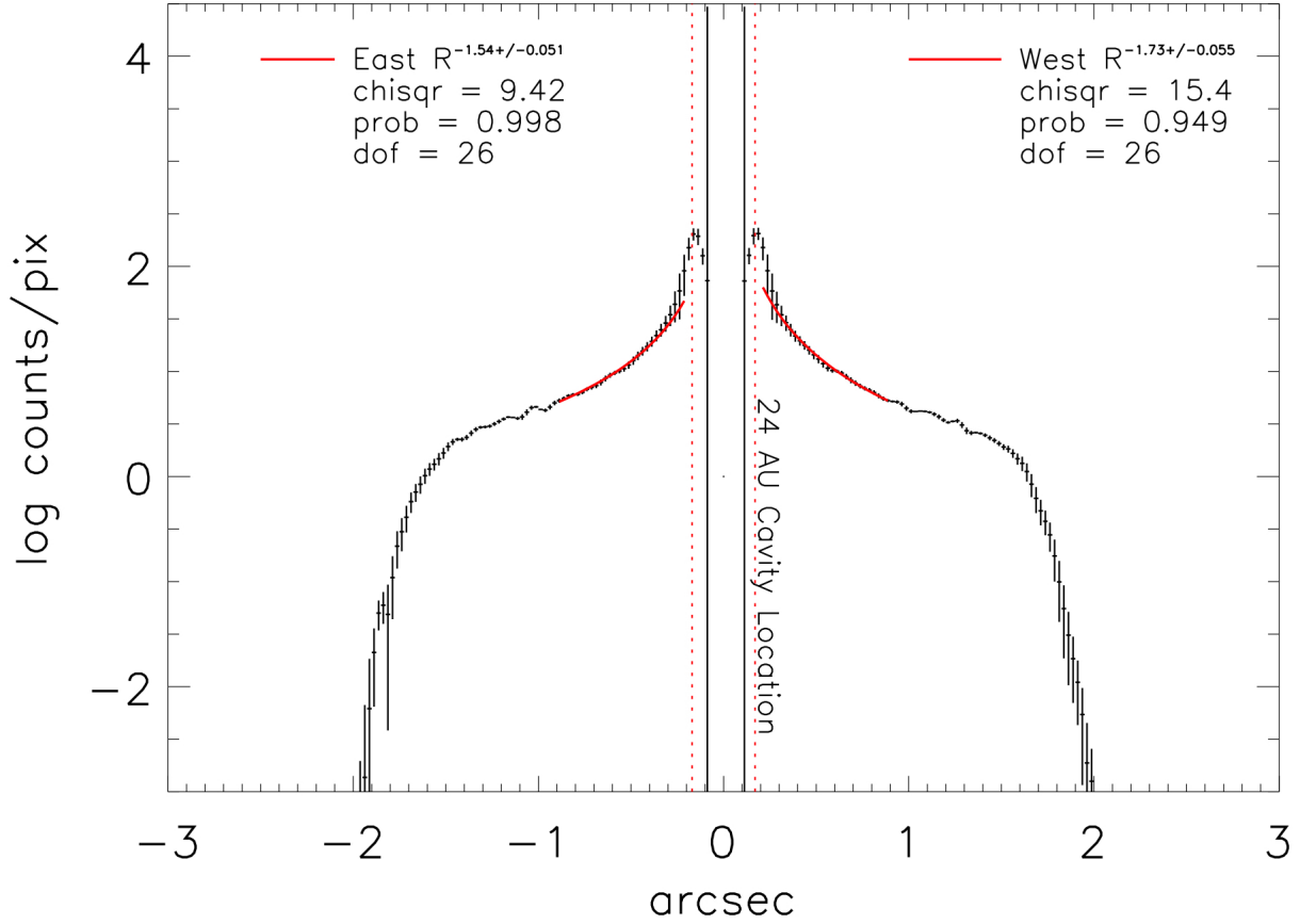
Fig. 11.— The same radial brightness profile calculation as in Fig. 6 on the model F330W image. The 24 AU cavity seen in the sub-millimeter (Hughes et al. 2009), which was not detected in the F330W data, is detected in our model image data. Consequently, the best fit to the model image required a starting point exterior to the cavity location; the fit from 0''.2 to 0''.9 is shown here.
