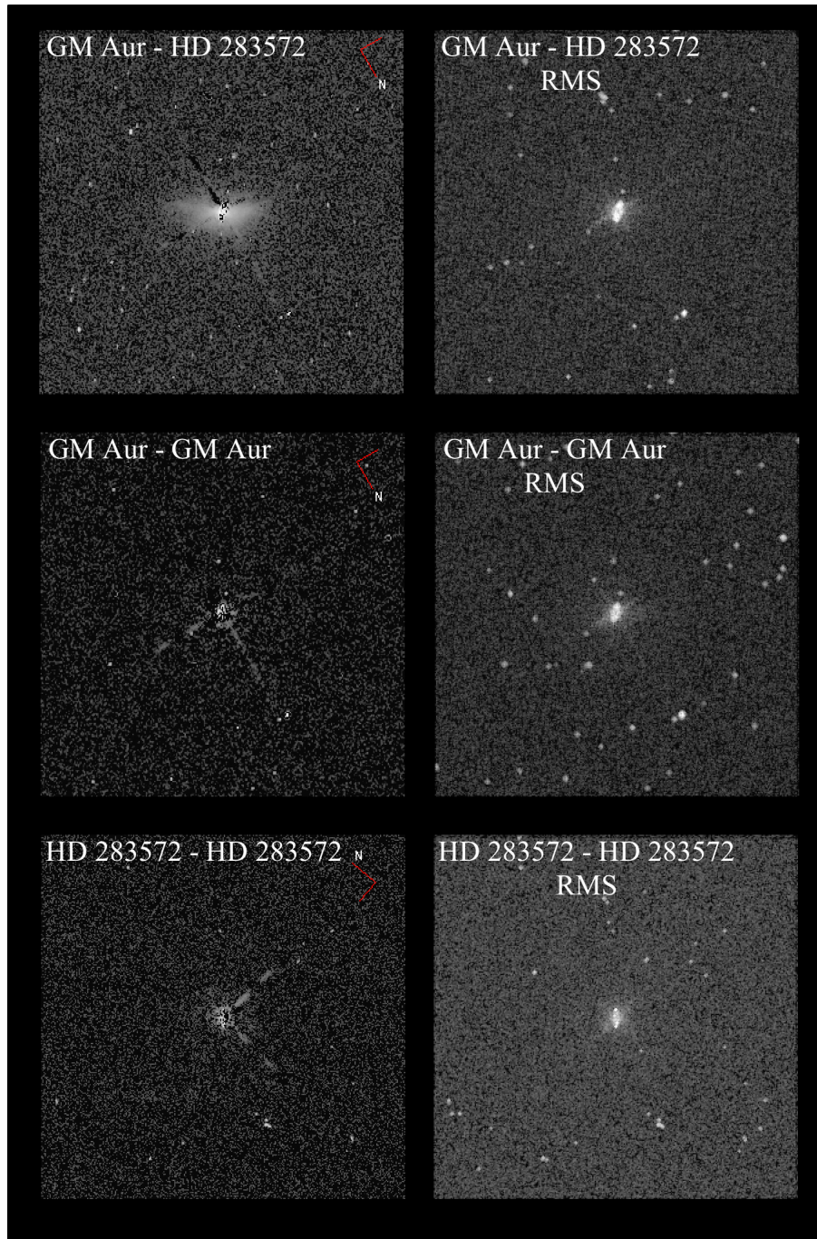
Fig. 2.— To determine the significance of variations between individual exposures we compared and RMS image of the PSF-subtracted data for GM Aur - HD 283572 with subtractions of GM Aur from itself and HD 283572 from itself. Unsurprisingly, the pixel to pixel variations are smallest for the self-subtracted images. See the text for values.
