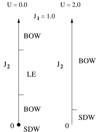
FIG. 13: A sketch of the ground-state phase diagram of the one-dimensional t - U - J_1 - J_2 model at zero and finite U obtained from analysis of the DMRG calculations.
