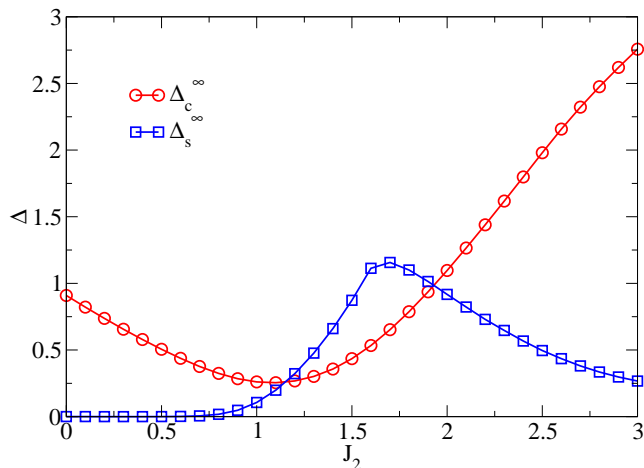
FIG. 11: (Color online) The L = \infty extrapolated spin gap and charge gap as functions of J_2 for U = 2 , J_1 = 1 .
