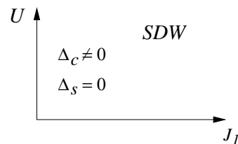
FIG. 3: Field-theory prediction for the half-filled t - U - J_1 model. For all J_1 > 0 , the ground state is a spin-density-wave (SDW) phase with a finite charge gap, zero spin gap and critical spin correlations.
