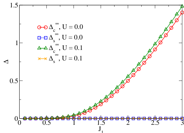
FIG. 6: (Color online) Extrapolated spin and charge gaps for the t - U - J_1 model at U = 0 and 0.1 as functions of J_1 .
