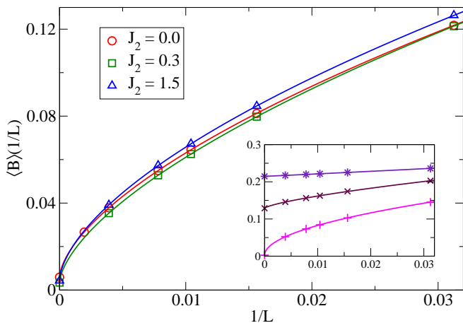
FIG. 8: (Color online) Finite-size scaling analysis for \langle B \rangle(L) for different J_2 when U = 0 and J_1 = 1 . The inset shows the finite-size scaling analysis for J_2 = 2.0, 2.5 , and 3.0 , from bottom to top.
