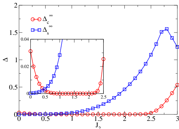
FIG. 9: (Color online) Extrapolated spin gap and charge gap as functions of J_2 for U = 0 , J_1 = 1 . The inset displays the same data for J_2 \leq 2.5 on an enlarged scale.
