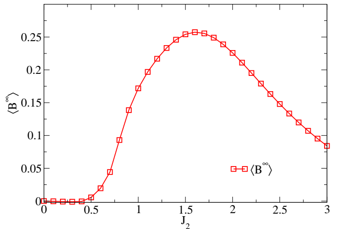
FIG. 12: (Color online) The L = \infty extrapolated \langle B \rangle as a function of J_2 for U = 2 , J_1 = 1 .
