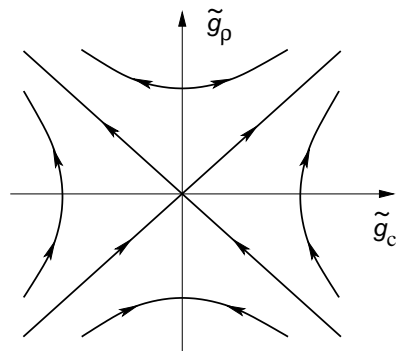
FIG. 1: Scaling curves for the charge-coupling parameters \tilde{g}_c and \tilde{g}_\rho in the presence of a spin gap.
