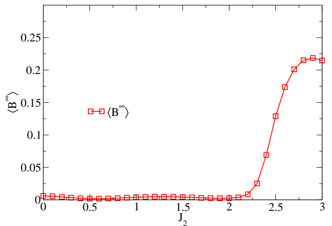
FIG. 10: (Color online) The L = \infty extrapolated bond order parameter \langle B^\infty \rangle as a function of J_2 for U = 0 and J_1 = 1 .
