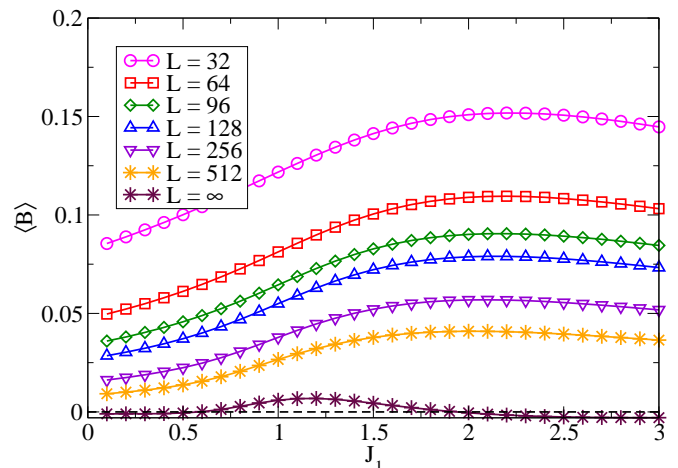
FIG. 7: (Color online) Bond-order parameter \langle B \rangle(L) for L = 32, 64, 96, 128, 256, 512 and extrapolated bond order parameter \langle B^\infty \rangle as a function of J_1 for the t - U - J_1 model at U = 0 .
