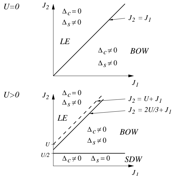
FIG. 2: Field-theory prediction for the half-filled t - U - J_1 - J_2 model. The solid lines give the phase boundaries between the fully gapped regime (bond-order wave, BOW) and the semi-gapped regimes (spin-density wave, SDW; Luther-Emery, LE). The dashed line shows the border between dominantly charge-density-wave and bond-order-wave correlations in the Luther-Emery phase.
