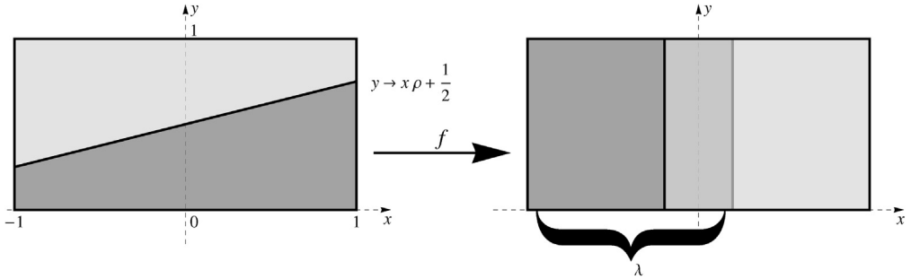
Fig. 10.1. The map f acting on the rectangle [-1, 1] \times [0, 1] .
