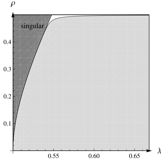
Fig. 10.2. The singularity and absolute continuity region of the measure \mu_{\lambda,\rho} .
