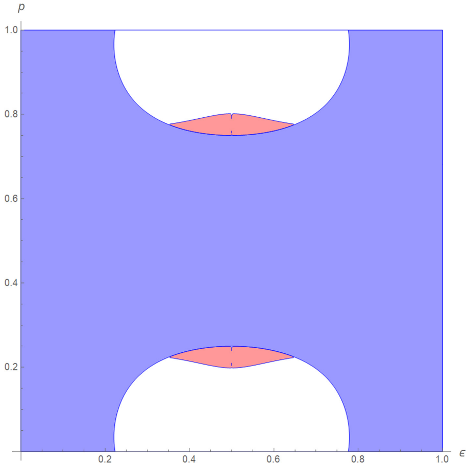
Fig. 10.3. The singularity (blue) and transversality region with \frac{h_{\mu_{\epsilon,p}}}{\chi_{\mu_{\epsilon,p}}} > 1 (red) of the measure \nu_{\epsilon,p} , [2, Figure 1].
