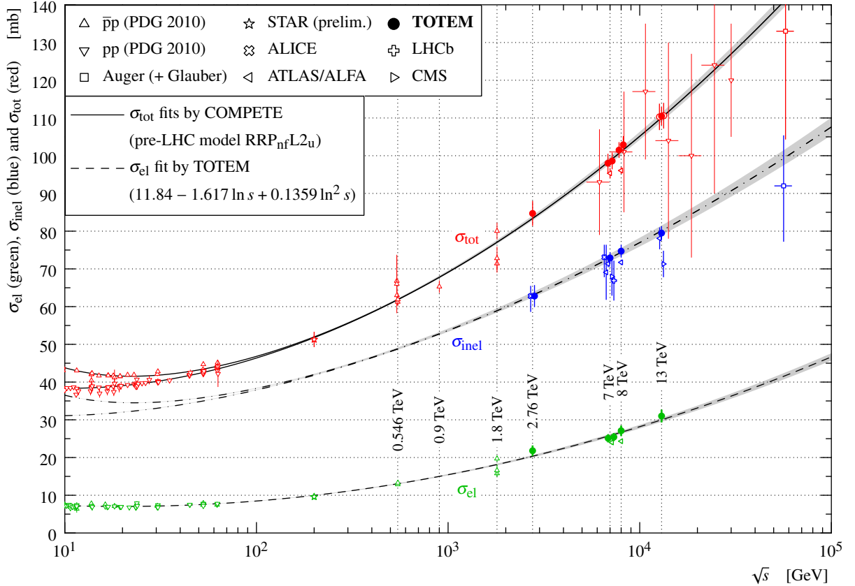
Fig. 18: Total (red), inelastic (blue) and elastic (green) cross-section as a function of energy, \sqrt{s} . The data are taken from Ref. [6] (and references therein) and Table 6. At \sqrt{s} = 13 TeV, three total cross-section points are shown: left hollow corresponds to approach 3, right hollow to Ref. [6] and central filled to the average in Eq. (21).
